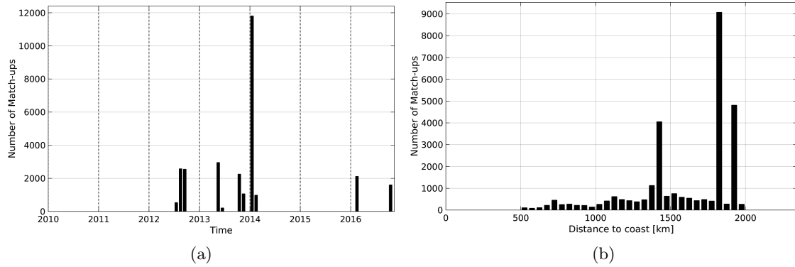
Figure 1: Number of match-ups between TSG-GOSUD-Research-vessel and SMOS-L3-CATDS-CPDC-V3-10DAYS-25KM SSS as a function of time (a) and as function of the distance to coast (b) over the SPURS 1 Pi-MEP region and for the full satellite product period.
