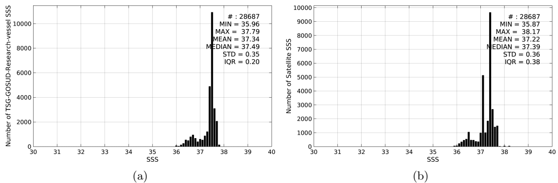
Figure 2: Histograms of SSS from TSG-GOSUD-Research-vessel (a) and SMOS-L3-CATDS-CPDC-V3-10DAYS-25KM (b) considering all match-up pairs per bins of 0.1 over the SPURS 1 Pi-MEP region and for the full satellite product period.
