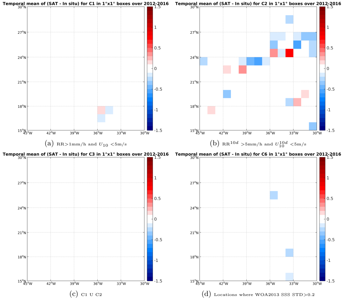
Figure 12: Temporal mean gridded over spatial boxes of size 1°x1° of \Delta SSS (SMOS-L3-CATDS-CPDC-V3-10DAYS-25KM - TSG-GOSUD-Research-vessel) for 4 different subdatasets corresponding to: RR > 1mm/h and U_{10} < 5 m/s (a), RR^{10d} > 5 mm/h and U_{10}^{10d} < 5 m/s (b), C1 U C2 (c), Locations where WOA2013 SSS STD > 0.2 (d).
