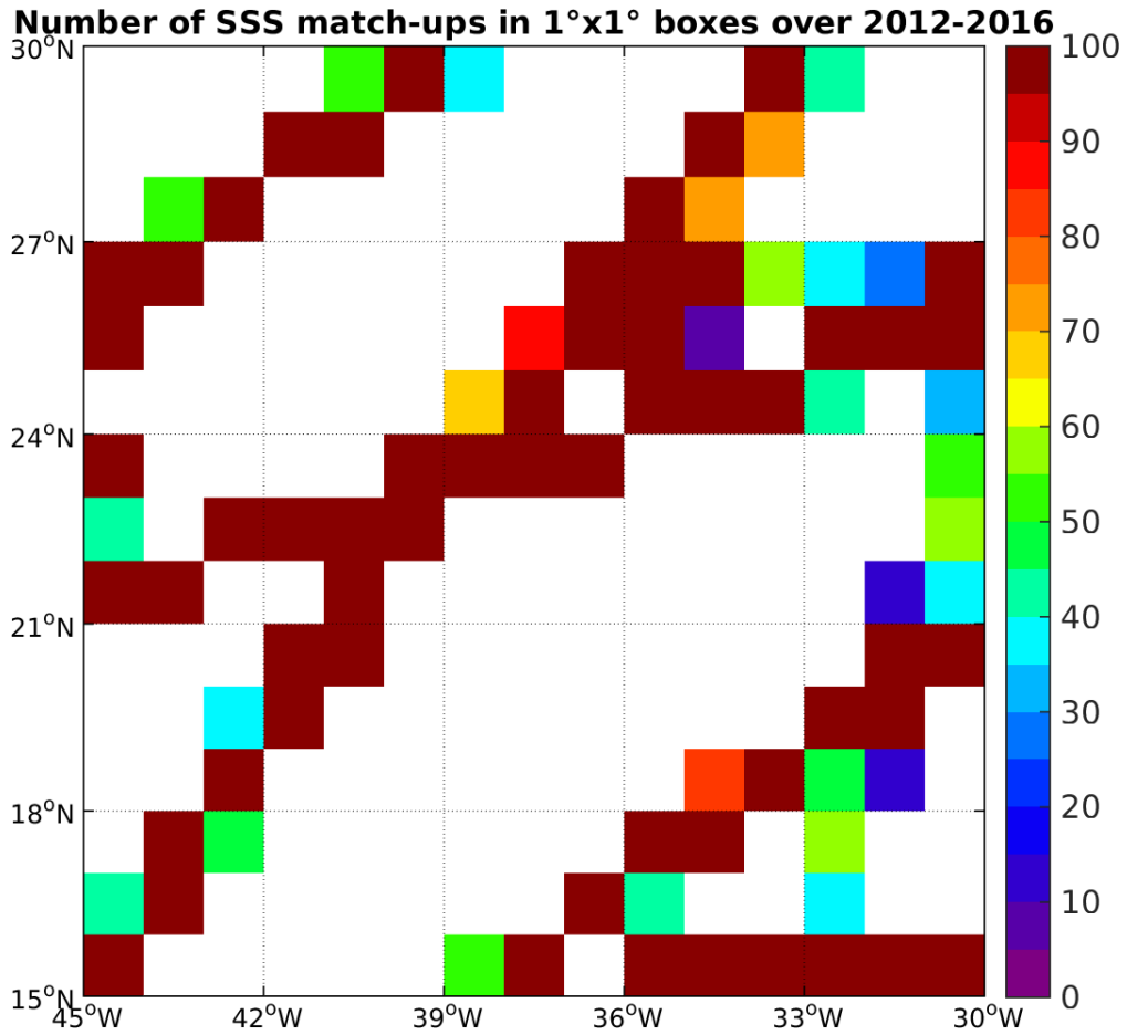
Figure 4: Number of SSS match-ups between TSG-GOSUD-Research-vessel SSS and the SMOS-L3-CATDS-CPDC-V3-10DAYS-25KM SSS product for the SPURS 1 Pi-MEP region over 1°x1° boxes and for the full satellite product period.
