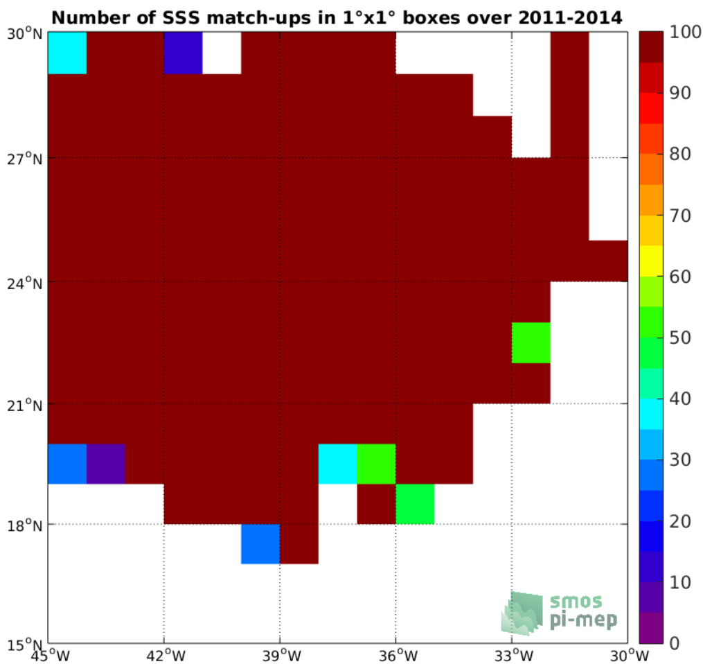
Figure 3: Number of SSS match-ups between Surface drifters SSS and the SMOS-L3-CATDS-CPDC-V3-10DAYS-25KM SSS product for the SPURS 1 Pi-MEP region over 1°x1° boxes and for the full satellite product period.
