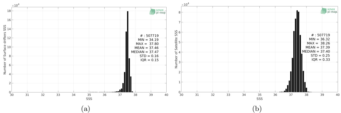
Figure 2: Histograms of SSS from Surface drifters (a) and SMOS-L3-CATDS-CPDC-V3-10DAYS-25KM (b) considering all match-up pairs per bins of 0.1 over the SPURS 1 Pi-MEP region and for the full satellite product period.
