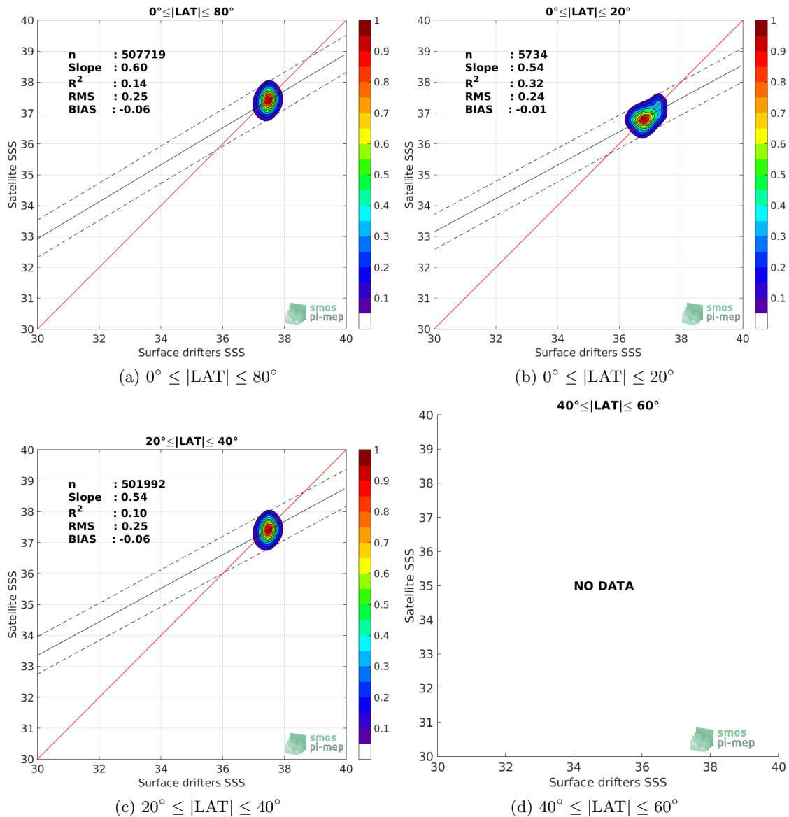
Figure 8: Contour maps of the concentration of SMOS-L3-CATDS-CPDC-V3-10DAYS-25KM SSS (y-axis) versus Surface drifters SSS (x-axis) at match-up pairs for different latitude bands. For each plot, the red line shows x=y . The black thin and dashed lines indicate a linear fit through the data cloud and the \pm 95\% confidence levels, respectively. The number match-up pairs n , the slope and R^2 coefficient of the linear fit, the root mean square (RMS) and the mean bias between satellite and in situ data are indicated for each latitude band in each plots.
