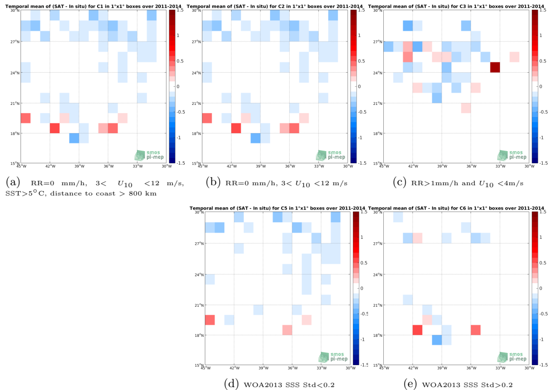
Figure 11: Temporal mean gridded over spatial boxes of size 1^\circ \times 1^\circ of \Delta SSS (SMOS-L3-CATDS-CPDC-V3-10DAYS-25KM - Surface drifters) for 5 different subdatasets corresponding to: RR=0 mm/h, 3 < U_{10} < 12 m/s, SST > 5^\circ\text{C} , distance to coast > 800 km (a), RR=0 mm/h, 3 < U_{10} < 12 m/s (b), RR > 1 mm/h and U_{10} < 4 m/s (c), WOA2013 SSS Std < 0.2 (d), WOA2013 SSS Std > 0.2 (e).
