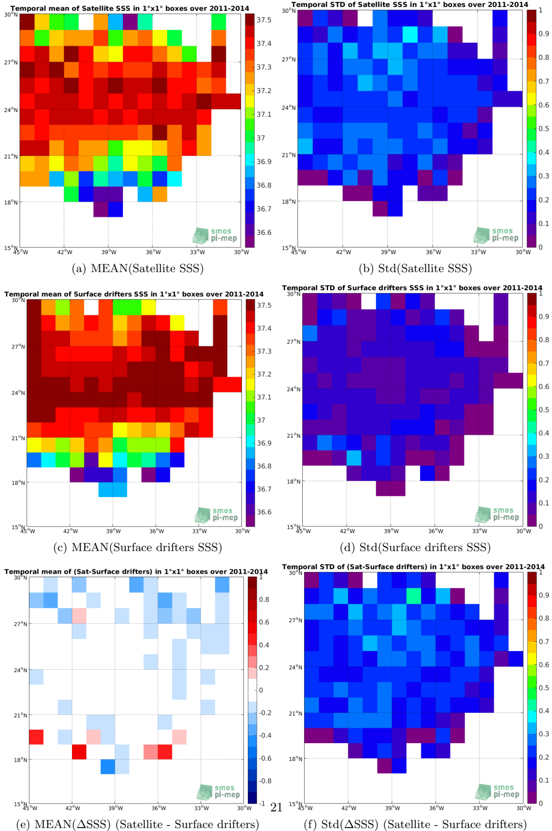
Figure 5: Temporal mean (left) and Std (right) of SSS from SMOS-L3-CATDS-CPDC-V3-10DAYS-25KM (top), Surface drifters (middle), and of \Delta SSS (Satellite - Surface drifters). Only match-up pairs are used to generate these maps.
