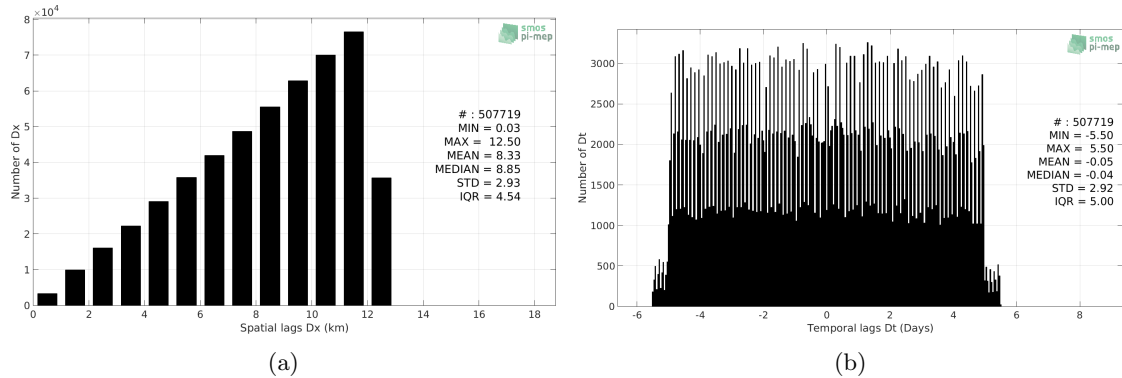
Figure 4: Histograms of the spatial (a) and temporal (b) lags between the time of the Surface drifters measurements and the date of the corresponding SMOS-L3-CATDS-CPDC-V3-10DAYS-25KM SSS product.
