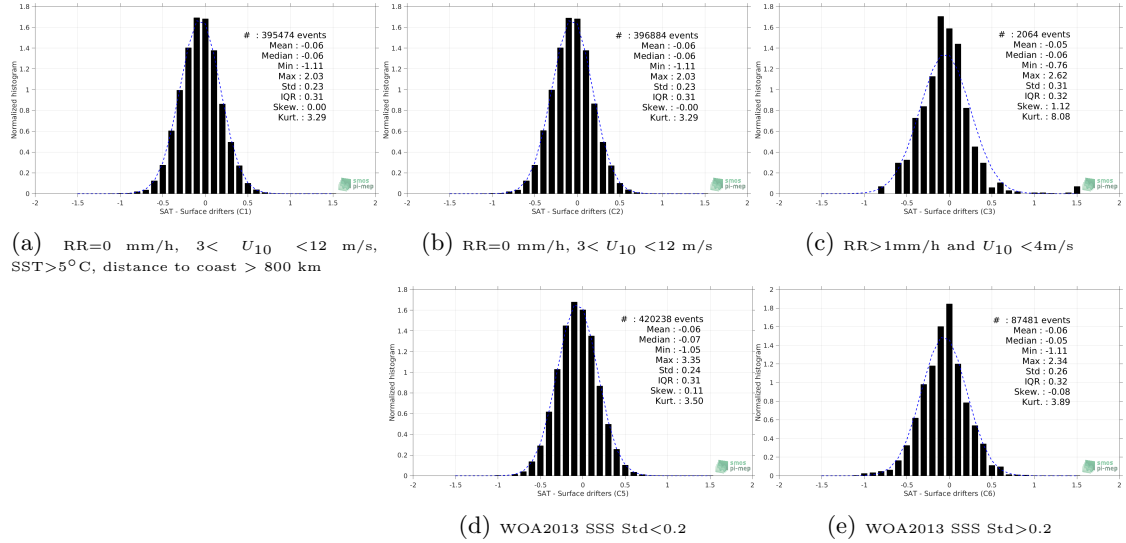
Figure 12: Normalized histogram of \Delta SSS (SMOS-L3-CATDS-CPDC-V3-10DAYS-25KM - Surface drifters) for 5 different subdatasets corresponding to: RR=0 mm/h, 3 < U_{10} < 12 m/s, SST>5°C, distance to coast > 800 km (a), RR=0 mm/h, 3 < U_{10} < 12 m/s (b), RR>1mm/h and U_{10} < 4 m/s (c), WOA2013 SSS Std<0.2 (d), WOA2013 SSS Std>0.2 (e).
