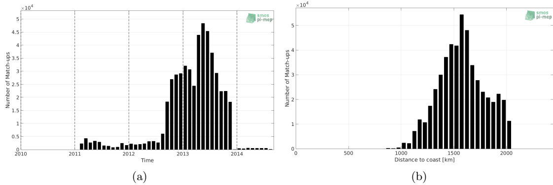
Figure 1: Number of match-ups between Surface drifters and SMOS-L3-CATDS-CPDC-V3-10DAYS-25KM SSS as a function of time (a) and as function of the distance to coast (b) over the SPURS 1 Pi-MEP region and for the full satellite product period.
