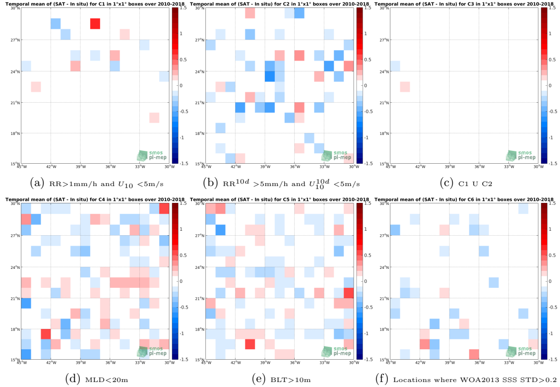
Figure 12: Temporal mean gridded over spatial boxes of size 1^\circ \times 1^\circ of \Delta\text{SSS} (SMOS-L3-CATDS-CPDC-V3-10DAYS-25KM - Argo) for 6 different subdatasets corresponding to: \text{RR} > 1\text{mm/h} and U_{10} < 5\text{m/s} (a), \text{RR}^{10d} > 5\text{mm/h} and U_{10}^{10d} < 5\text{m/s} (b), C1 U C2 (c), \text{MLD} < 20\text{m} (d), \text{BLT} > 10\text{m} (e), Locations where WOA2013 SSS STD > 0.2 (f).
