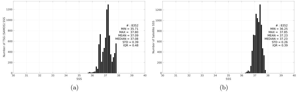
Figure 3: Histograms of SSS from TSG (SAMOS) (a) and SMOS SSS L3 v2 - 9-Days (BEC) (b) considering all match-up pairs per bins of 0.1 over the SPURS 1 Pi-MEP region and for the full satellite product period.
