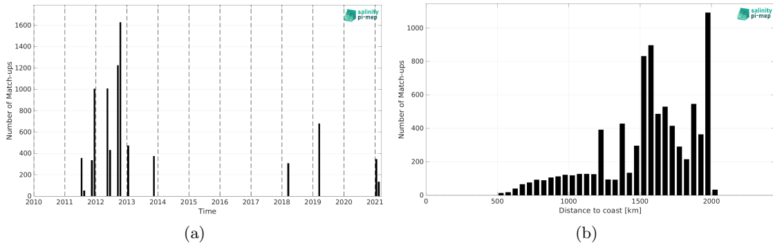
Figure 2: Number of match-ups between TSG (SAMOS) and SMOS SSS L3 v2 - 9-Days (BEC) SSS as a function of time (a) and as function of the distance to coast (b) over the SPURS 1 Pi-MEP region and for the full satellite product period.
