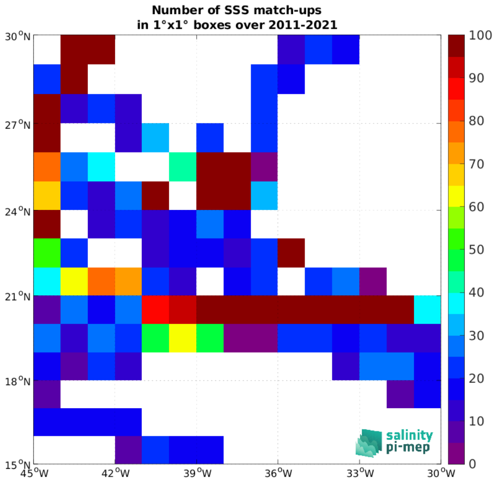
Figure 5: Number of SSS match-ups between TSG (SAMOS) SSS and the SMOS SSS L3 v2 - 9-Days (BEC) SSS product for the SPURS 1 Pi-MEP region over 1^\circ \times 1^\circ boxes and for the full satellite product period.
