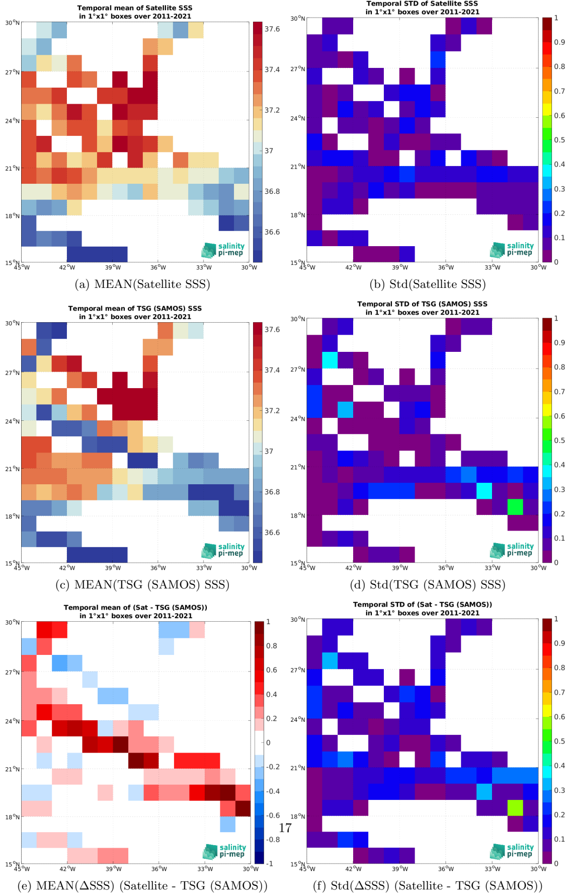
Figure 7: Temporal mean (left) and Std (right) of SSS from SMOS SSS L3 v2 - 9-Days (BEC) (top), TSG (SAMOS) (middle), and of \Delta SSS (Satellite - TSG (SAMOS)). Only match-up pairs are used to generate these maps.
