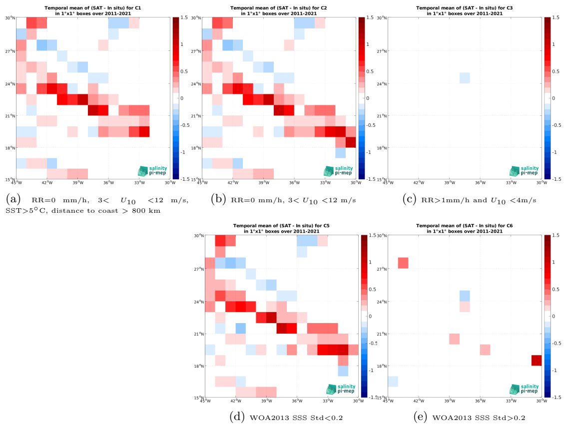
Figure 14: Temporal mean gridded over spatial boxes of size 1^\circ \times 1^\circ of \Delta SSS (SMOS SSS L3 v2 - 9-Days (BEC) - TSG (SAMOS)) for 5 different subdatasets corresponding to:RR=0 mm/h, 3 < U_{10} < 12 m/s, SST >5^\circ C, distance to coast > 800 km (a), RR=0 mm/h, 3 < U_{10} < 12 m/s (b), RR >1 mm/h and U_{10} < 4 m/s (c), WOA2013 SSS Std <0.2 (d), WOA2013 SSS Std >0.2 (e).
