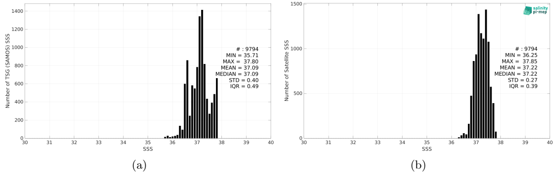
Figure 2: Histograms of SSS from TSG (SAMOS) (a) and SMOS SSS L3 v2 - 9-Days (BEC) (b) considering all match-up pairs per bins of 0.1 over the SPURS 1 Pi-MEP region and for the full satellite product period.
