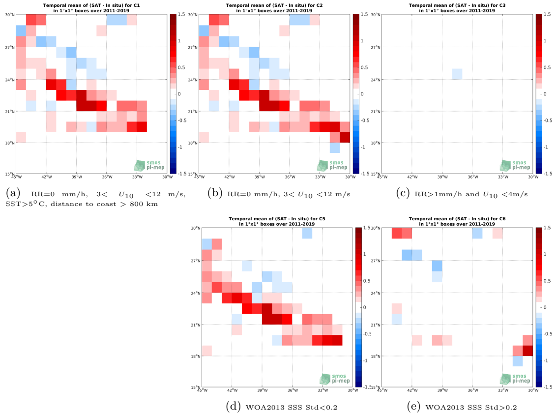
Figure 12: Temporal mean gridded over spatial boxes of size 1^\circ \times 1^\circ of \Delta SSS (SMOS SSS L3 v2 - 9-Days (BEC) - TSG (SAMOS)) for 5 different subdatasets corresponding to: RR=0 mm/h, 3 < U_{10} < 12 m/s, SST > 5^\circ C , distance to coast > 800 km (a), RR=0 mm/h, 3 < U_{10} < 12 m/s (b), RR > 1 mm/h and U_{10} < 4 m/s (c), WOA2013 SSS Std < 0.2 (d), WOA2013 SSS Std > 0.2 (e).
