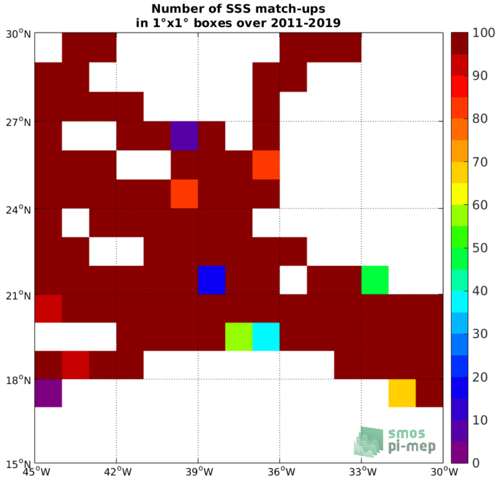
Figure 4: Number of SSS match-ups between TSG (SAMOS) SSS and the SMOS SSS L3 v2 - 9-Days (BEC) SSS product for the SPURS 1 Pi-MEP region over 1^\circ \times 1^\circ boxes and for the full satellite product period.
