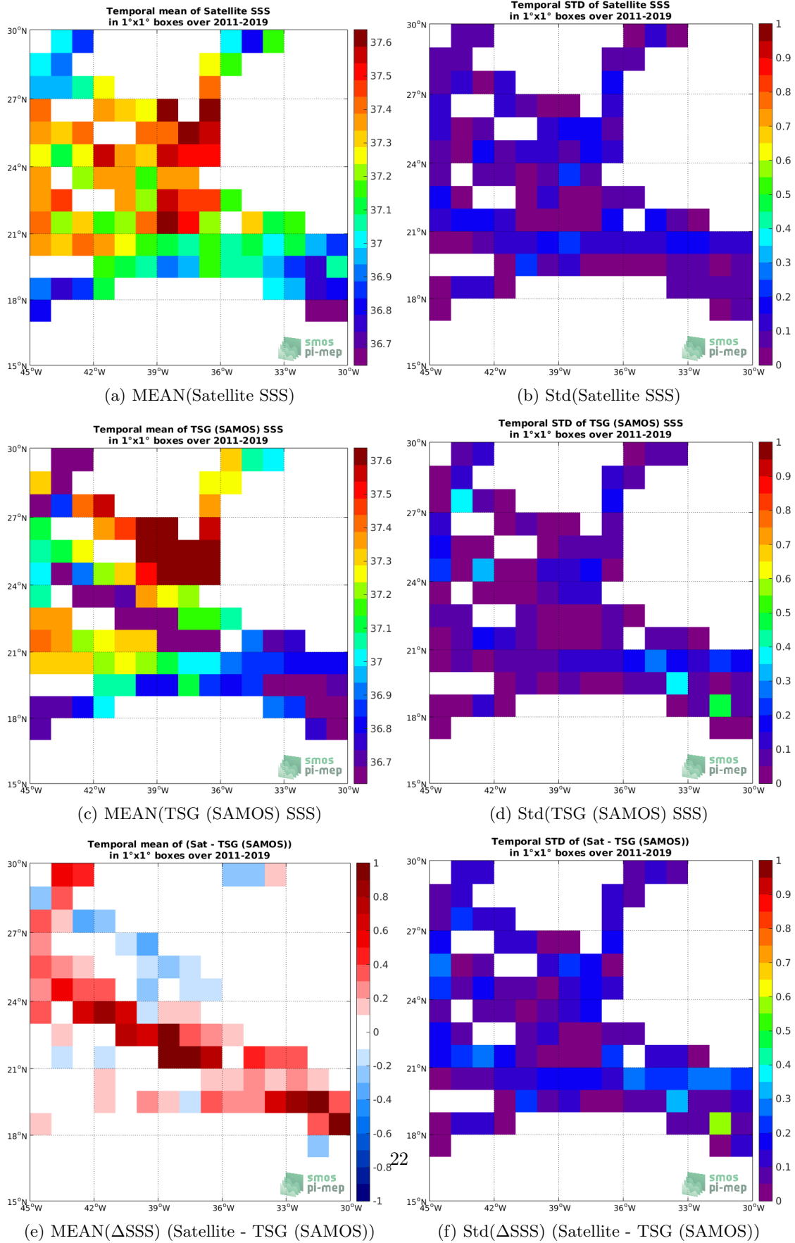
Figure 6: Temporal mean (left) and Std (right) of SSS from SMOS SSS L3 v2 - 9-Days (BEC) (top), TSG (SAMOS) (middle), and of \Delta SSS (Satellite - TSG (SAMOS)). Only match-up pairs are used to generate these maps.
