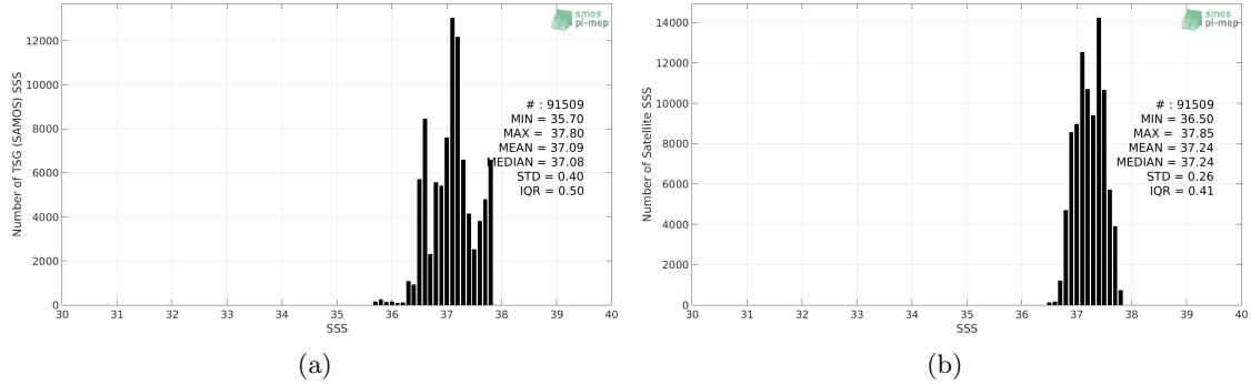
Figure 2: Histograms of SSS from TSG (SAMOS) (a) and SMOS SSS L3 v2 - 9-Days (BEC) (b) considering all match-up pairs per bins of 0.1 over the SPURS 1 Pi-MEP region and for the full satellite product period.
