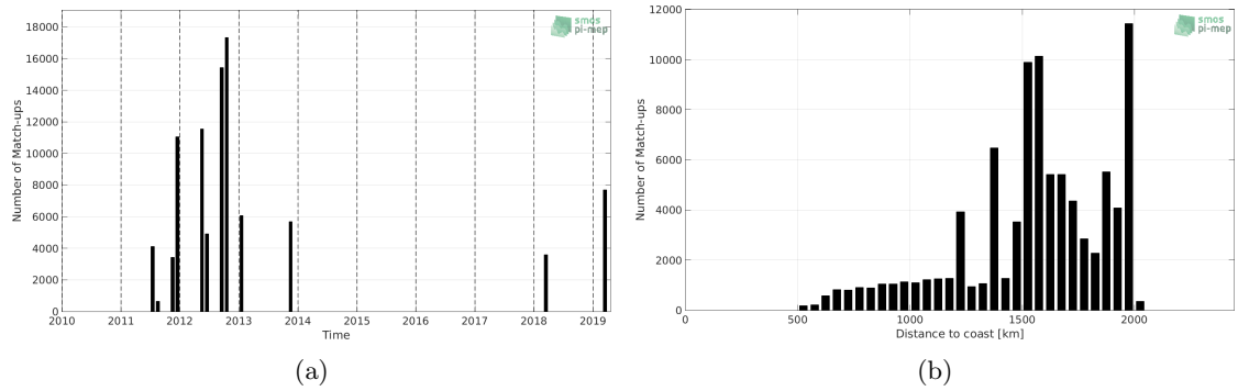
Figure 1: Number of match-ups between TSG (SAMOS) and SMOS SSS L3 v2 - 9-Days (BEC) SSS as a function of time (a) and as function of the distance to coast (b) over the SPURS 1 Pi-MEP region and for the full satellite product period.
