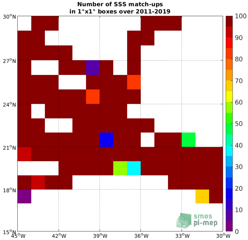
Figure 4: Number of SSS match-ups between TSG (SAMOS) SSS and the SMOS SSS L3 v2 - 9-Days (BEC) SSS product for the SPURS 1 Pi-MEP region over 1°x1° boxes and for the full satellite product period.
