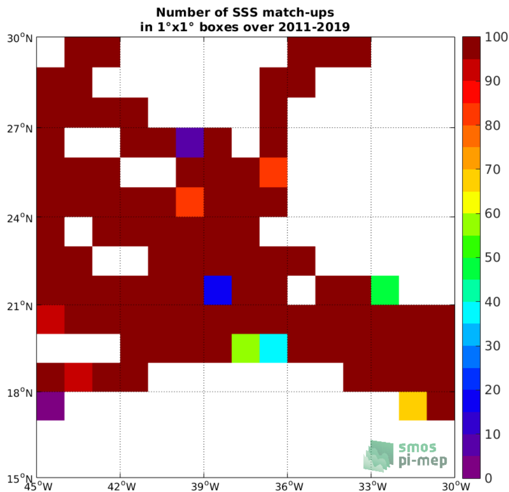
Figure 4: Number of SSS match-ups between TSG (SAMOS) SSS and the SMOS L3 v2 - 9-Days (BEC) SSS product for the SPURS 1 Pi-MEP region over 1°x1° boxes and for the full satellite product period.
