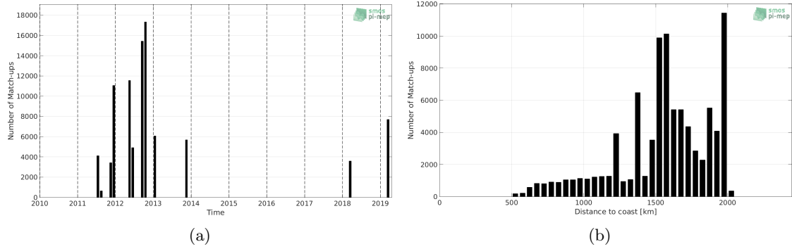
Figure 1: Number of match-ups between TSG (SAMOS) and SMOS L3 v2 - 9-Days (BEC) SSS as a function of time (a) and as function of the distance to coast (b) over the SPURS 1 Pi-MEP region and for the full satellite product period.
