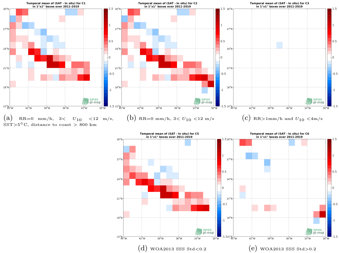
Figure 12: Temporal mean gridded over spatial boxes of size 1^\circ \times 1^\circ of \Delta SSS (SMOS L3 v2 - 9-Days (BEC) - TSG (SAMOS)) for 5 different subdatasets corresponding to: RR=0 mm/h, 3 < U_{10} < 12 m/s, SST > 5^\circ C , distance to coast > 800 km (a), RR=0 mm/h, 3 < U_{10} < 12 m/s (b), RR > 1 mm/h and U_{10} < 4 m/s (c), WOA2013 SSS Std < 0.2 (d), WOA2013 SSS Std > 0.2 (e).
