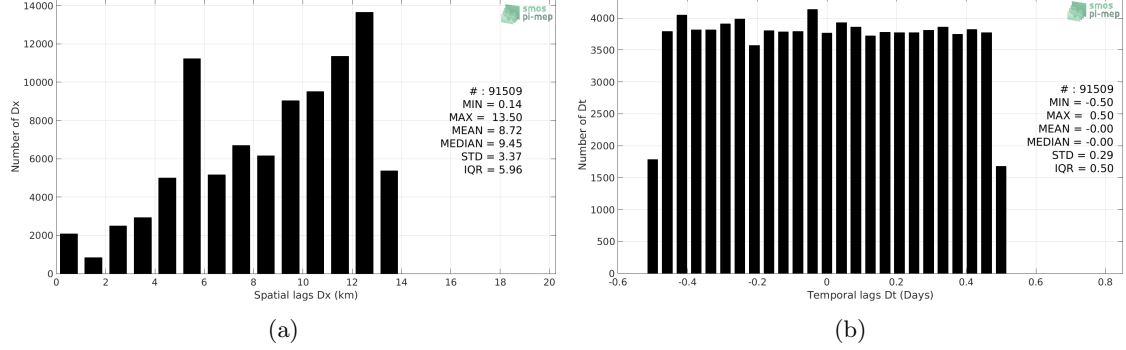
Figure 5: Histograms of the spatial (a) and temporal (b) lags between the time of the TSG (SAMOS) measurements and the date of the corresponding SMOS L3 v2 - 9-Days (BEC) SSS product.
