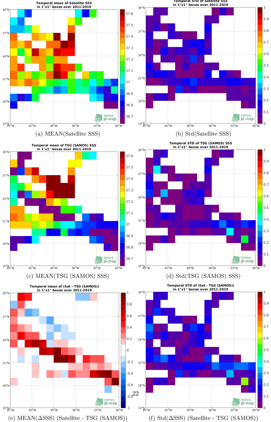
Figure 6: Temporal mean (left) and Std (right) of SSS from SMOS L3 v2 - 9-Days (BEC) (top), TSG (SAMOS) (middle), and of \Delta SSS (Satellite - TSG (SAMOS)). Only match-up pairs are used to generate these maps.
