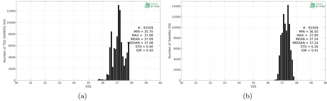
Figure 2: Histograms of SSS from TSG (SAMOS) (a) and SMOS L3 v2 - 9-Days (BEC) (b) considering all match-up pairs per bins of 0.1 over the SPURS 1 Pi-MEP region and for the full satellite product period.
