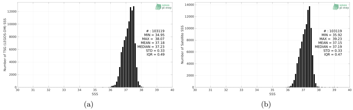
Figure 2: Histograms of SSS from TSG (LEGOS-DM) (a) and SMOS SSS L3 v2 - 9-Days (BEC) (b) considering all match-up pairs per bins of 0.1 over the SPURS 1 Pi-MEP region and for the full satellite product period.
