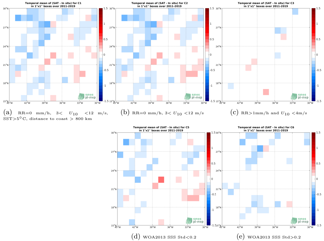
Figure 12: Temporal mean gridded over spatial boxes of size 1^\circ \times 1^\circ of \Delta SSS (SMOS SSS L3 v2 - 9-Days (BEC) - TSG (LEGOS-DM)) for 5 different subdatasets corresponding to: RR=0 mm/h, 3 < U_{10} < 12 m/s, SST>5°C, distance to coast > 800 km (a), RR=0 mm/h, 3 < U_{10} < 12 m/s (b), RR>1mm/h and U_{10} < 4 m/s (c), WOA2013 SSS Std<0.2 (d), WOA2013 SSS Std>0.2 (e).
