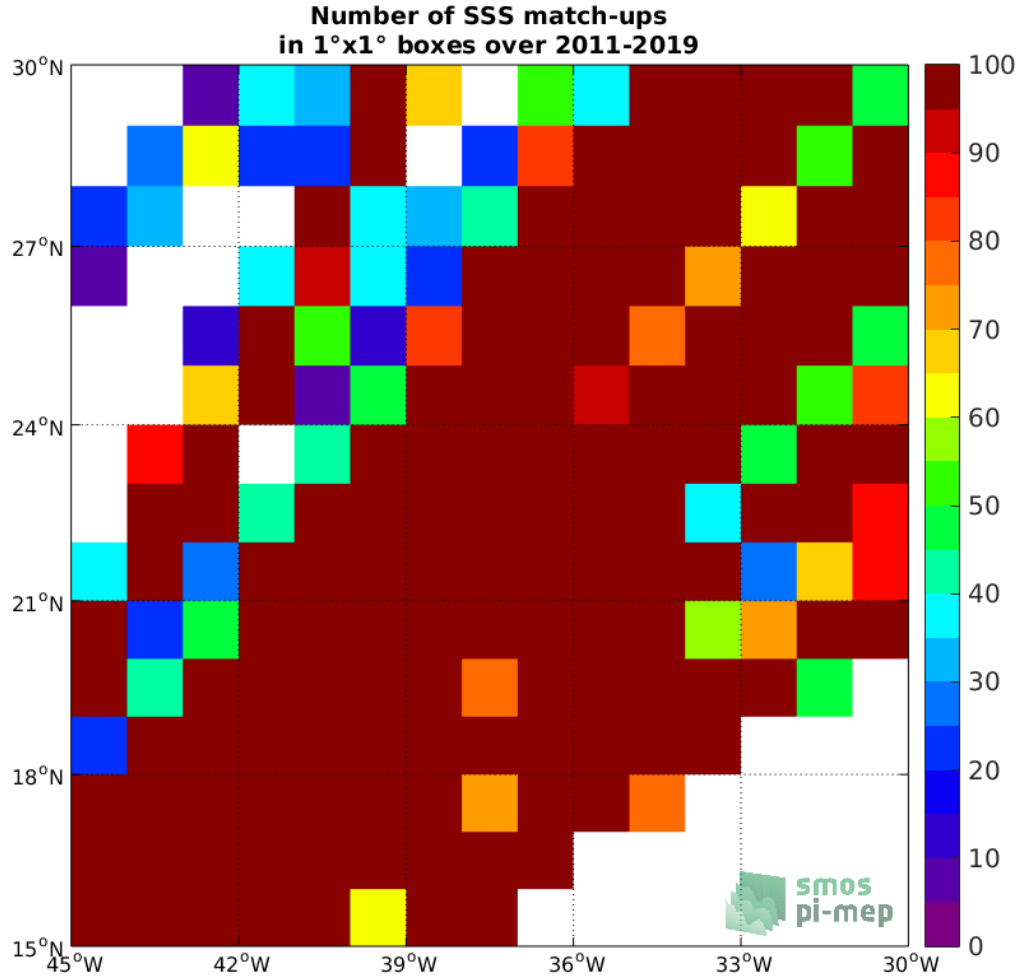
Figure 4: Number of SSS match-ups between TSG (LEGOS-DM) SSS and the SMOS SSS L3 v2 - 9-Days (BEC) SSS product for the SPURS 1 Pi-MEP region over 1^\circ \times 1^\circ boxes and for the full satellite product period.
