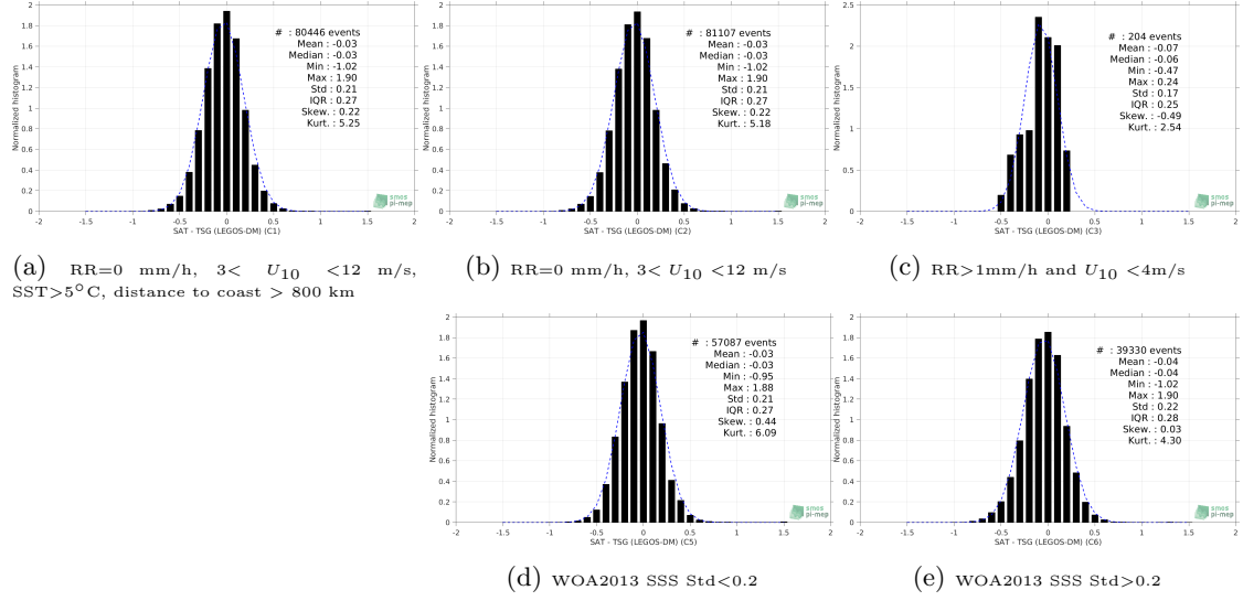
Figure 13: Normalized histogram of \Delta\text{SSS} (SMOS SSS L3 v2 - 9-Days (BEC) - TSG (LEGOS-DM)) for 5 different subdatasets corresponding to: RR=0 mm/h, 3 < U_{10} < 12 m/s, SST > 5^\circ\text{C} , distance to coast > 800 km (a), RR=0 mm/h, 3 < U_{10} < 12 m/s (b), RR > 1\text{mm/h} and U_{10} < 4\text{m/s} (c), WOA2013 SSS Std < 0.2 (d), WOA2013 SSS Std > 0.2 (e).
