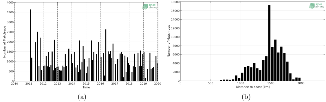
Figure 1: Number of match-ups between TSG (LEGOS-DM) and SMOS SSS L3 v2 - 9-Days (BEC) SSS as a function of time (a) and as function of the distance to coast (b) over the SPURS 1 Pi-MEP region and for the full satellite product period.
