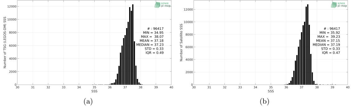
Figure 2: Histograms of SSS from TSG (LEGOS-DM) (a) and SMOS SSS L3 v2 - 9-Days (BEC) (b) considering all match-up pairs per bins of 0.1 over the SPURS 1 Pi-MEP region and for the full satellite product period.
