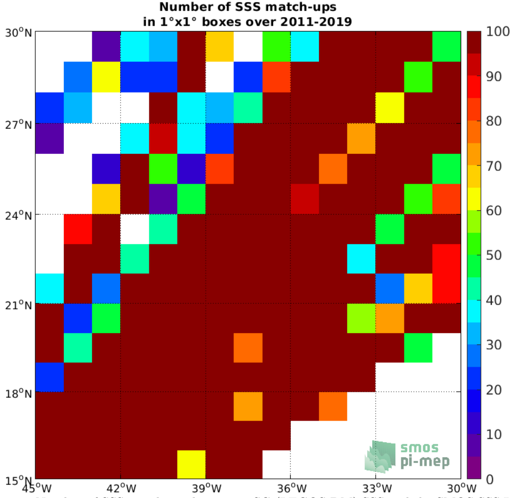
Figure 4: Number of SSS match-ups between TSG (LEGOS-DM) SSS and the SMOS SSS L3 v2 - 9-Days (BEC) SSS product for the SPURS 1 Pi-MEP region over 1°x1° boxes and for the full satellite product period.
