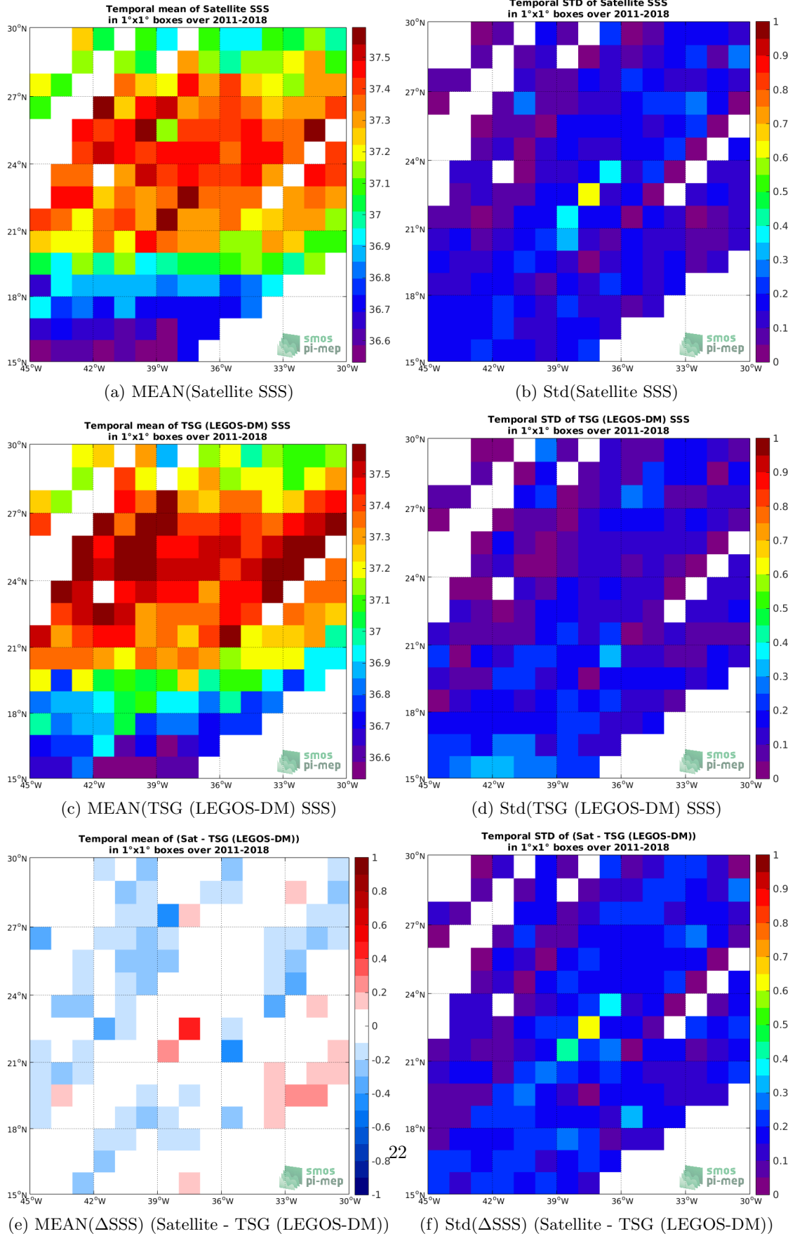
Figure 6: Temporal mean (left) and Std (right) of SSS from SMOS L3 v2- 9-Days (BEC) (top), TSG (LEGOS-DM) (middle), and of \Delta SSS (Satellite - TSG (LEGOS-DM)). Only match-up pairs are used to generate these maps.
