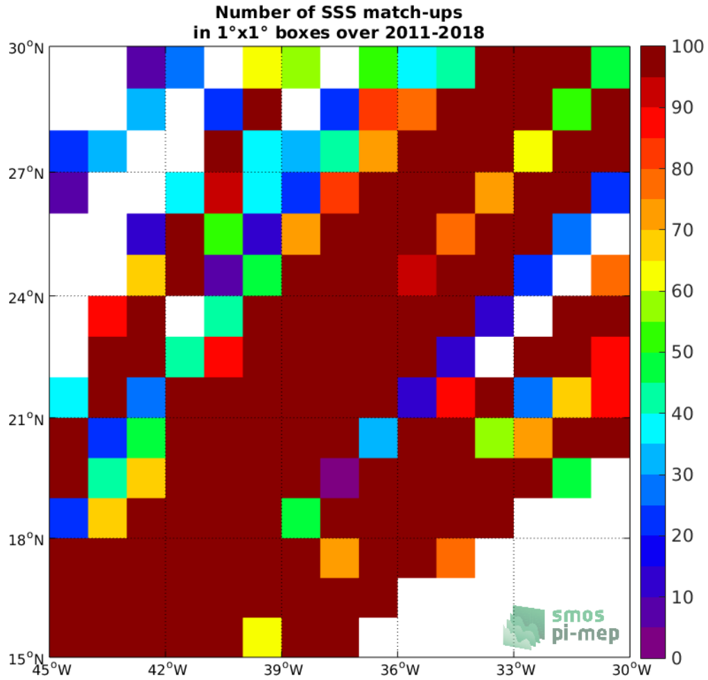
Figure 4: Number of SSS match-ups between TSG (LEGOS-DM) SSS and the SMOS L3 v2 - 9-Days (BEC) SSS product for the SPURS 1 Pi-MEP region over 1°x1° boxes and for the full satellite product period.
