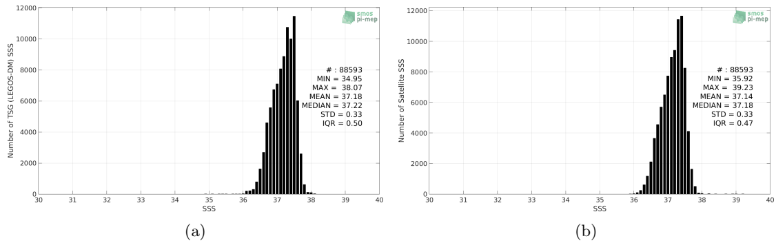
Figure 2: Histograms of SSS from TSG (LEGOS-DM) (a) and SMOS L3 v2 - 9-Days (BEC) (b) considering all match-up pairs per bins of 0.1 over the SPURS 1 Pi-MEP region and for the full satellite product period.
