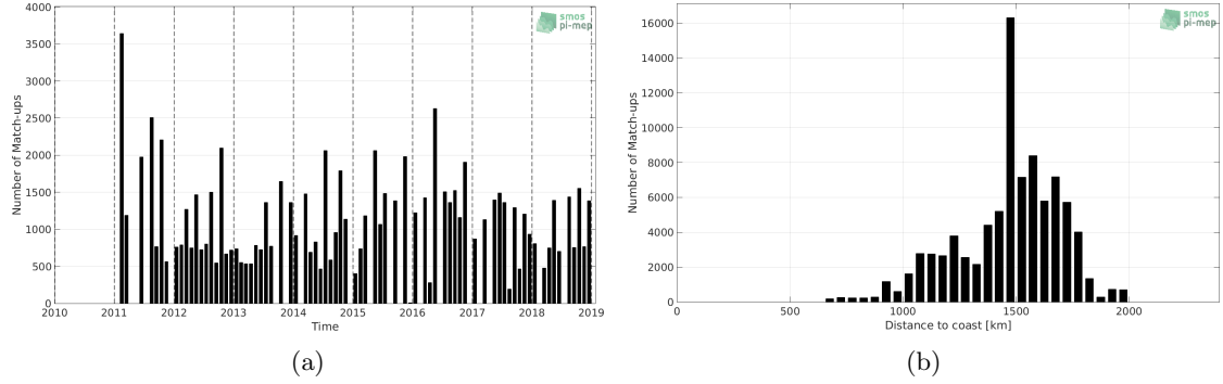
Figure 1: Number of match-ups between TSG (LEGOS-DM) and SMOS L3 v2 - 9-Days (BEC) SSS as a function of time (a) and as function of the distance to coast (b) over the SPURS 1 Pi-MEP region and for the full satellite product period.
