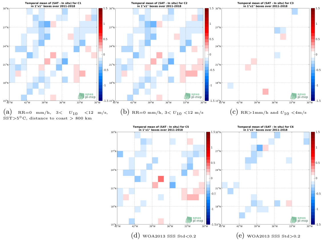
Figure 12: Temporal mean gridded over spatial boxes of size 1^\circ \times 1^\circ of \Delta SSS (SMOS L3 v2 - 9-Days (BEC) - TSG (LEGOS-DM)) for 5 different subdatasets corresponding to: RR=0 mm/h, 3 < U_{10} < 12 m/s, SST > 5^\circ C , distance to coast > 800 km (a), RR=0 mm/h, 3 < U_{10} < 12 m/s (b), RR > 1 mm/h and U_{10} < 4 m/s (c), WOA2013 SSS Std < 0.2 (d), WOA2013 SSS Std > 0.2 (e).
