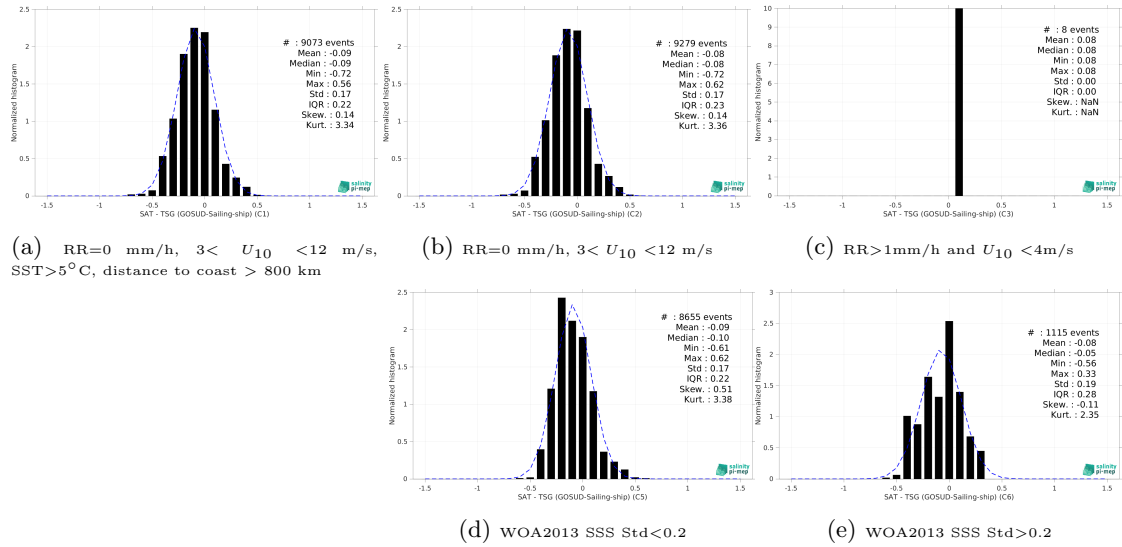
Figure 15: Normalized histogram of \Delta\text{SSS} (SMOS SSS L3 v2 - 9-Days (BEC) - TSG (GOSUD-Sailing-ship)) for 5 different subdatasets corresponding to: RR=0 mm/h, 3 < U_{10} < 12 m/s, SST > 5^\circ\text{C} , distance to coast > 800 km (a), RR=0 mm/h, 3 < U_{10} < 12 m/s (b), RR > 1\text{mm/h} and U_{10} < 4\text{m/s} (c), WOA2013 SSS Std < 0.2 (d), WOA2013 SSS Std > 0.2 (e).
