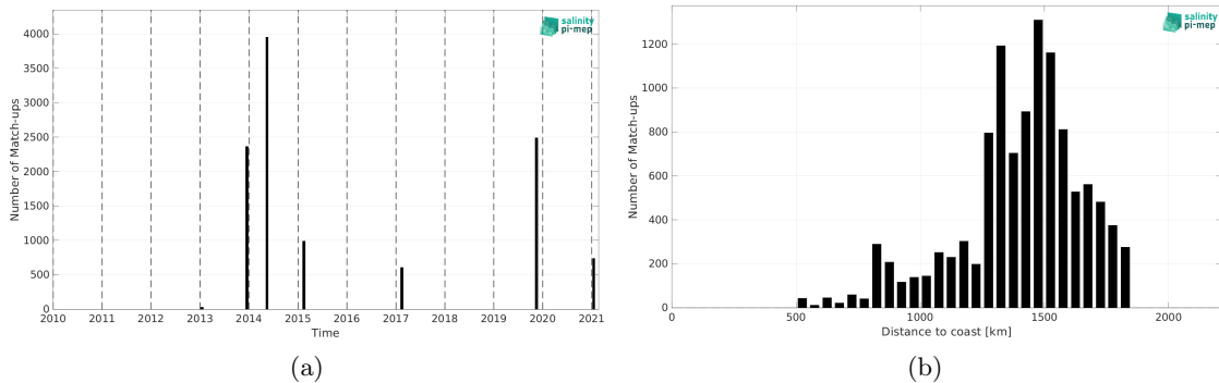
Figure 2: Number of match-ups between TSG (GOSUD-Sailing-ship) and SMOS SSS L3 v2 - 9-Days (BEC) SSS as a function of time (a) and as function of the distance to coast (b) over the SPURS 1 Pi-MEP region and for the full satellite product period.
