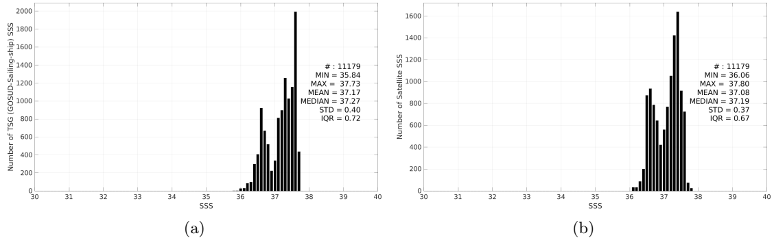
Figure 3: Histograms of SSS from TSG (GOSUD-Sailing-ship) (a) and SMOS SSS L3 v2 - 9-Days (BEC) (b) considering all match-up pairs per bins of 0.1 over the SPURS 1 Pi-MEP region and for the full satellite product period.
