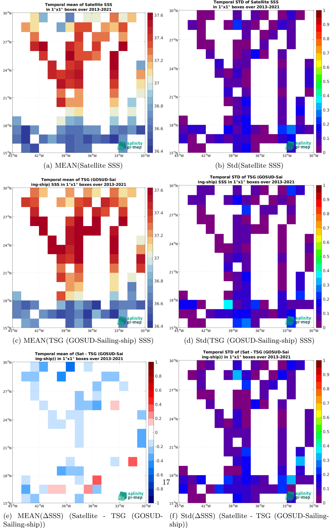
Figure 7: Temporal mean (left) and Std (right) of SSS from SMOS SSS L3 v2 - 9-Days (BEC) (top), TSG (GOSUD-Sailing-ship) (middle), and of \Delta SSS (Satellite - TSG (GOSUD-Sailing-ship)). Only match-up pairs are used to generate these maps.
