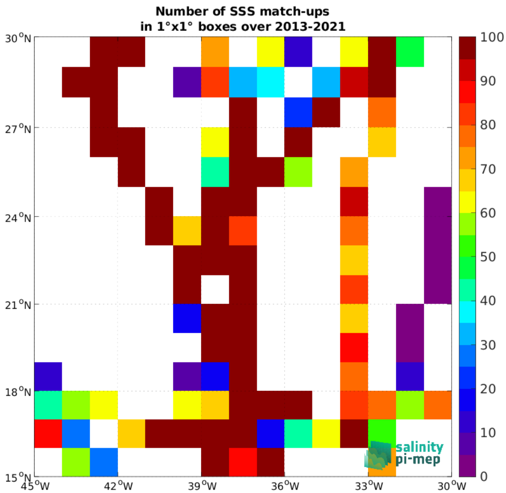
Figure 5: Number of SSS match-ups between TSG (GOSUD-Sailing-ship) SSS and the SMOS SSS L3 v2 - 9-Days (BEC) SSS product for the SPURS 1 Pi-MEP region over 1°x1° boxes and for the full satellite product period.
