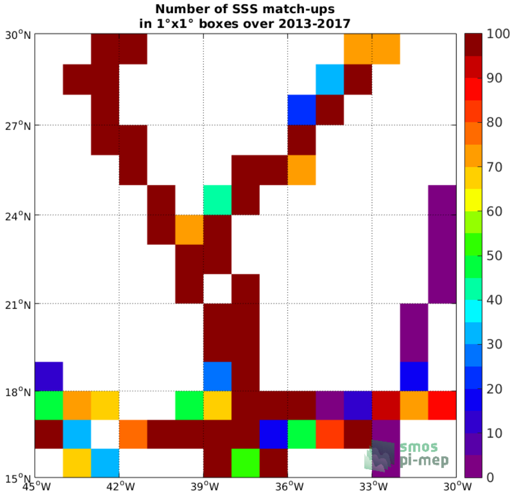
Figure 4: Number of SSS match-ups between TSG (GOSUD-Sailing-ship) SSS and the SMOS SSS L3 v2 - 9-Days (BEC) SSS product for the SPURS 1 Pi-MEP region over 1°×1° boxes and for the full satellite product period.
