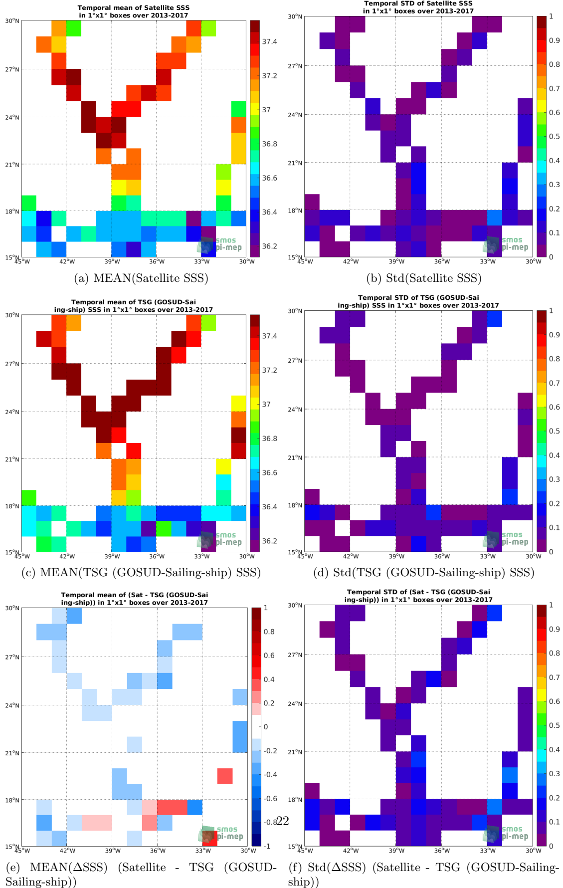
Figure 6: Temporal mean (left) and Std (right) of SSS from SMOS SSS L3 v2 - 9-Days (BEC) (top), TSG (GOSUD-Sailing-ship) (middle), and of \Delta SSS (Satellite - TSG (GOSUD-Sailing-ship)). Only match-up pairs are used to generate these maps.
