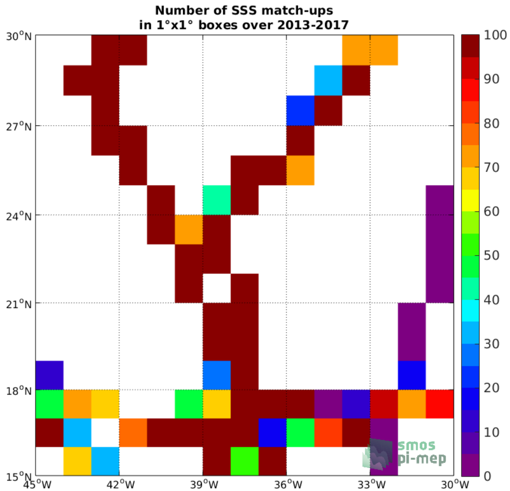
Figure 4: Number of SSS match-ups between TSG (GOSUD-Sailing-ship) SSS and the SMOS L3 v2 - 9-Days (BEC) SSS product for the SPURS 1 Pi-MEP region over 1°x1° boxes and for the full satellite product period.
