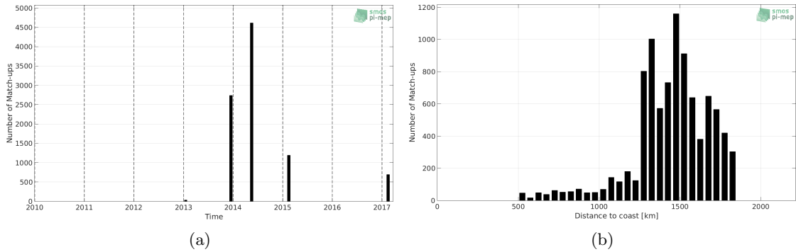
Figure 1: Number of match-ups between TSG (GOSUD-Sailing-ship) and SMOS L3 v2 - 9-Days (BEC) SSS as a function of time (a) and as function of the distance to coast (b) over the SPURS 1 Pi-MEP region and for the full satellite product period.
