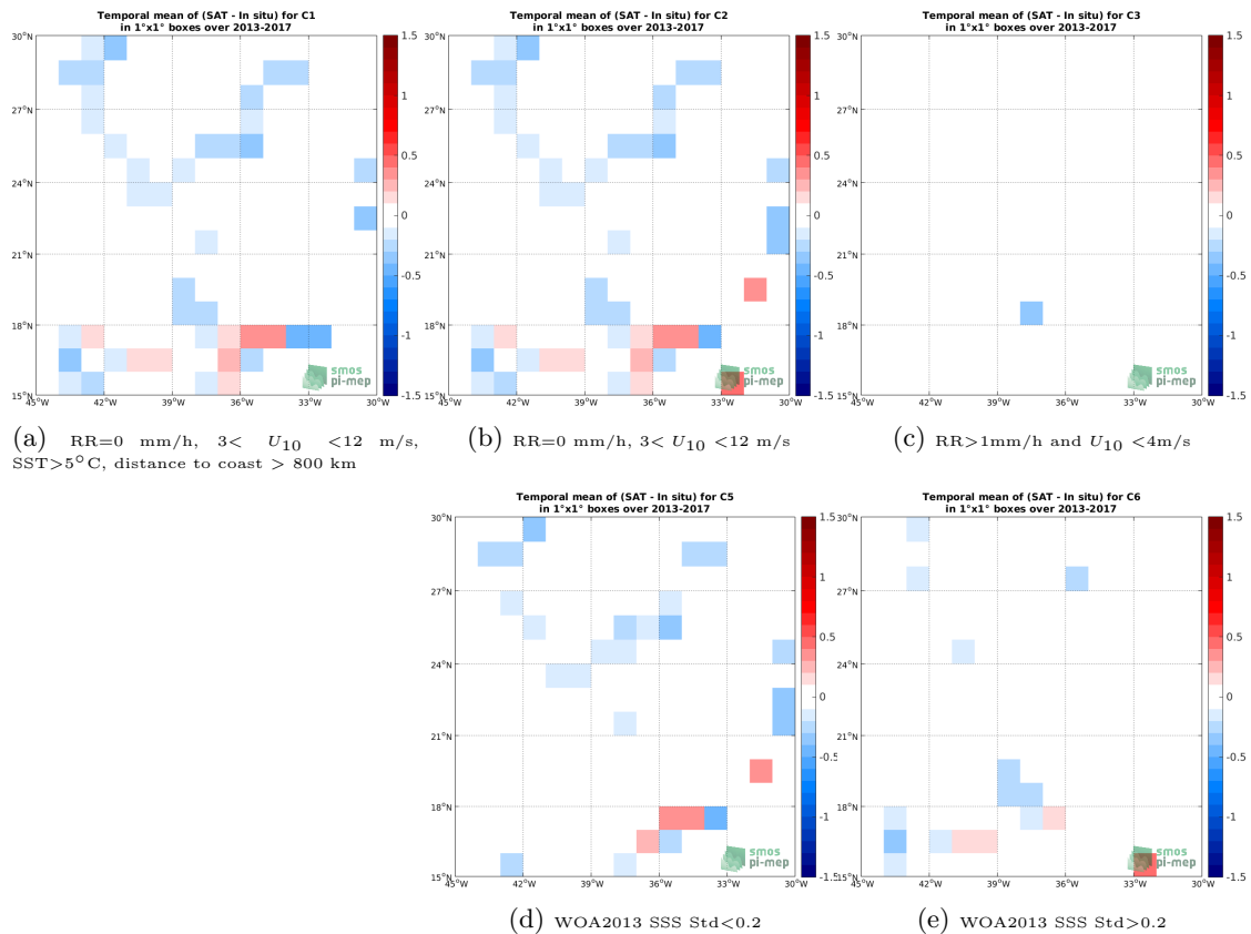
Figure 12: Temporal mean gridded over spatial boxes of size 1^\circ \times 1^\circ of \Delta\text{SSS} (SMOS L3 v2 - 9-Days (BEC) - TSG (GOSUD-Sailing-ship)) for 5 different subdatasets corresponding to:RR=0 mm/h, 3 < U_{10} < 12 m/s, SST>5°C, distance to coast > 800 km (a), RR=0 mm/h, 3 < U_{10} < 12 m/s (b), RR>1mm/h and U_{10} < 4 m/s (c), WOA2013 SSS Std<0.2 (d), WOA2013 SSS Std>0.2 (e).
