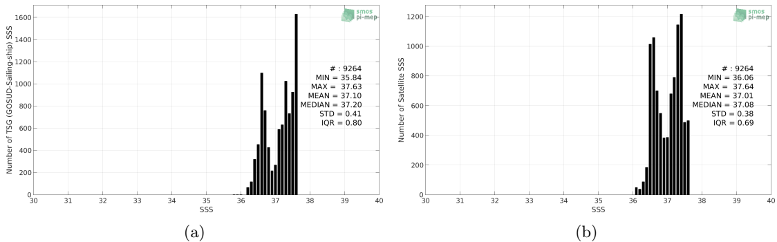
Figure 2: Histograms of SSS from TSG (GOSUD-Sailing-ship) (a) and SMOS L3 v2 - 9-Days (BEC) (b) considering all match-up pairs per bins of 0.1 over the SPURS 1 Pi-MEP region and for the full satellite product period.
