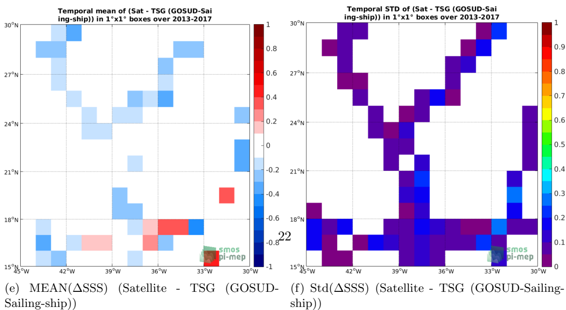
Figure 6: Temporal mean (left) and Std (right) of SSS from SMOS L3 v2 - 9-Days (BEC) (top), TSG (GOSUD-Sailing-ship) (middle), and of \Delta SSS (Satellite - TSG (GOSUD-Sailing-ship)). Only match-up pairs are used to generate these maps.
