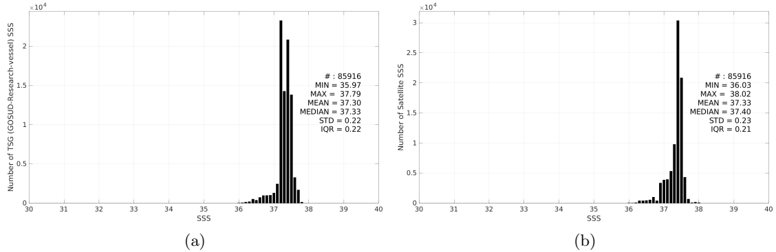
Figure 3: Histograms of SSS from TSG (GOSUD-Research-vessel) (a) and SMOS SSS L3 v2 - 9-Days (BEC) (b) considering all match-up pairs per bins of 0.1 over the SPURS 1 Pi-MEP region and for the full satellite product period.
