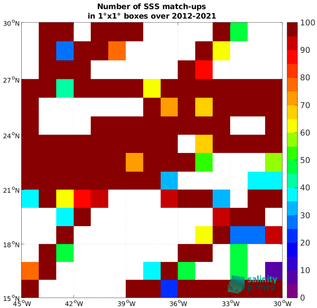
Figure 5: Number of SSS match-ups between TSG (GOSUD-Research-vessel) SSS and the SMOS SSS L3 v2 - 9-Days (BEC) SSS product for the SPURS 1 Pi-MEP region over 1^\circ \times 1^\circ boxes and for the full satellite product period.
