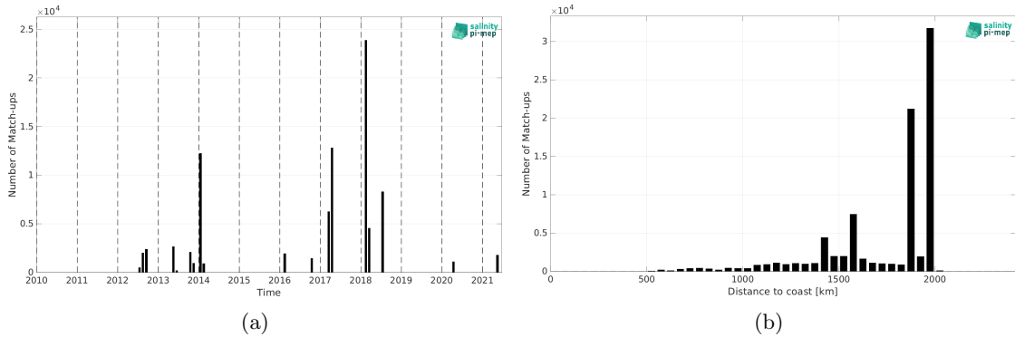
Figure 2: Number of match-ups between TSG (GOSUD-Research-vessel) and SMOS SSS L3 v2 - 9-Days (BEC) SSS as a function of time (a) and as function of the distance to coast (b) over the SPURS 1 Pi-MEP region and for the full satellite product period.
