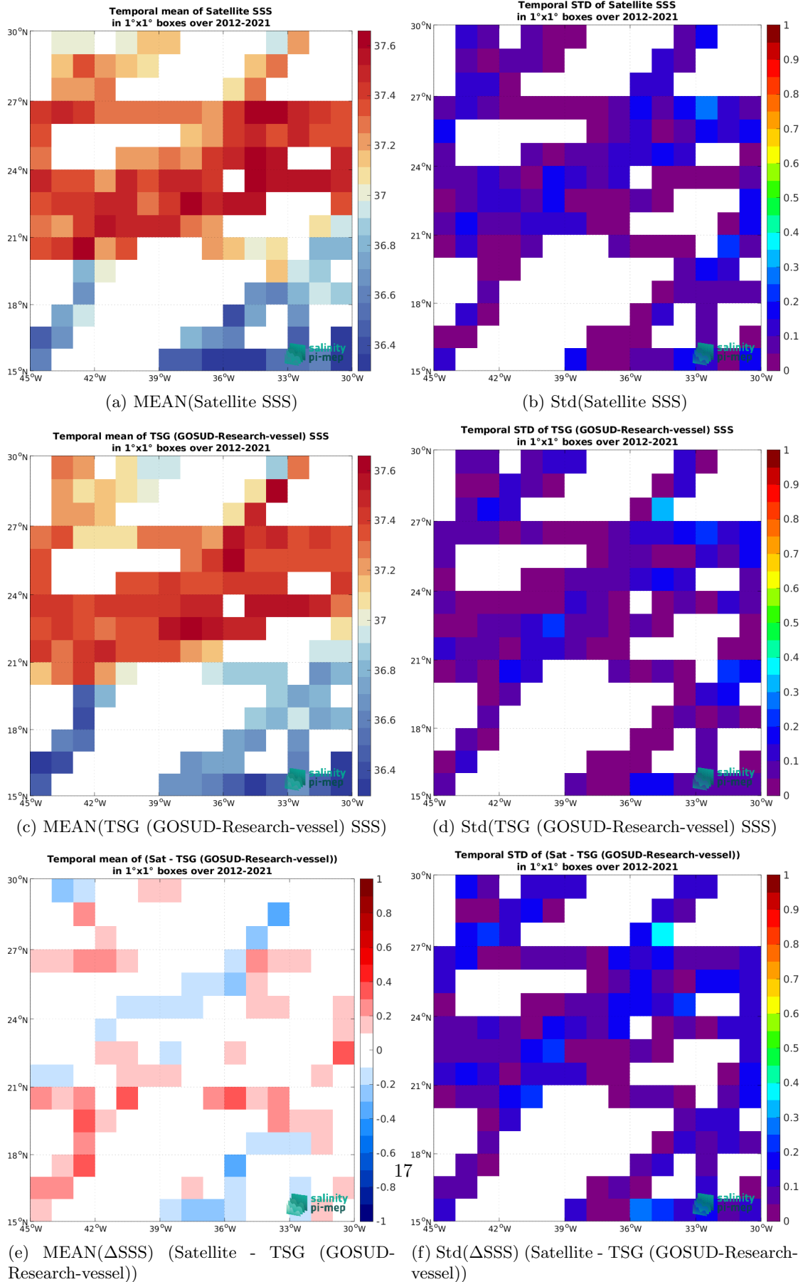
Figure 7: Temporal mean (left) and Std (right) of SSS from SMOS SSS L3 v2 - 9-Days (BEC) (top), TSG (GOSUD-Research-vessel) (middle), and of \Delta\text{SSS} (Satellite - TSG (GOSUD-Research-vessel)). Only match-up pairs are used to generate these maps.
