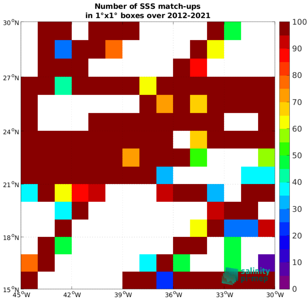
Figure 5: Number of SSS match-ups between TSG (GOSUD-Research-vessel) SSS and the SMOS SSS L3 v2 - 9-Days (BEC) SSS product for the SPURS 1 Pi-MEP region over 1°x1° boxes and for the full satellite product period.
