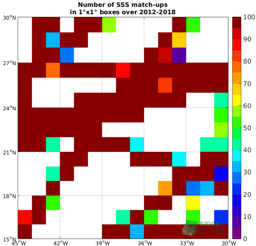
Figure 4: Number of SSS match-ups between TSG (GOSUD-Research-vessel) SSS and the SMOS SSS L3 v2 - 9-Days (BEC) SSS product for the SPURS 1 Pi-MEP region over 1^\circ \times 1^\circ boxes and for the full satellite product period.
