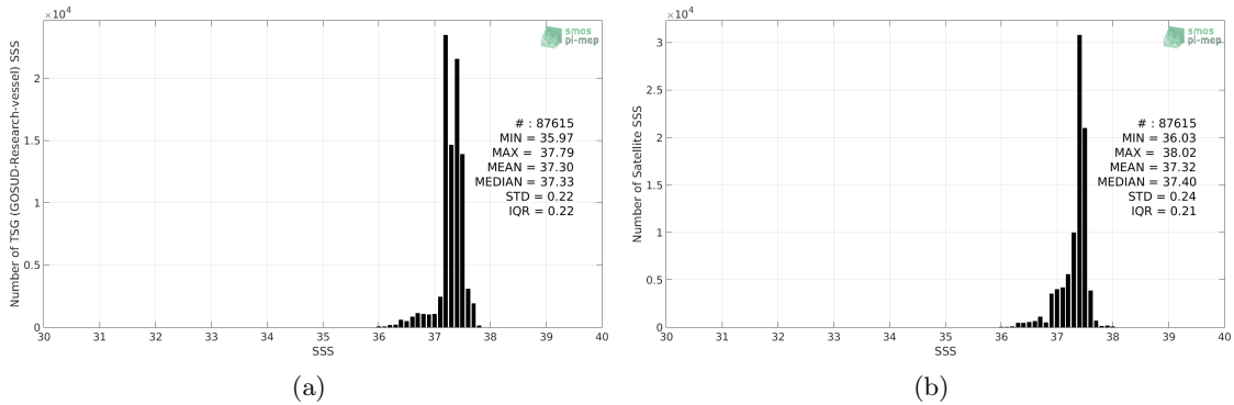
Figure 2: Histograms of SSS from TSG (GOSUD-Research-vessel) (a) and SMOS L3 v2 - 9-Days (BEC) (b) considering all match-up pairs per bins of 0.1 over the SPURS 1 Pi-MEP region and for the full satellite product period.
