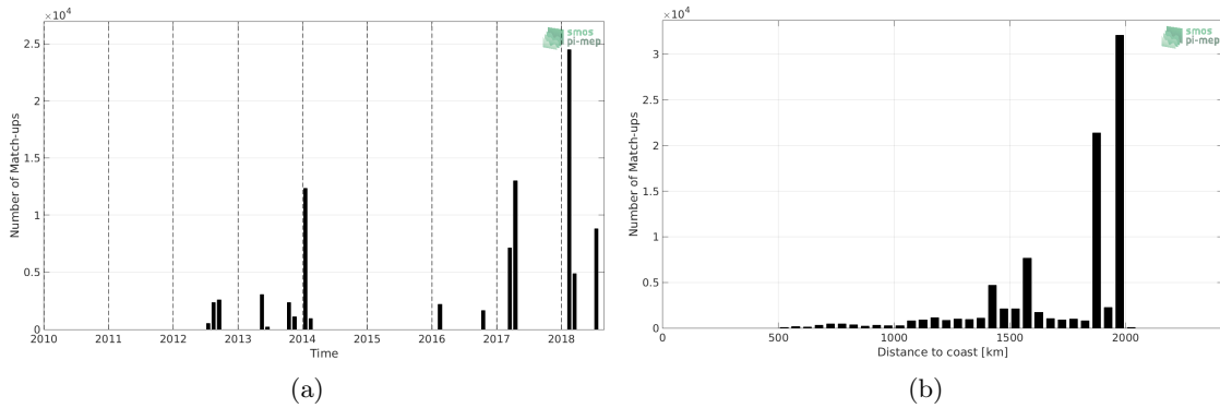
Figure 1: Number of match-ups between TSG (GOSUD-Research-vessel) and SMOS L3 v2 - 9-Days (BEC) SSS as a function of time (a) and as function of the distance to coast (b) over the SPURS 1 Pi-MEP region and for the full satellite product period.
