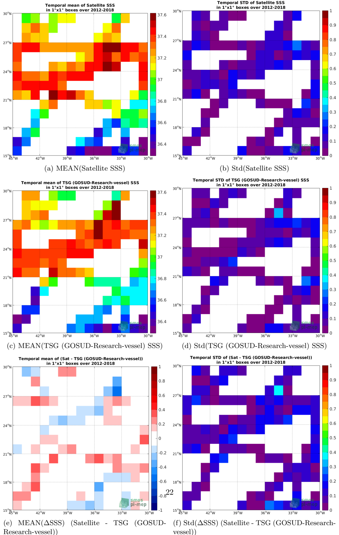
Figure 6: Temporal mean (left) and Std (right) of SSS from SMOS L3 v2 - 9-Days (BEC) (top), TSG (GOSUD-Research-vessel) (middle), and of \Delta SSS (Satellite - TSG (GOSUD-Research-vessel)). Only match-up pairs are used to generate these maps.
