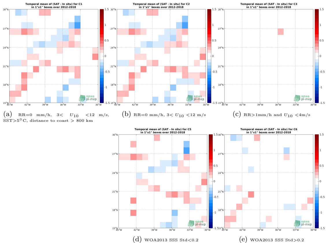
Figure 12: Temporal mean gridded over spatial boxes of size 1^\circ \times 1^\circ of \Delta\text{SSS} (SMOS L3 v2 - 9-Days (BEC) - TSG (GOSUD-Research-vessel)) for 5 different subdatasets corresponding to:RR=0 mm/h, 3 < U_{10} < 12 m/s, SST>5°C, distance to coast > 800 km (a), RR=0 mm/h, 3 < U_{10} < 12 m/s (b), RR>1mm/h and U_{10} < 4 m/s (c), WOA2013 SSS Std<0.2 (d), WOA2013 SSS Std>0.2 (e).
