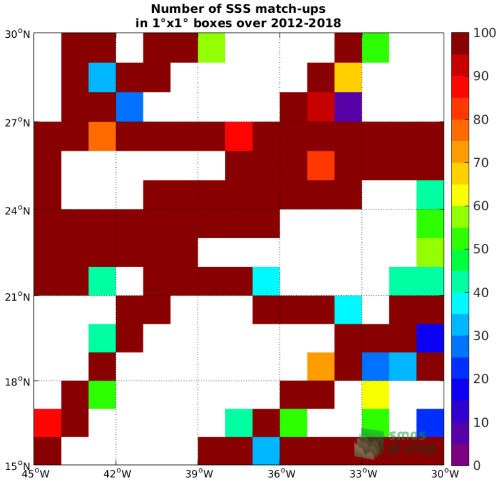
Figure 4: Number of SSS match-ups between TSG (GOSUD-Research-vessel) SSS and the SMOS L3 v2 - 9-Days (BEC) SSS product for the SPURS 1 Pi-MEP region over 1°x1° boxes and for the full satellite product period.
