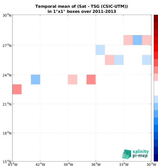
(e) MEAN( \Delta SSS) (Satellite - TSG (CSIC-UTM))
