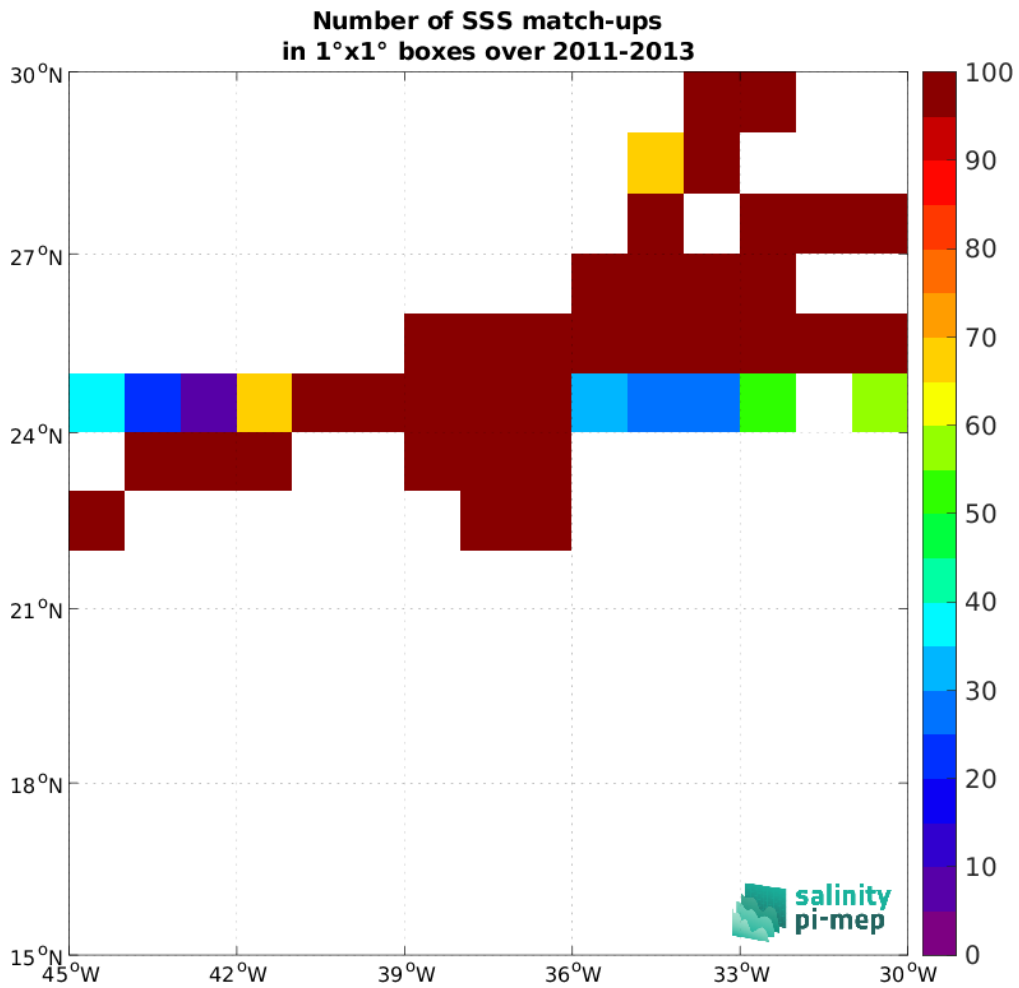
Figure 4: Number of SSS match-ups between TSG (CSIC-UTM) SSS and the SMOS SSS L3 v2 - 9-Days (BEC) SSS product for the SPURS 1 Pi-MEP region over 1°x1° boxes and for the full satellite product period.
