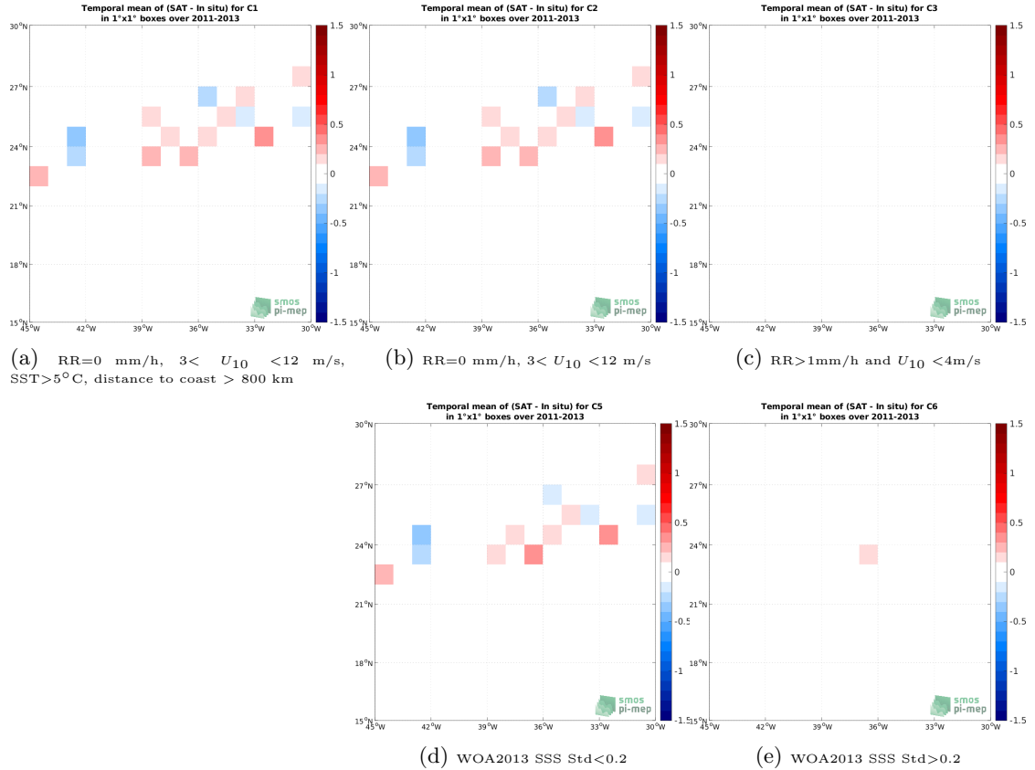
Figure 12: Temporal mean gridded over spatial boxes of size 1^{\circ}\times 1^{\circ} of \Delta\text{SSS} (SMOS SSS L3 v2 - 9-Days (BEC) - TSG (CSIC-UTM)) for 5 different subdatasets corresponding to:RR=0 mm/h, 3 < U_{10} < 12 m/s, SST >5^{\circ}\text{C} , distance to coast > 800 km (a), RR=0 mm/h, 3 < U_{10} < 12 m/s (b), RR >1 mm/h and U_{10} < 4 m/s (c), WOA2013 SSS Std <0.2 (d), WOA2013 SSS Std >0.2 (e).
