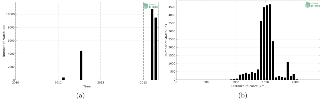
Figure 1: Number of match-ups between TSG (CSIC-UTM) and SMOS SSS L3 v2 - 9-Days (BEC) SSS as a function of time (a) and as function of the distance to coast (b) over the SPURS 1 Pi-MEP region and for the full satellite product period.
