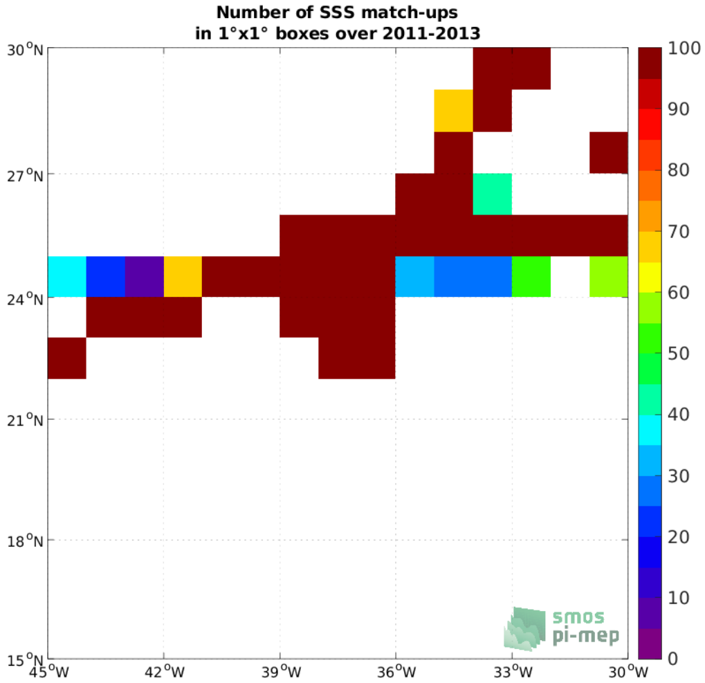
Figure 4: Number of SSS match-ups between TSG (CSIC-UTM) SSS and the SMOS SSS L3 v2 - 9-Days (BEC) SSS product for the SPURS 1 Pi-MEP region over 1^\circ \times 1^\circ boxes and for the full satellite product period.
