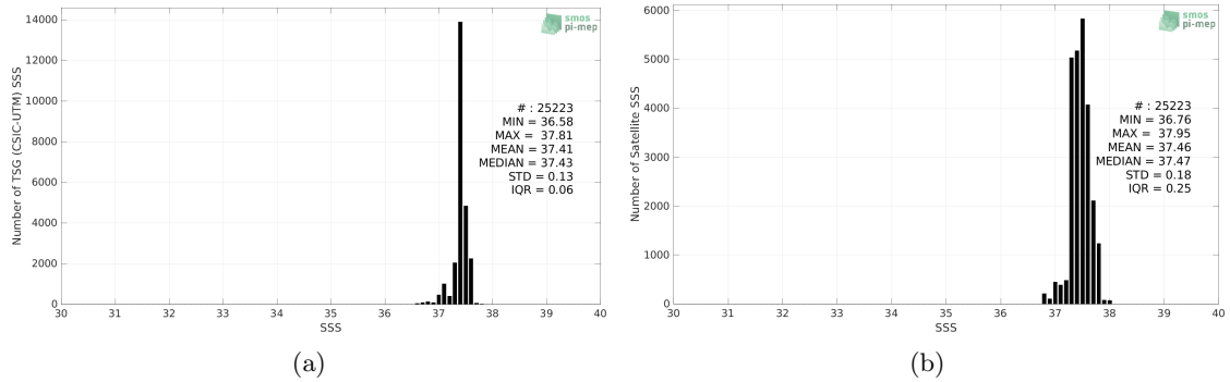
Figure 2: Histograms of SSS from TSG (CSIC-UTM) (a) and SMOS SSS L3 v2 - 9-Days (BEC) (b) considering all match-up pairs per bins of 0.1 over the SPURS 1 Pi-MEP region and for the full satellite product period.
