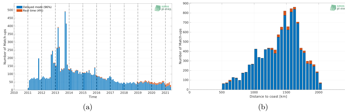
Figure 1: Number of match-ups between Argo and SMOS SSS L3 v2 - 9-Days (BEC) SSS as a function of time (a) and as function of the distance to coast (b) over the SPURS 1 Pi-MEP region and for the full satellite product period.
