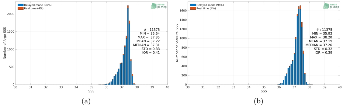
Figure 2: Histograms of SSS from Argo (a) and SMOS SSS L3 v2 - 9-Days (BEC) (b) considering all match-up pairs per bins of 0.1 over the SPURS 1 Pi-MEP region and for the full satellite product period.
