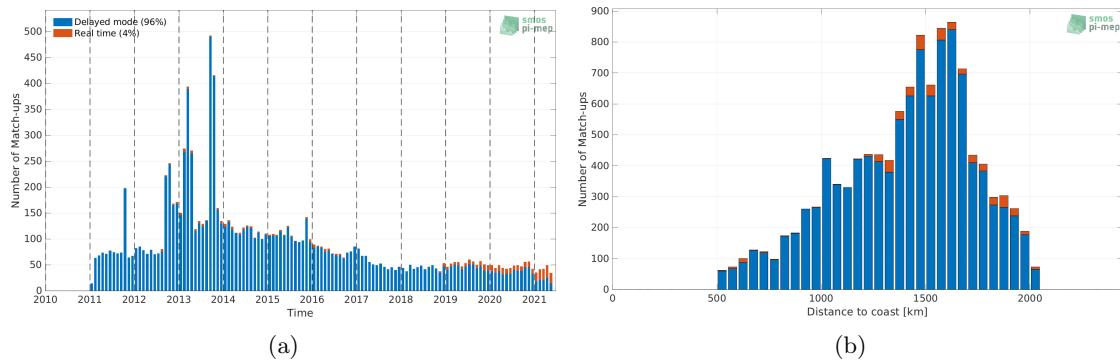
Figure 1: Number of match-ups between Argo and SMOS SSS L3 v2 - 9-Days (BEC) SSS as a function of time (a) and as function of the distance to coast (b) over the SPURS 1 Pi-MEP region and for the full satellite product period.
