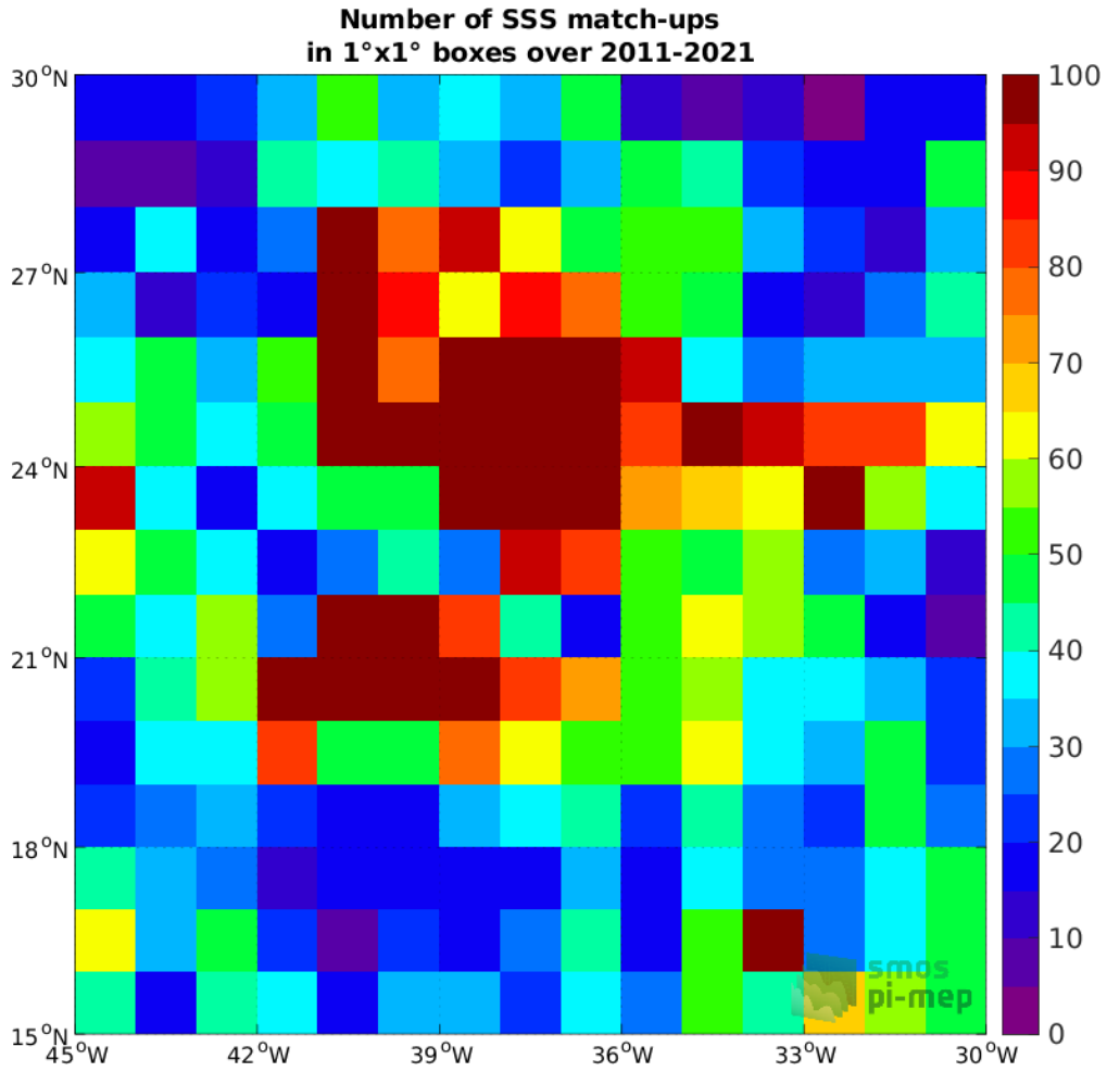
Figure 4: Number of SSS match-ups between Argo SSS and the SMOS SSS L3 v2 - 9-Days (BEC) SSS product for the SPURS 1 Pi-MEP region over 1°×1° boxes and for the full satellite product period.
