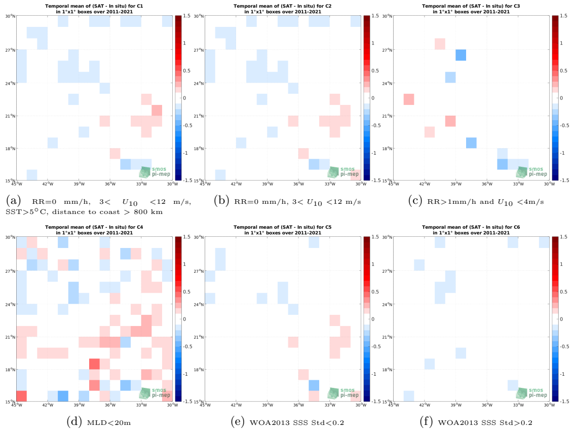
Figure 12: Temporal mean gridded over spatial boxes of size 1^\circ \times 1^\circ of \Delta SSS (SMOS SSS L3 v2 - 9-Days (BEC) - Argo) for 6 different subdatasets corresponding to:RR=0 mm/h, 3 < U_{10} < 12 m/s, SST >5^\circ C, distance to coast > 800 km (a), RR=0 mm/h, 3 < U_{10} < 12 m/s (b), RR >1 mm/h and U_{10} < 4 m/s (c),MLD <20 m (d),WOA2013 SSS Std <0.2 (e),WOA2013 SSS Std >0.2 (f).
