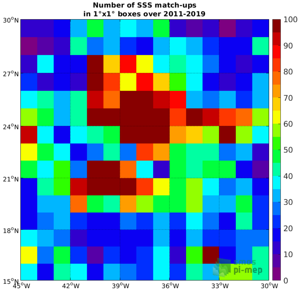
Figure 4: Number of SSS match-ups between Argo SSS and the SMOS SSS L3 v2 - 9-Days (BEC) SSS product for the SPURS 1 Pi-MEP region over 1°x1° boxes and for the full satellite product period.
