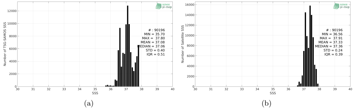
Figure 2: Histograms of SSS from TSG-SAMOS (a) and SMOS-L3-BEC-OA-V1-9DAYS-0.25DEG (b) considering all match-up pairs per bins of 0.1 over the SPURS 1 Pi-MEP region and for the full satellite product period.
