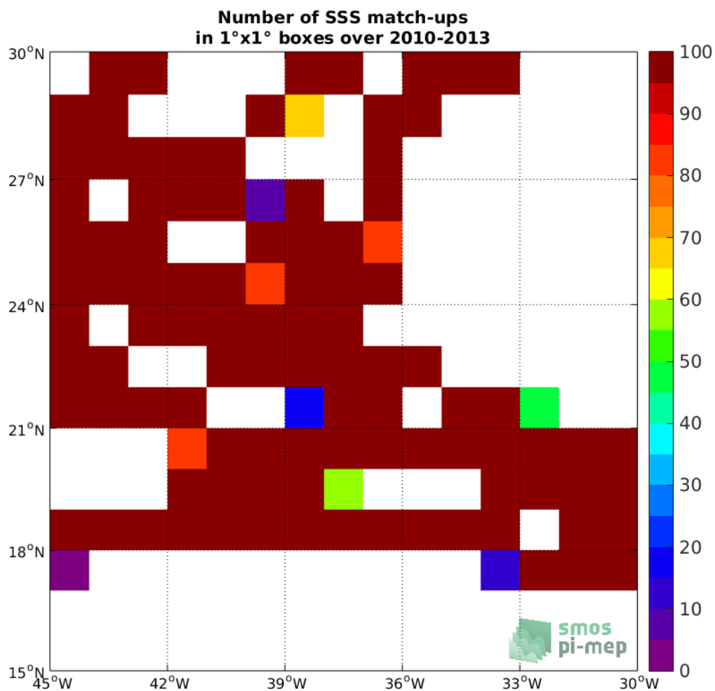
Figure 4: Number of SSS match-ups between TSG-SAMOS SSS and the SMOS-L3-BEC-OA-V1-9DAYS-0.25DEG SSS product for the SPURS 1 Pi-MEP region over 1°x1° boxes and for the full satellite product period.
