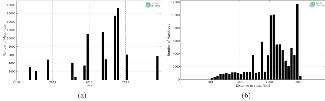
Figure 1: Number of match-ups between TSG-SAMOS and SMOS-L3-BEC-OA-V1-9DAYS-0.25DEG SSS as a function of time (a) and as function of the distance to coast (b) over the SPURS 1 Pi-MEP region and for the full satellite product period.
