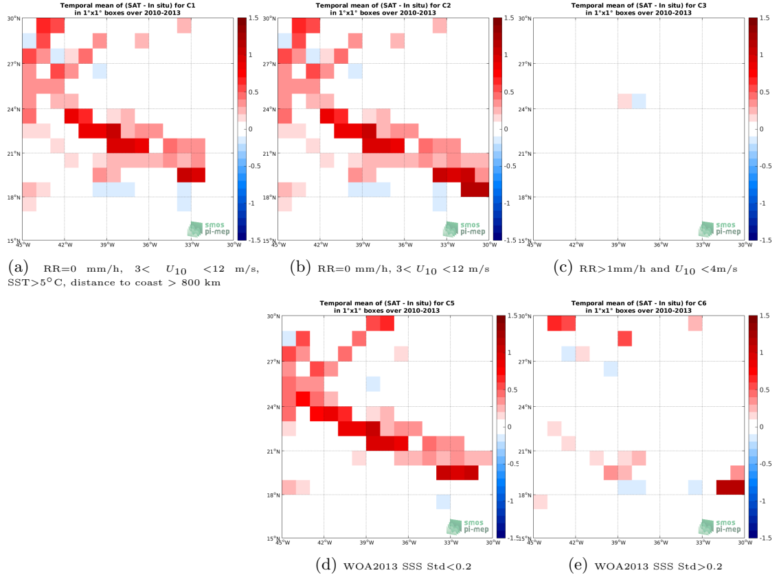
Figure 12: Temporal mean gridded over spatial boxes of size 1^\circ \times 1^\circ of \Delta SSS (SMOS-L3-BEC-OA-V1-9DAYS-0.25DEG - TSG-SAMOS) for 5 different subdatasets corresponding to: RR=0 mm/h, 3 < U_{10} < 12 m/s, SST > 5^\circ\text{C} , distance to coast > 800 km (a), RR=0 mm/h, 3 < U_{10} < 12 m/s (b), RR > 1 mm/h and U_{10} < 4 m/s (c), WOA2013 SSS Std < 0.2 (d), WOA2013 SSS Std > 0.2 (e).
