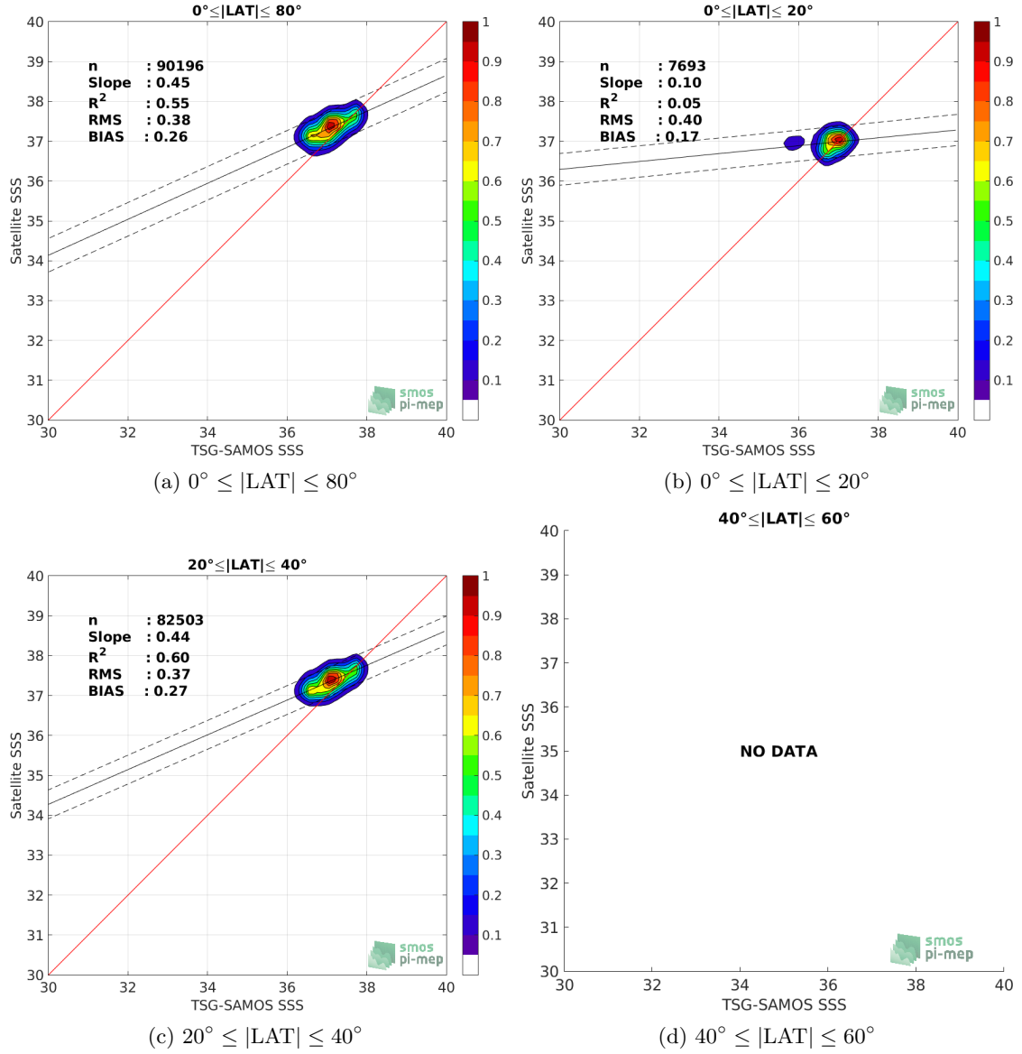
Figure 9: Contour maps of the concentration of SMOS-L3-BEC-OA-V1-9DAYS-0.25DEG SSS (y-axis) versus TSG-SAMOS SSS (x-axis) at match-up pairs for different latitude bands. For each plot, the red line shows x=y . The black thin and dashed lines indicate a linear fit through the data cloud and the \pm 95\% confidence levels, respectively. The number match-up pairs n , the slope and R^2 coefficient of the linear fit, the root mean square (RMS) and the mean bias between satellite and in situ data are indicated for each latitude band in each plots.
