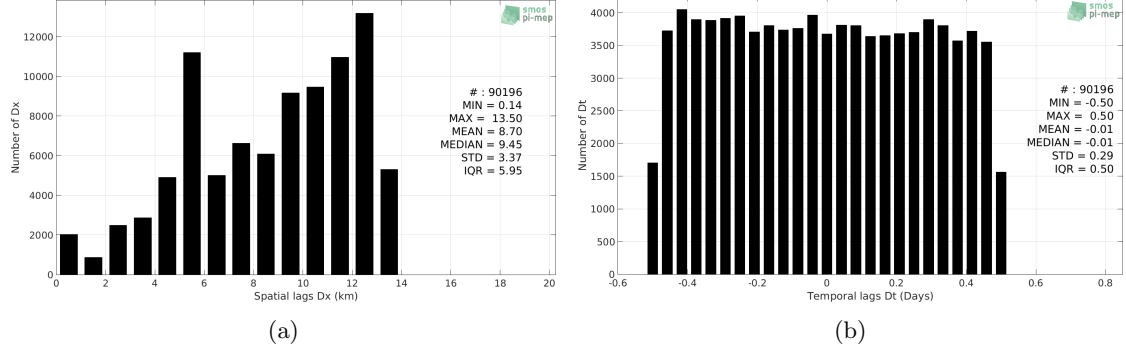
Figure 5: Histograms of the spatial (a) and temporal (b) lags between the time of the TSG-SAMOS measurements and the date of the corresponding SMOS-L3-BEC-OA-V1-9DAYS-0.25DEG SSS product.
