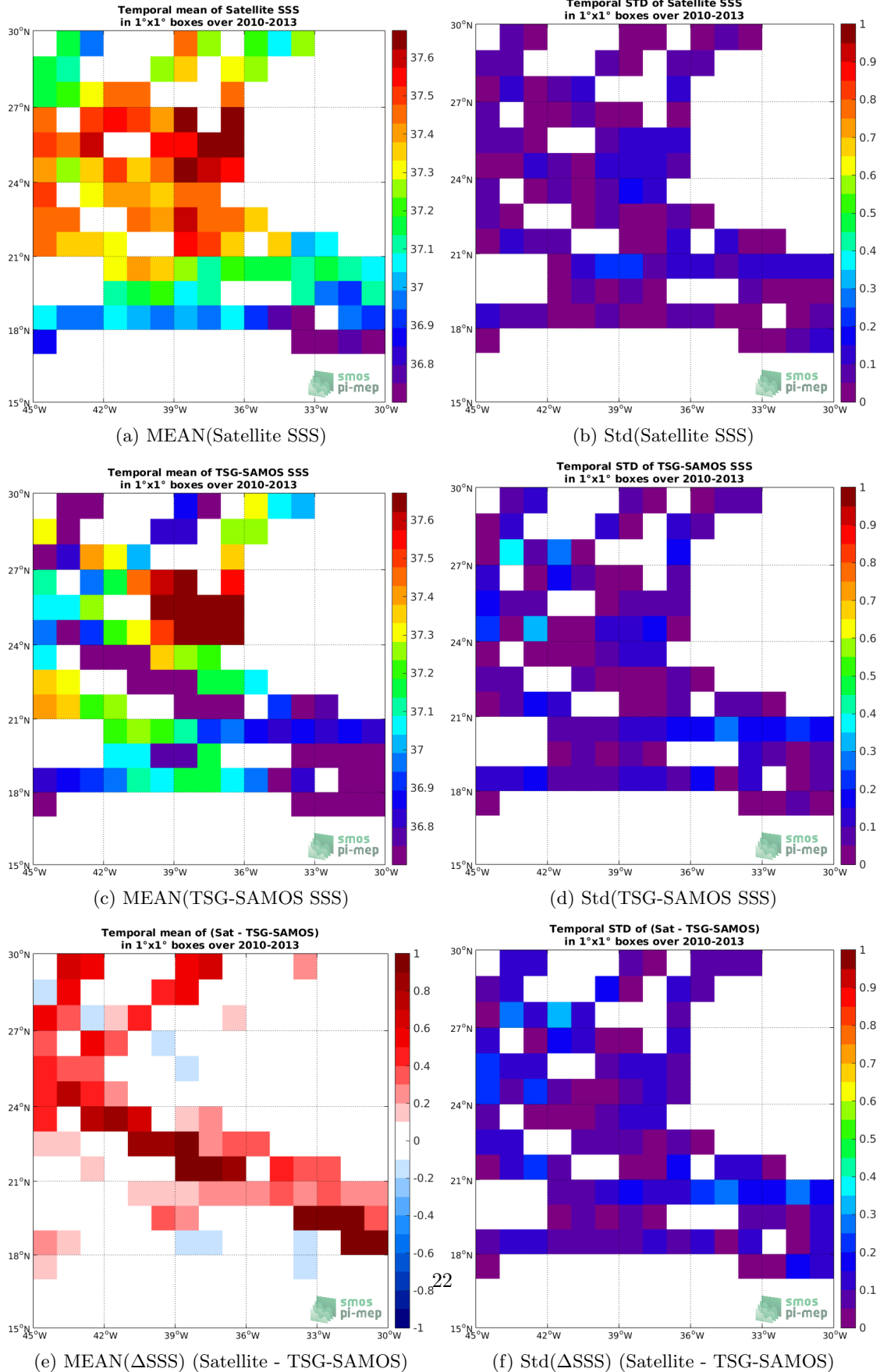
Figure 6: Temporal mean (left) and Std (right) of SSS from SMOS-L3-BEC-OA-V1-9DAYS-0.25DEG (top), TSG-SAMOS (middle), and of \Delta SSS (Satellite - TSG-SAMOS). Only match-up pairs are used to generate these maps.
