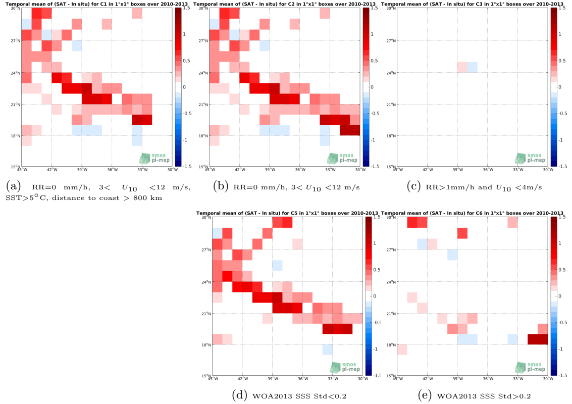
Figure 12: Temporal mean gridded over spatial boxes of size 1^\circ \times 1^\circ of \Delta SSS (SMOS-L3-BEC-OA-V1-9DAYS-0.25DEG - TSG-SAMOS) for 5 different subdatasets corresponding to: RR=0 mm/h, 3 < U_{10} < 12 m/s, SST > 5^\circ C , distance to coast > 800 km (a), RR=0 mm/h, 3 < U_{10} < 12 m/s (b), RR > 1 mm/h and U_{10} < 4 m/s (c), WOA2013 SSS Std < 0.2 (d), WOA2013 SSS Std > 0.2 (e).
