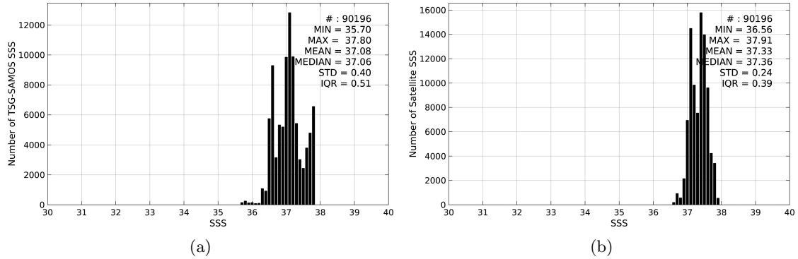
Figure 2: Histograms of SSS from TSG-SAMOS (a) and SMOS-L3-BEC-OA-V1-9DAYS-0.25DEG (b) considering all match-up pairs per bins of 0.1 over the SPURS 1 Pi-MEP region and for the full satellite product period.
