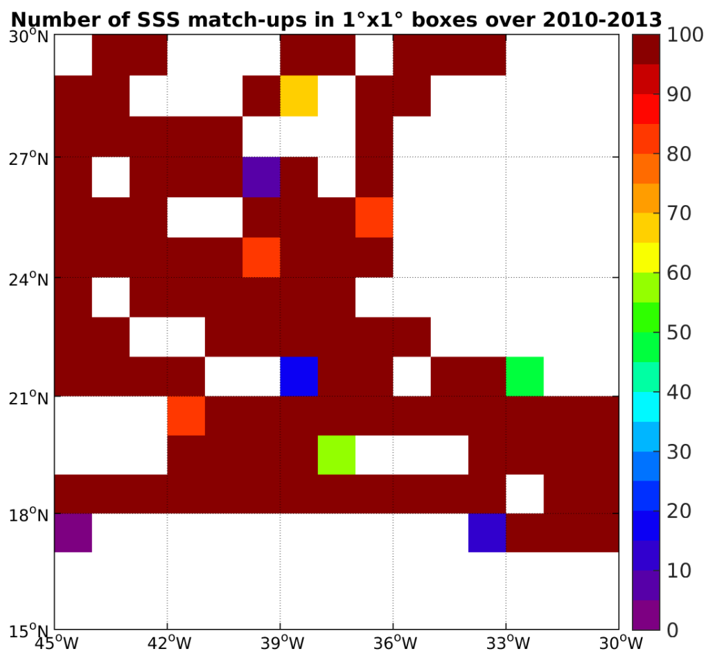
Figure 4: Number of SSS match-ups between TSG-SAMOS SSS and the SMOS-L3-BEC-OA-V1-9DAYS-0.25DEG SSS product for the SPURS 1 Pi-MEP region over 1°x1° boxes and for the full satellite product period.
