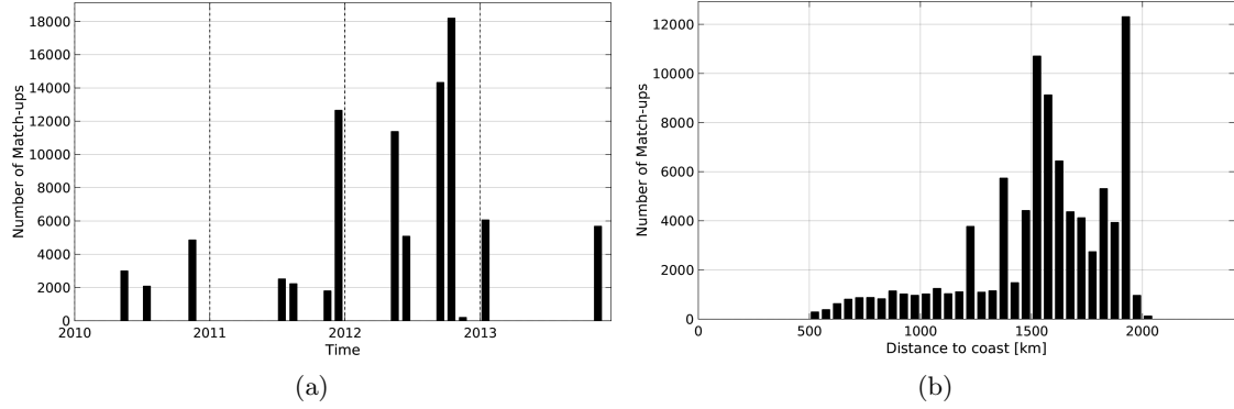
Figure 1: Number of match-ups between TSG-SAMOS and SMOS-L3-BEC-OA-V1-9DAYS-0.25DEG SSS as a function of time (a) and as function of the distance to coast (b) over the SPURS 1 Pi-MEP region and for the full satellite product period.
