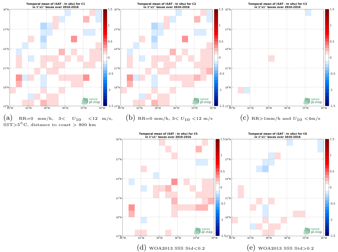
Figure 12: Temporal mean gridded over spatial boxes of size 1^\circ \times 1^\circ of \Delta SSS (SMOS-L3-BEC-OA-V1-9DAYS-0.25DEG - TSG-LEGOS-DM) for 5 different subdatasets corresponding to: RR=0 mm/h, 3 < U_{10} < 12 m/s, SST > 5^\circ\text{C} , distance to coast > 800 km (a), RR=0 mm/h, 3 < U_{10} < 12 m/s (b), RR > 1\text{mm/h} and U_{10} < 4\text{m/s} (c), WOA2013 SSS Std < 0.2 (d), WOA2013 SSS Std > 0.2 (e).
