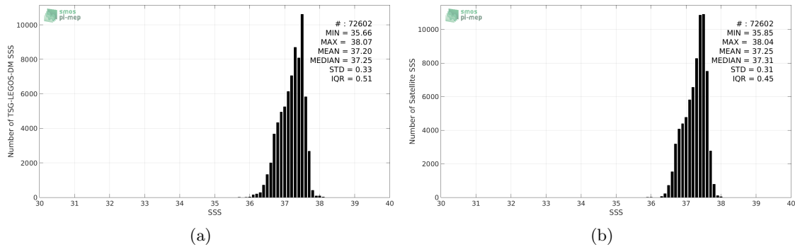
Figure 2: Histograms of SSS from TSG-LEGOS-DM (a) and SMOS-L3-BEC-OA-V1-9DAYS-0.25DEG (b) considering all match-up pairs per bins of 0.1 over the SPURS 1 Pi-MEP region and for the full satellite product period.
