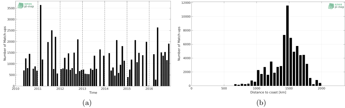
Figure 1: Number of match-ups between TSG-LEGOS-DM and SMOS-L3-BEC-OA-V1-9DAYS-0.25DEG SSS as a function of time (a) and as function of the distance to coast (b) over the SPURS 1 Pi-MEP region and for the full satellite product period.
