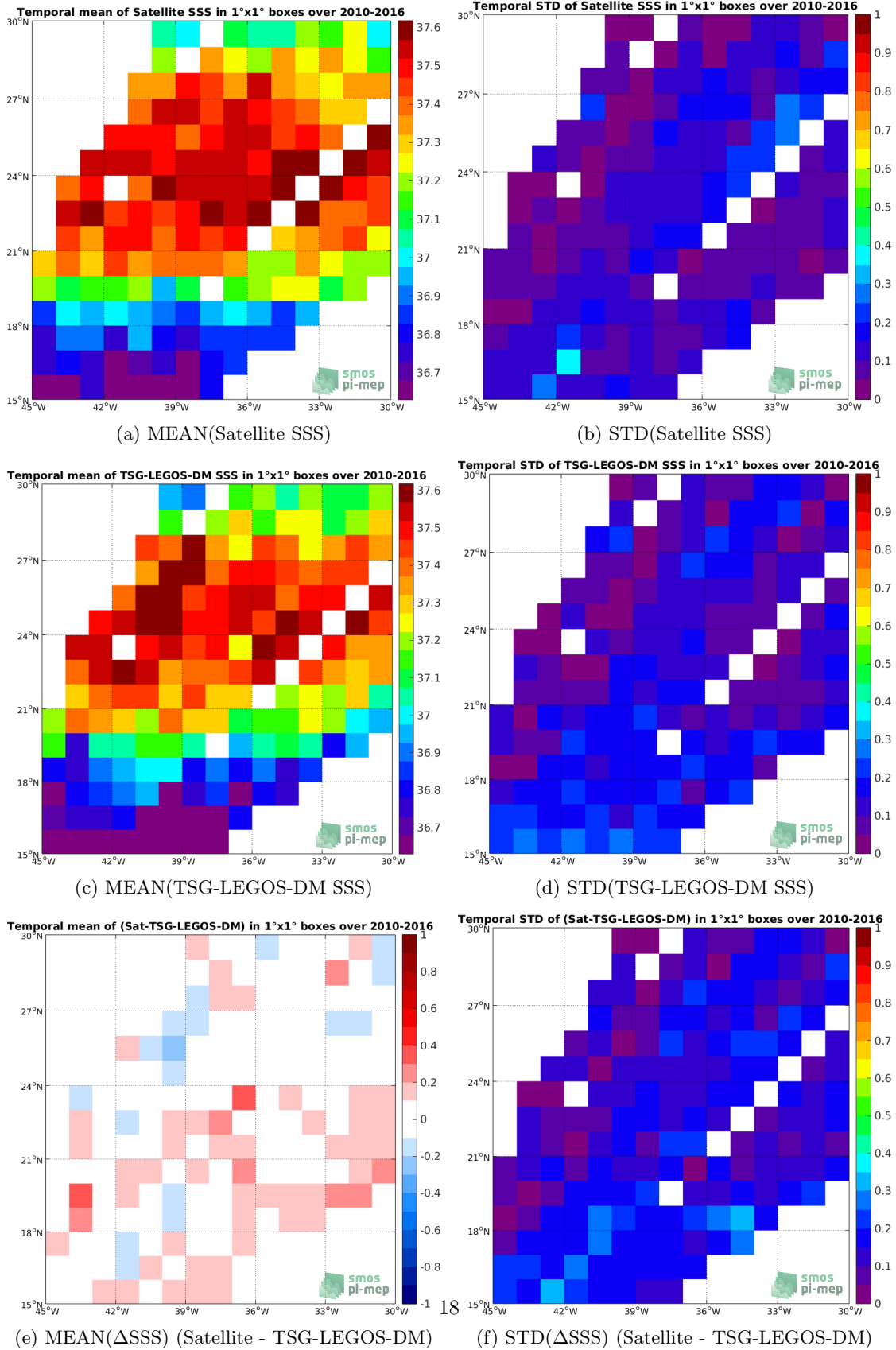
Figure 6: Temporal mean (left) and STD (right) of SSS from SMOS-L3-BEC-OA-V1-9DAYS-0.25DEG (top), TSG-LEGOS-DM (middle), and of \Delta SSS (Satellite - TSG-LEGOS-DM). Only match-up pairs are used to generate these maps.
