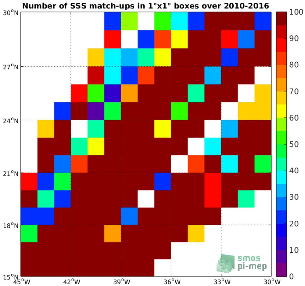
Figure 4: Number of SSS match-ups between TSG-LEGOS-DM SSS and the SMOS-L3-BEC-OA-V1-9DAYS-0.25DEG SSS product for the SPURS 1 Pi-MEP region over 1°x1° boxes and for the full satellite product period.
