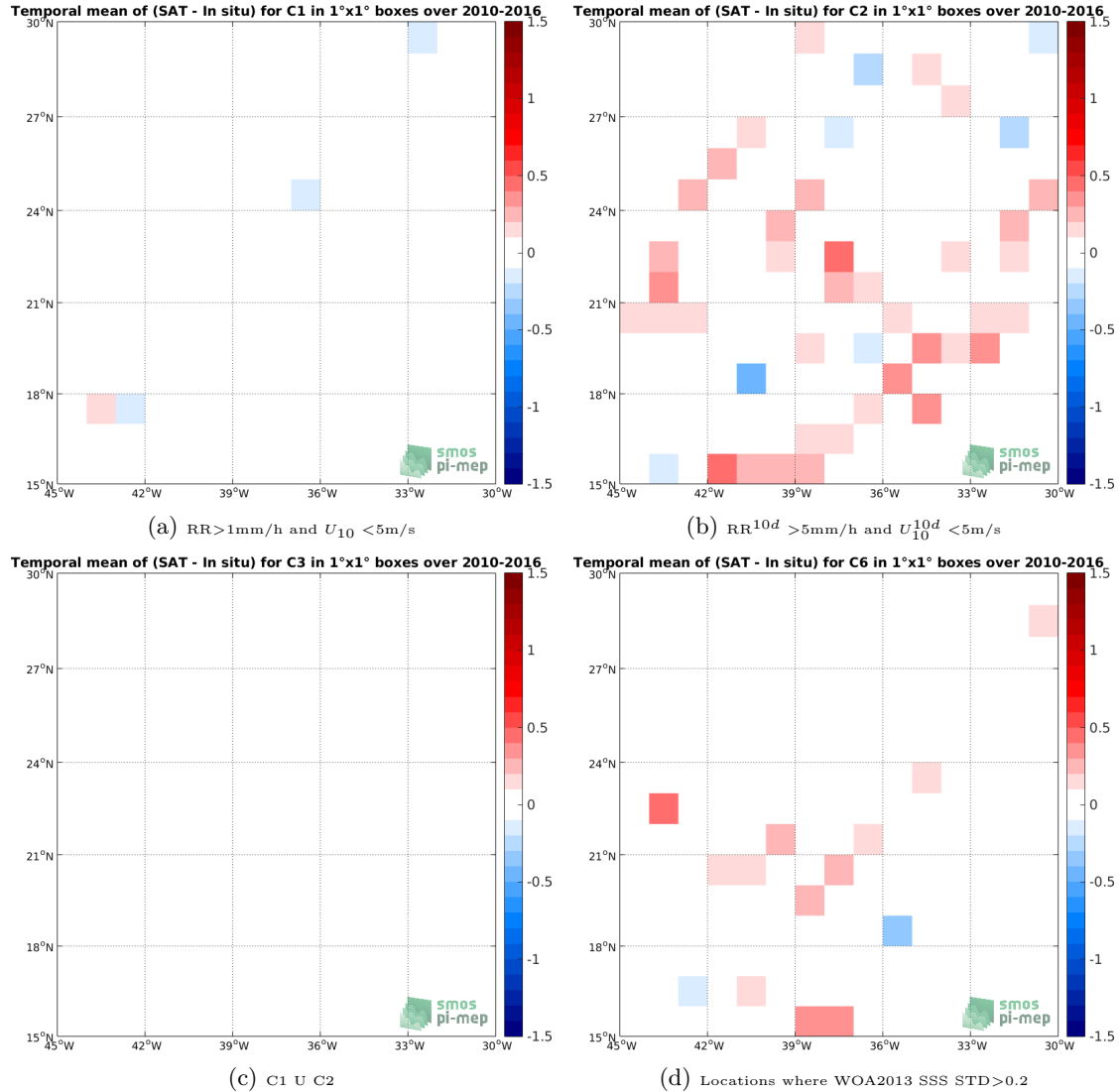
Figure 12: Temporal mean gridded over spatial boxes of size 1^\circ \times 1^\circ of \Delta SSS (SMOS-L3-BEC-OA-V1-9DAYS-0.25DEG - TSG-LEGOS-DM) for 4 different subdatasets corresponding to: RR > 1\text{mm/h} and U_{10} < 5\text{m/s} (a), RR^{10d} > 5\text{mm/h} and U_{10}^{10d} < 5\text{m/s} (b), C1 U C2 (c), Locations where WOA2013 SSS STD > 0.2 (d).
