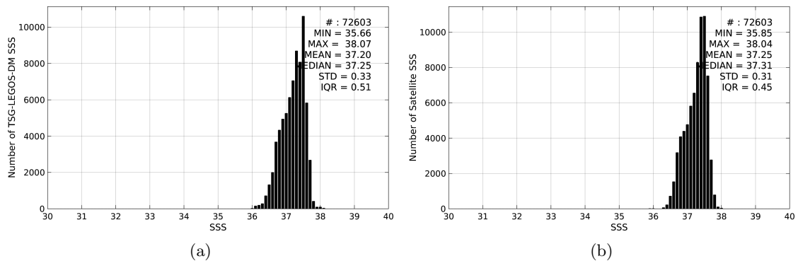
Figure 2: Histograms of SSS from TSG-LEGOS-DM (a) and SMOS-L3-BEC-OA-V1-9DAYS-0.25DEG (b) considering all match-up pairs per bins of 0.1 over the SPURS 1 Pi-MEP region and for the full satellite product period.
