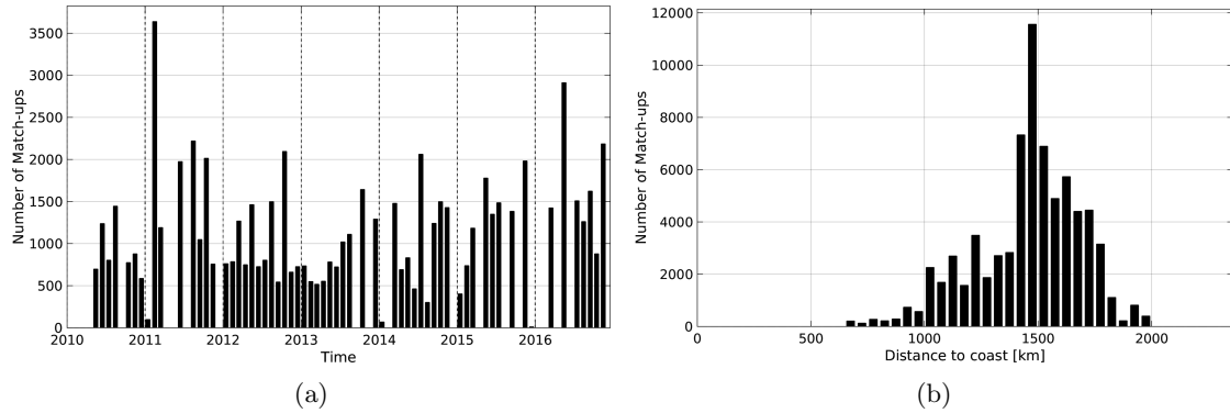
Figure 1: Number of match-ups between TSG-LEGOS-DM and SMOS-L3-BEC-OA-V1-9DAYS-0.25DEG SSS as a function of time (a) and as function of the distance to coast (b) over the SPURS 1 Pi-MEP region and for the full satellite product period.
