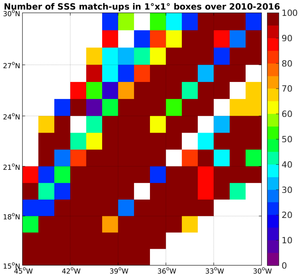
Figure 4: Number of SSS match-ups between TSG-LEGOS-DM SSS and the SMOS-L3-BEC-OA-V1-9DAYS-0.25DEG SSS product for the SPURS 1 Pi-MEP region over 1°x1° boxes and for the full satellite product period.
