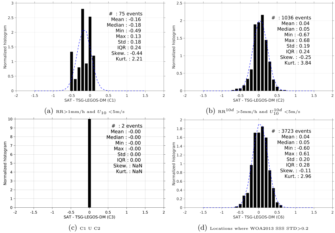
Figure 13: Normalized histogram of \Delta SSS (SMOS-L3-BEC-OA-V1-9DAYS-0.25DEG - TSG-LEGOS-DM) for 6 different subdatasets corresponding to: RR > 1mm/h and U_{10} < 5 m/s (a), RR^{10d} > 5 mm/h and U_{10}^{10d} < 5 m/s (b), C1 U C2 (c), Locations where WOA2013 SSS STD > 0.2 (d).
