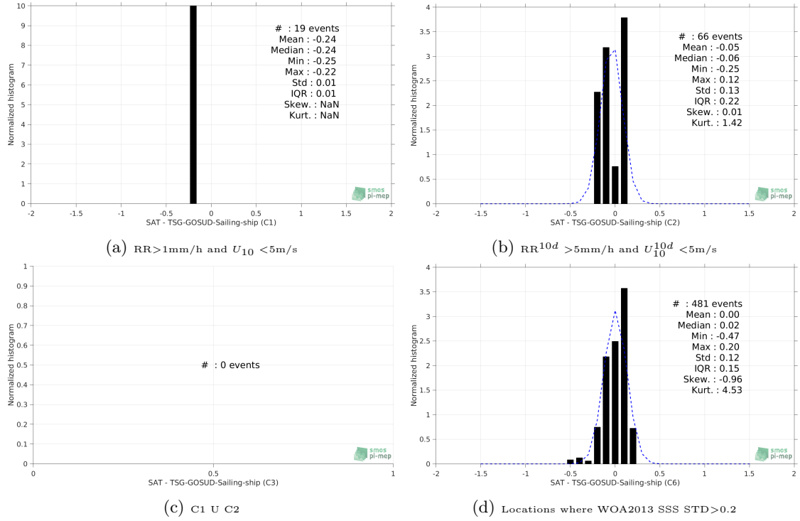
Figure 13: Normalized histogram of \Delta\text{SSS} (SMOS-L3-BEC-OA-V1-9DAYS-0.25DEG - TSG-GOSUD-Sailing-ship) for 6 different subdatasets corresponding to: RR > 1\text{mm/h} and U_{10} < 5\text{m/s} (a), RR^{10d} > 5\text{mm/h} and U_{10}^{10d} < 5\text{m/s} (b), C1 U C2 (c), Locations where WOA2013 SSS STD > 0.2 (d).
