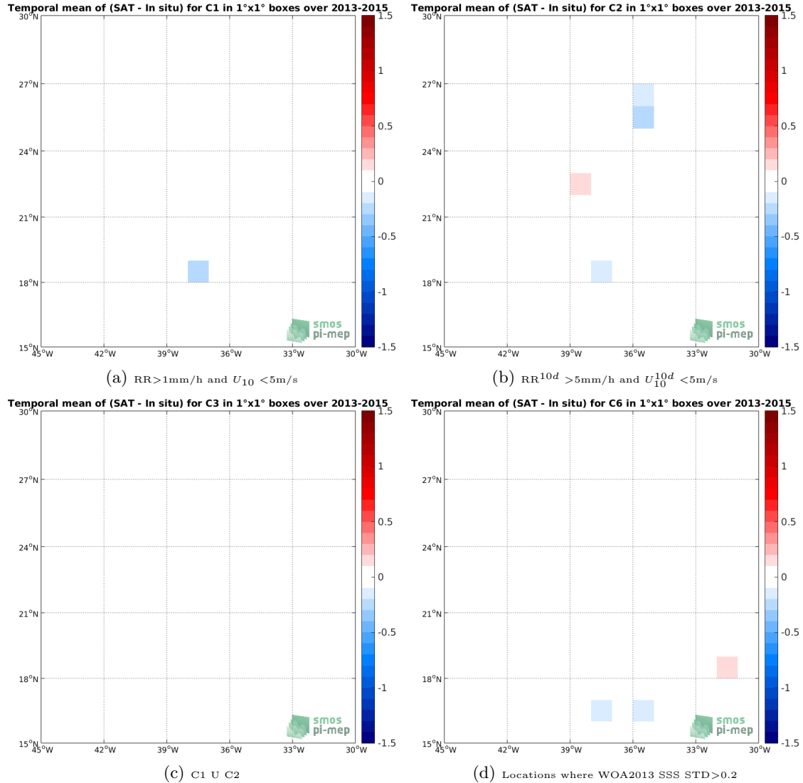
Figure 12: Temporal mean gridded over spatial boxes of size 1^\circ \times 1^\circ of \Delta SSS (SMOS-L3-BEC-OA-V1-9DAYS-0.25DEG - TSG-GOSUD-Sailing-ship) for 4 different subdatasets corresponding to: RR > 1\text{mm/h} and U_{10} < 5\text{m/s} (a), RR^{10d} > 5\text{mm/h} and U_{10}^{10d} < 5\text{m/s} (b), C1 U C2 (c), Locations where WOA2013 SSS STD > 0.2 (d).
