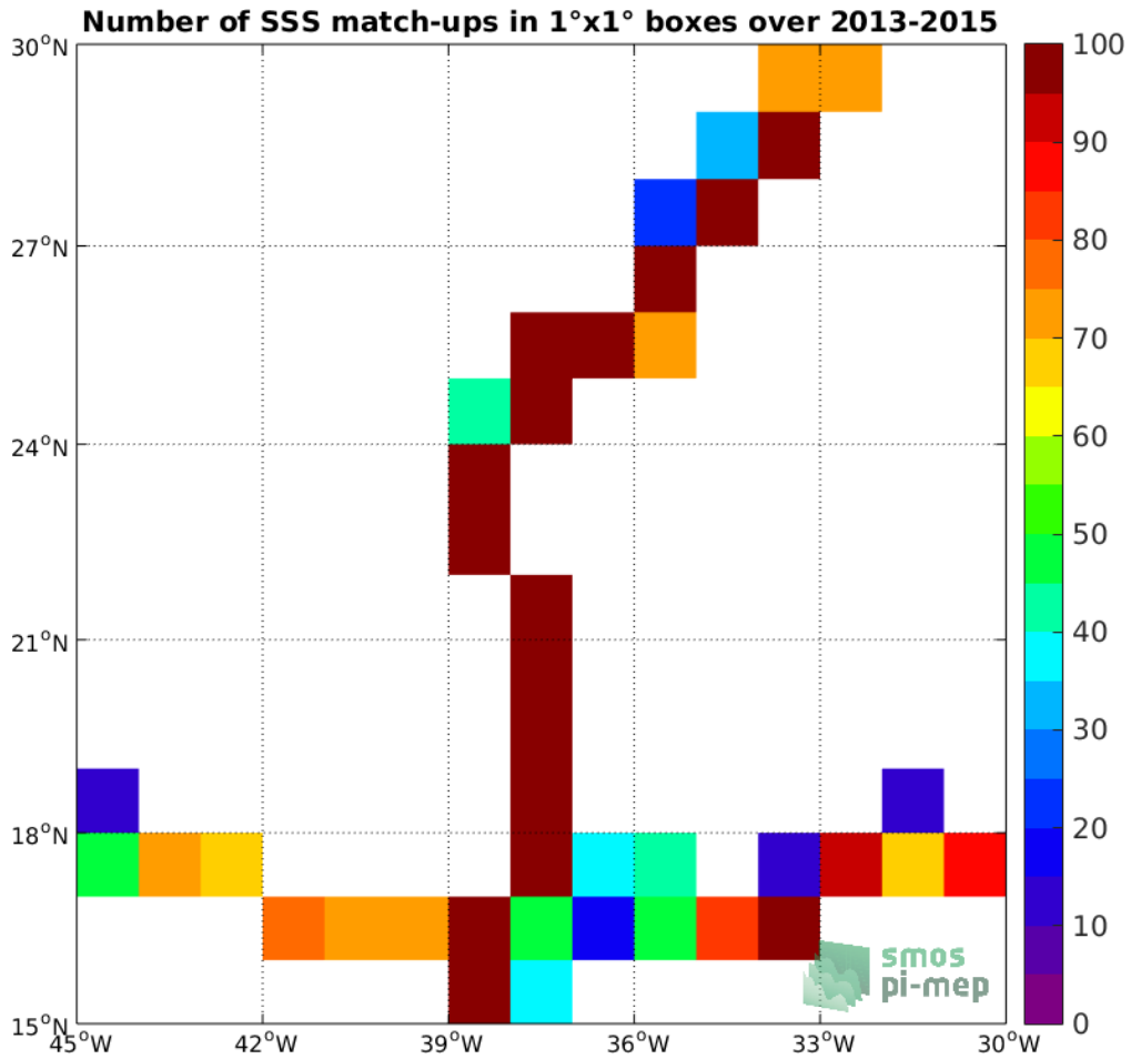
Figure 4: Number of SSS match-ups between TSG-GOSUD-Sailing-ship SSS and the SMOS-L3-BEC-OA-V1-9DAYS-0.25DEG SSS product for the SPURS 1 Pi-MEP region over 1°x1° boxes and for the full satellite product period.
