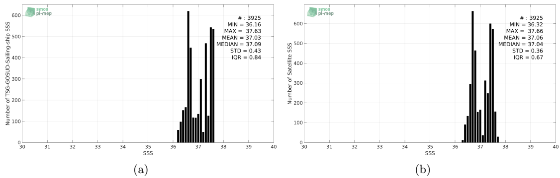
Figure 2: Histograms of SSS from TSG-GOSUD-Sailing-ship (a) and SMOS-L3-BEC-OA-V1-9DAYS-0.25DEG (b) considering all match-up pairs per bins of 0.1 over the SPURS 1 Pi-MEP region and for the full satellite product period.
