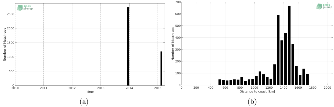
Figure 1: Number of match-ups between TSG-GOSUD-Sailing-ship and SMOS-L3-BEC-OA-V1-9DAYS-0.25DEG SSS as a function of time (a) and as function of the distance to coast (b) over the SPURS 1 Pi-MEP region and for the full satellite product period.
