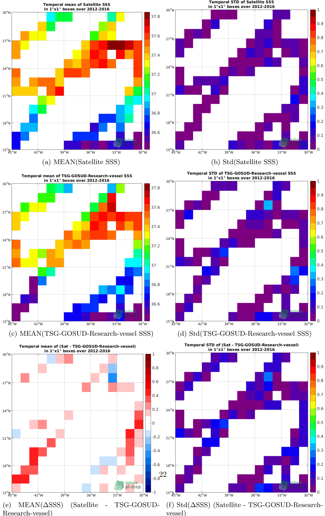
Figure 6: Temporal mean (left) and Std (right) of SSS from SMOS-L3-BEC-OA-V1-9DAYS-0.25DEG (top), TSG-GOSUD-Research-vessel (middle), and of \Delta SSS (Satellite - TSG-GOSUD-Research-vessel). Only match-up pairs are used to generate these maps.
