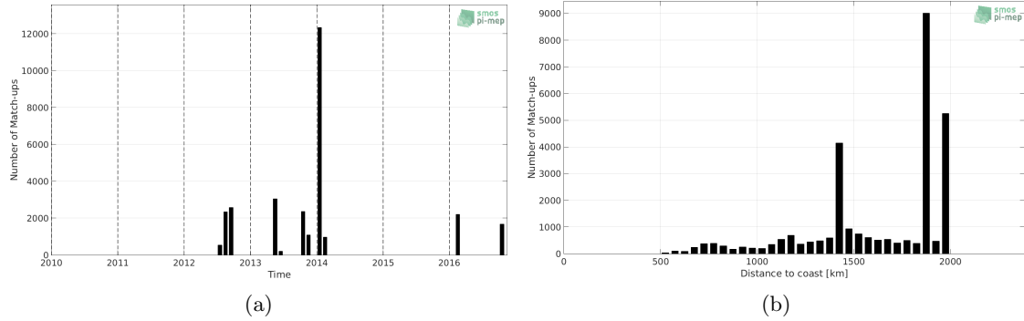
Figure 1: Number of match-ups between TSG-GOSUD-Research-vessel and SMOS-L3-BEC-OA-V1-9DAYS-0.25DEG SSS as a function of time (a) and as function of the distance to coast (b) over the SPURS 1 Pi-MEP region and for the full satellite product period.
