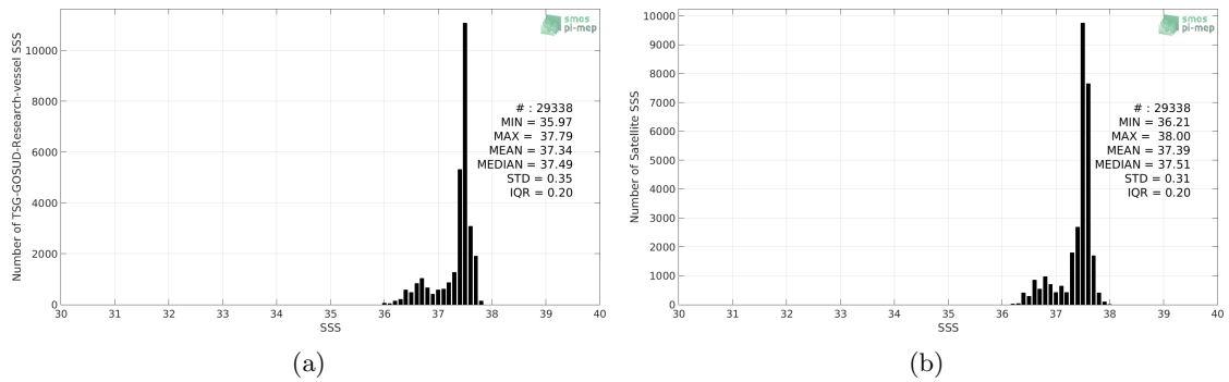
Figure 2: Histograms of SSS from TSG-GOSUD-Research-vessel (a) and SMOS-L3-BEC-OA-V1-9DAYS-0.25DEG (b) considering all match-up pairs per bins of 0.1 over the SPURS 1 Pi-MEP region and for the full satellite product period.
