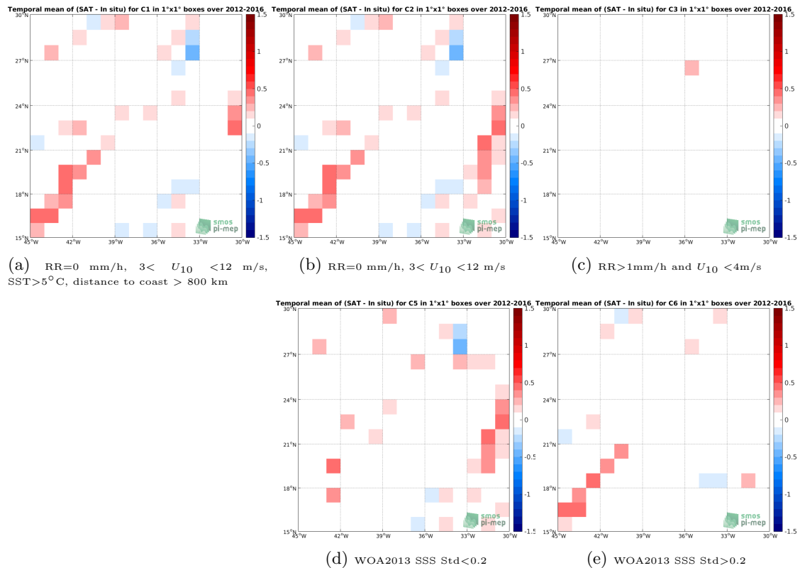
Figure 12: Temporal mean gridded over spatial boxes of size 1^\circ \times 1^\circ of \Delta SSS (SMOS-L3-BEC-OA-V1-9DAYS-0.25DEG - TSG-GOSUD-Research-vessel) for 5 different subdatasets corresponding to:RR=0 mm/h, 3 < U_{10} < 12 m/s, SST >5^\circ\text{C} , distance to coast > 800 km (a), RR=0 mm/h, 3 < U_{10} < 12 m/s (b), RR >1 mm/h and U_{10} < 4 m/s (c), WOA2013 SSS Std <0.2 (d), WOA2013 SSS Std >0.2 (e).
