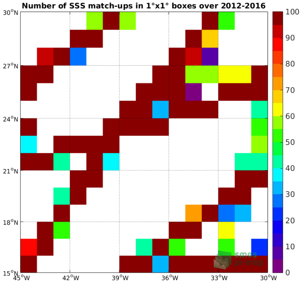
Figure 4: Number of SSS match-ups between TSG-GOSUD-Research-vessel SSS and the SMOS-L3-BEC-OA-V1-9DAYS-0.25DEG SSS product for the SPURS 1 Pi-MEP region over 1°x1° boxes and for the full satellite product period.
