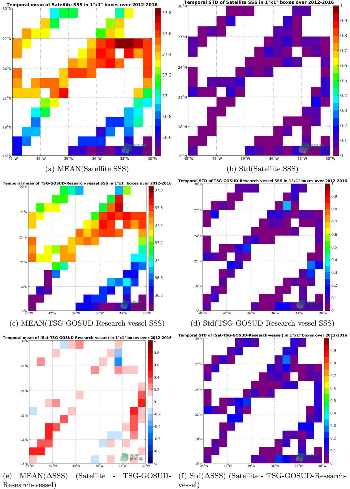
Figure 6: Temporal mean (left) and Std (right) of SSS from SMOS-L3-BEC-OA-V1-9DAYS-0.25DEG (top), TSG-GOSUD-Research-vessel (middle), and of \Delta SSS (Satellite - TSG-GOSUD-Research-vessel). Only match-up pairs are used to generate these maps.
