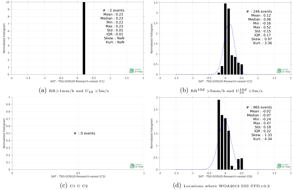
Figure 13: Normalized histogram of \Delta\text{SSS} (SMOS-L3-BEC-OA-V1-9DAYS-0.25DEG - TSG-GOSUD-Research-vessel) for 6 different subdatasets corresponding to: RR > 1mm/h and U_{10} < 5\text{m/s} (a), RR^{10d} > 5\text{mm/h} and U_{10}^{10d} < 5\text{m/s} (b), C1 U C2 (c), Locations where WOA2013 SSS STD > 0.2 (d).
