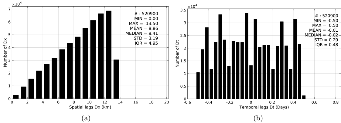
Figure 4: Histograms of the spatial (a) and temporal (b) lags between the time of the Surface drifters measurements and the date of the corresponding SMOS-L3-BEC-OA-V1-9DAYS-0.25DEG SSS product.
