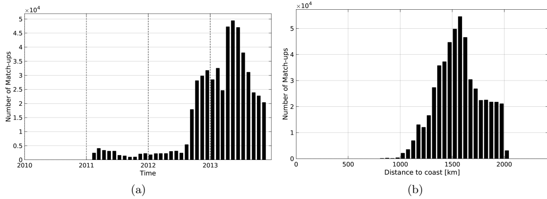
Figure 1: Number of match-ups between Surface drifters and SMOS-L3-BEC-OA-V1-9DAYS-0.25DEG SSS as a function of time (a) and as function of the distance to coast (b) over the SPURS 1 Pi-MEP region and for the full satellite product period.
