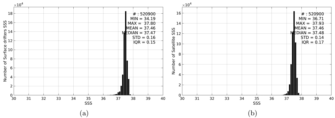
Figure 2: Histograms of SSS from Surface drifters (a) and SMOS-L3-BEC-OA-V1-9DAYS-0.25DEG (b) considering all match-up pairs per bins of 0.1 over the SPURS 1 Pi-MEP region and for the full satellite product period.
