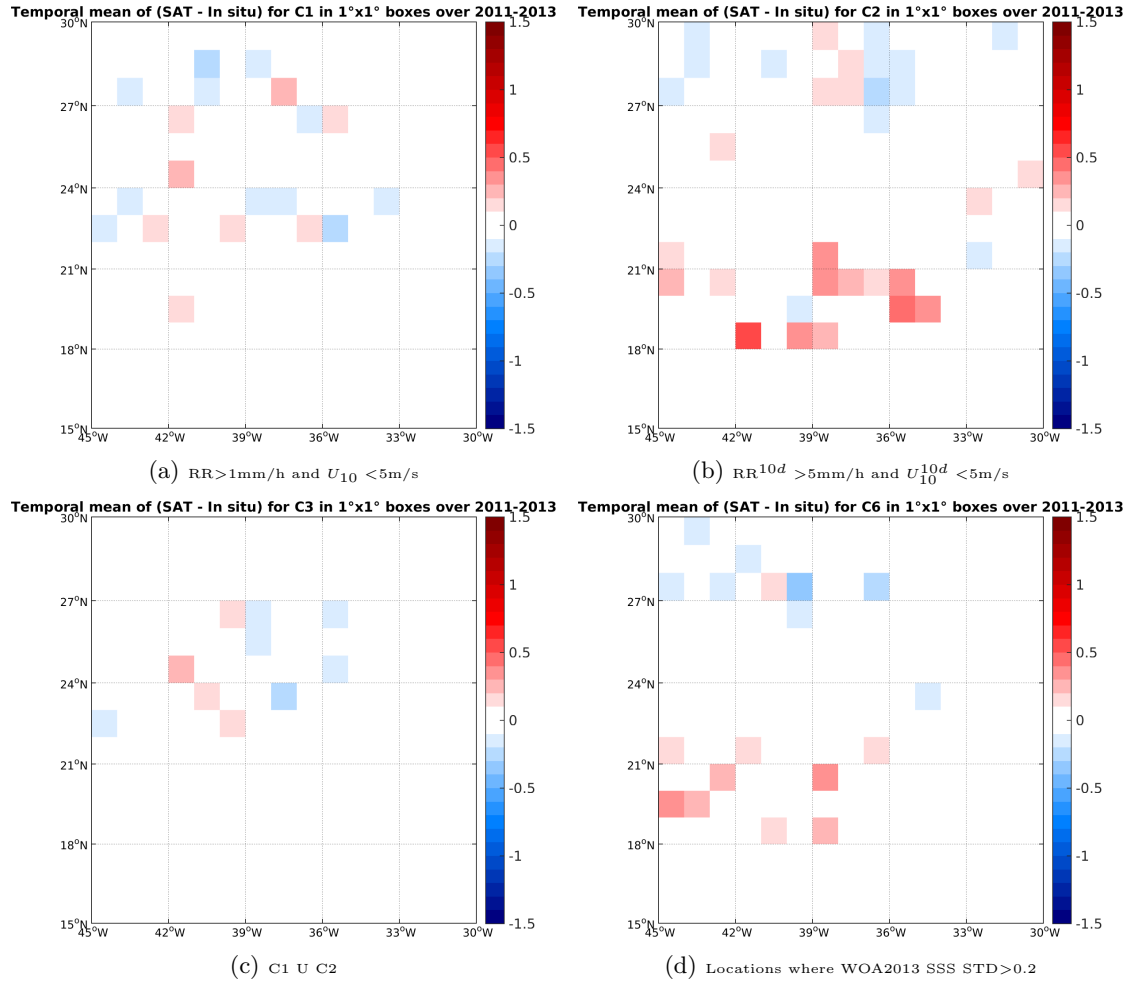
Figure 11: Temporal mean gridded over spatial boxes of size 1°x1° of \Delta SSS (SMOS-L3-BEC-OA-V1-9DAYS-0.25DEG - Surface drifters) for 4 different subdatasets corresponding to:RR>1mm/h and U_{10} < 5\text{m/s} (a), RR^{10d} > 5\text{mm/h} and U_{10}^{10d} < 5\text{m/s} (b), C1 U C2 (c),Locations where WOA2013 SSS STD>0.2 (d).
