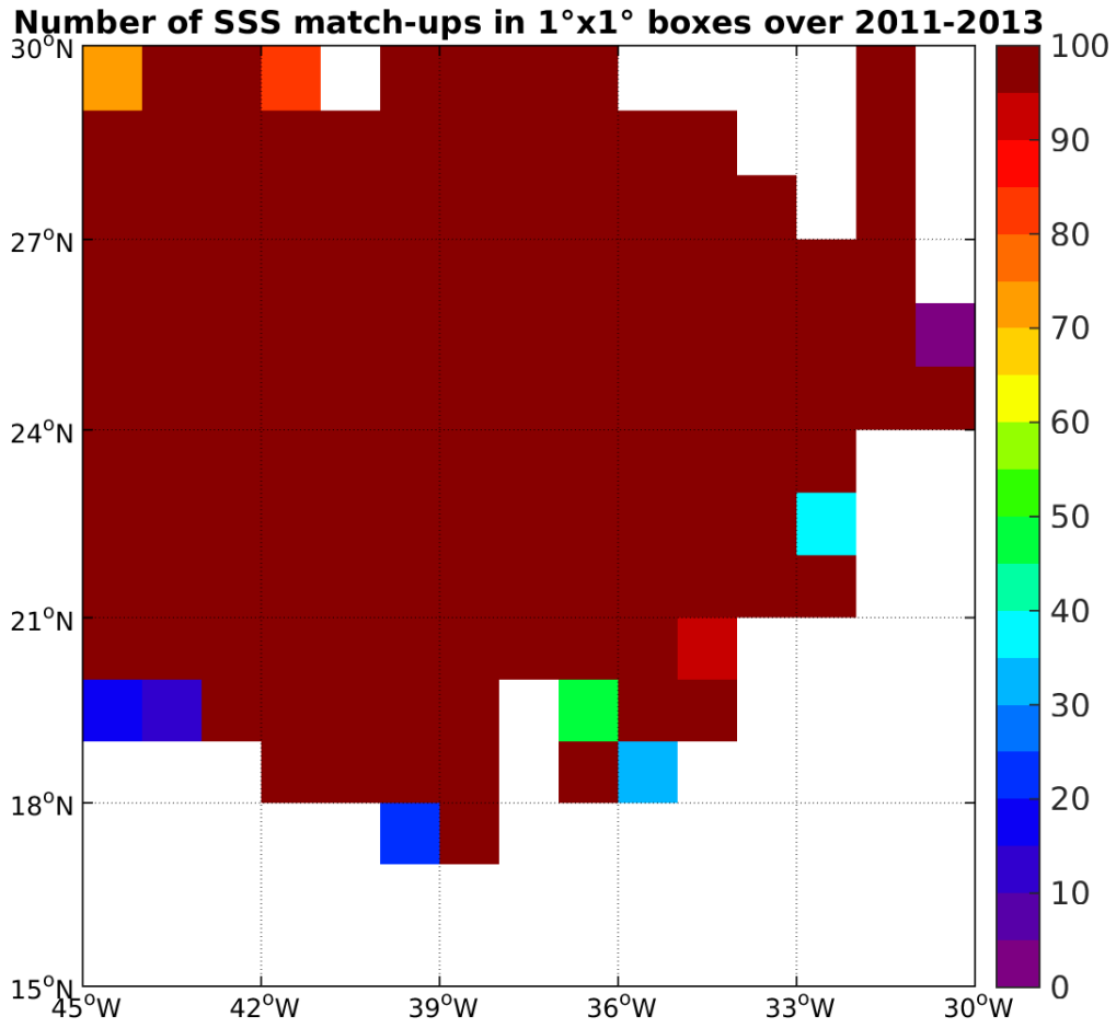
Figure 3: Number of SSS match-ups between Surface drifters SSS and the SMOS-L3-BEC-OA-V1-9DAYS-0.25DEG SSS product for the SPURS 1 Pi-MEP region over 1°x1° boxes and for the full satellite product period.
