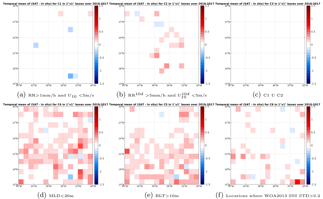
Figure 12: Temporal mean gridded over spatial boxes of size 1^\circ \times 1^\circ of \Delta SSS (SMOS-L3-BEC-OA-V1-9DAYS-0.25DEG - Argo) for 6 different subdatasets corresponding to: RR > 1\text{mm/h} and U_{10} < 5\text{m/s} (a), RR^{10d} > 5\text{mm/h} and U_{10}^{10d} < 5\text{m/s} (b), C1 U C2 (c), MLD < 20\text{m} (d), BLT > 10\text{m} (e), Locations where WOA2013 SSS STD > 0.2 (f).
