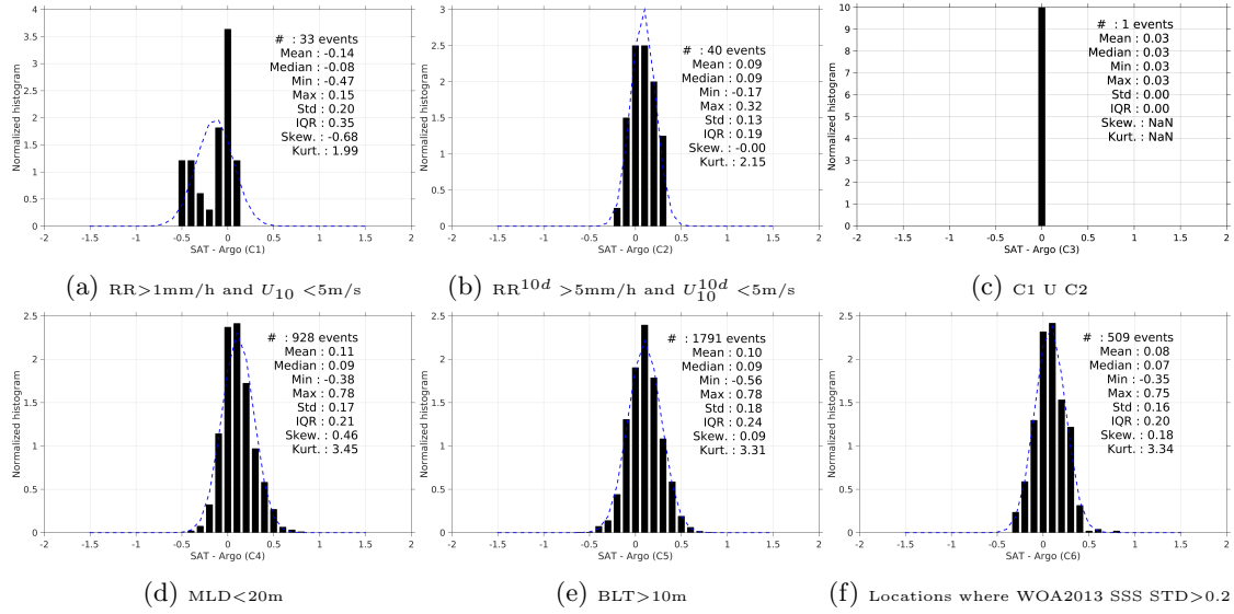
Figure 13: Normalized histogram of \Delta SSS (SMOS-L3-BEC-OA-V1-9DAYS-0.25DEG - Argo) for 6 different subdatasets corresponding to: RR>1mm/h and U_{10} < 5\text{m/s} (a), RR 10d >5mm/h and U_{10}^{10d} < 5\text{m/s} (b), C1 U C2 (c),MLD<20m (d),BLT>10m (e),Locations where WOA2013 SSS STD>0.2 (f).
