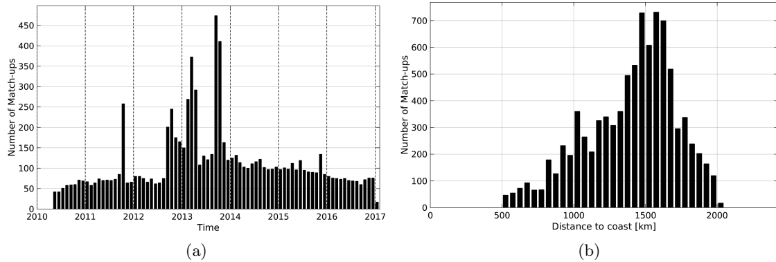
Figure 1: Number of match-ups between Argo and SMOS-L3-BEC-OA-V1-9DAYS-0.25DEG SSS as a function of time (a) and as function of the distance to coast (b) over the SPURS 1 Pi-MEP region and for the full satellite product period.
