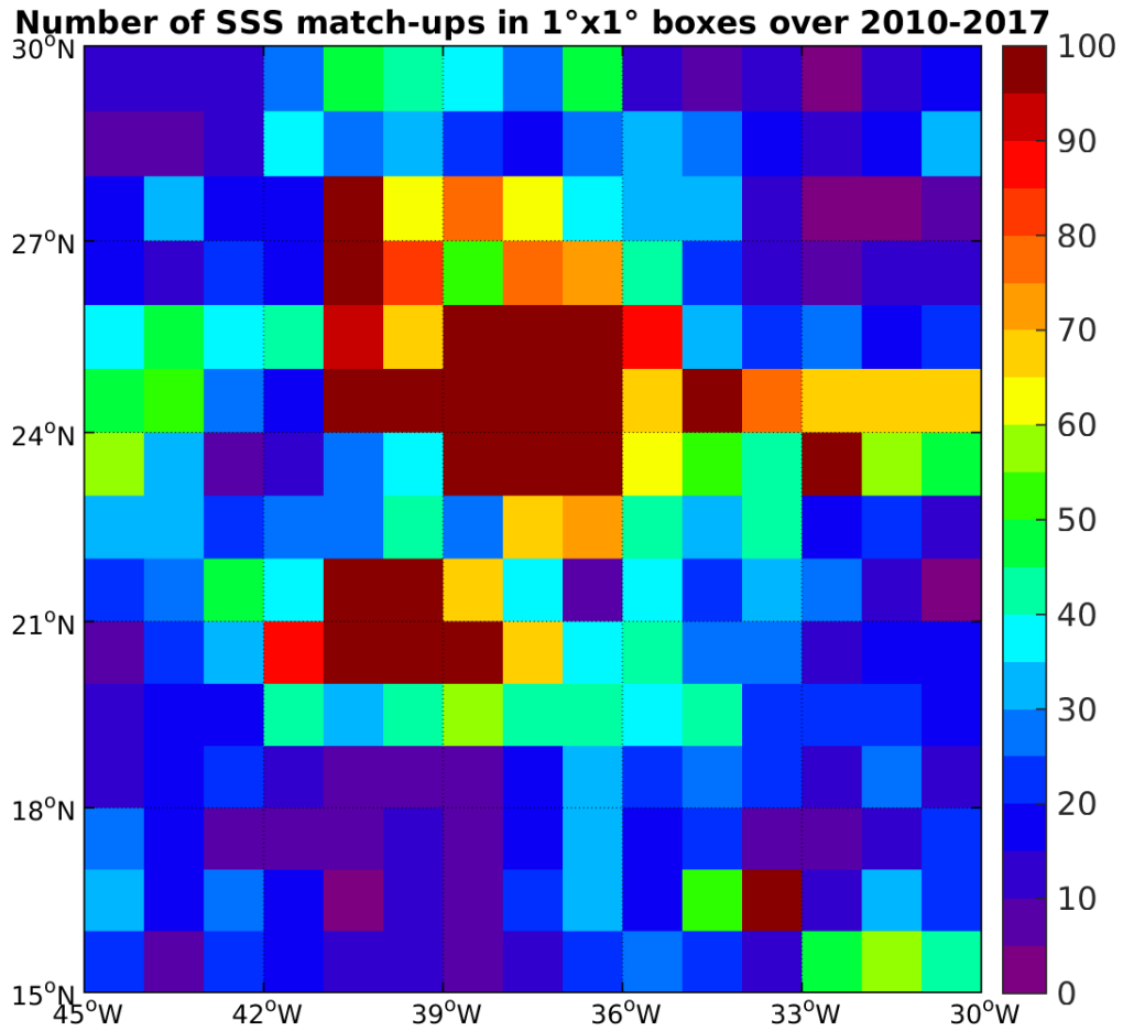
Figure 4: Number of SSS match-ups between Argo SSS and the SMOS-L3-BEC-OA-V1-9DAYS-0.25DEG SSS product for the SPURS 1 Pi-MEP region over 1°x1° boxes and for the full satellite product period.
