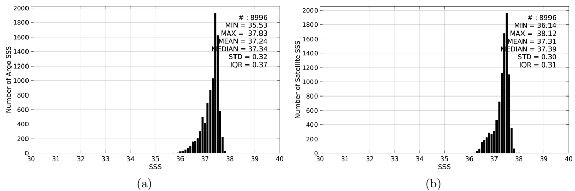
Figure 2: Histograms of SSS from Argo (a) and SMOS-L3-BEC-OA-V1-9DAYS-0.25DEG (b) considering all match-up pairs per bins of 0.1 over the SPURS 1 Pi-MEP region and for the full satellite product period.
