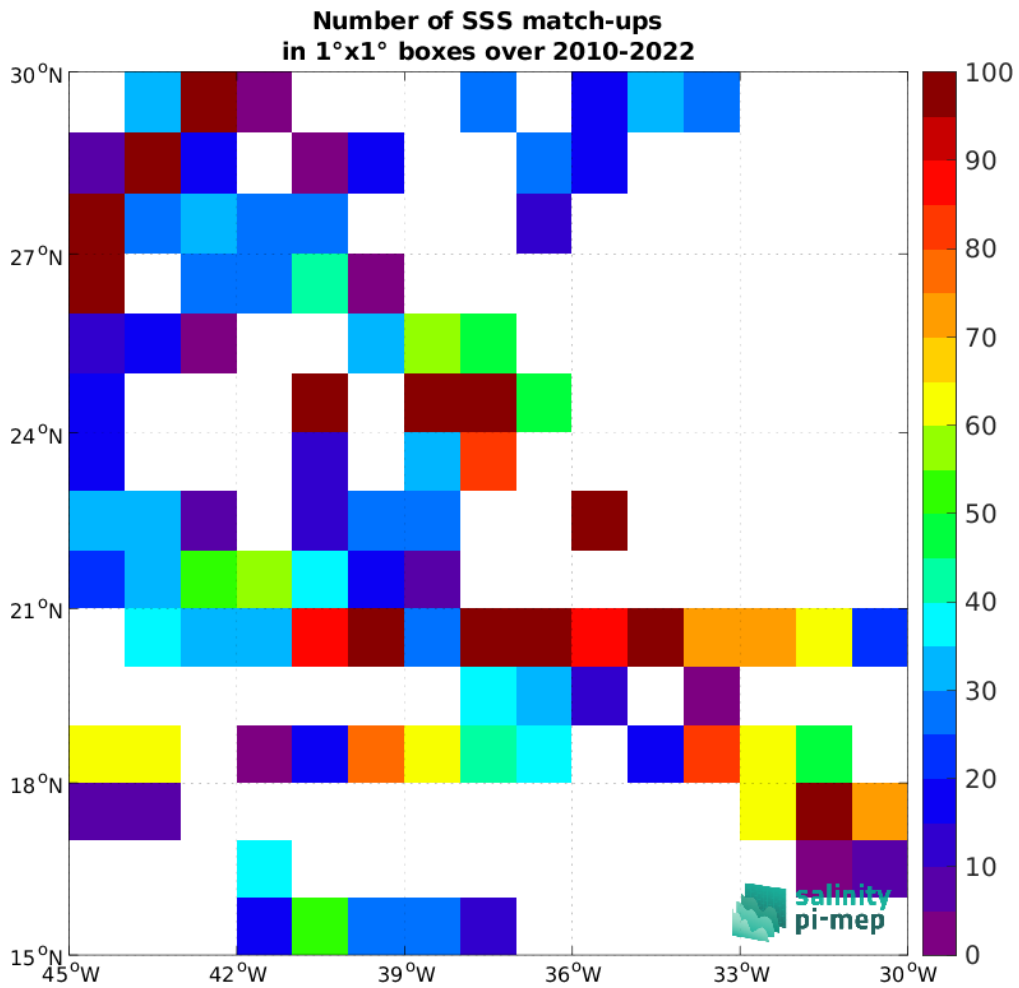
Figure 4: Number of SSS match-ups between TSG (SAMOS) SSS and the SMOS SSS L2 v700 (ESA) SSS product for the SPURS 1 Pi-MEP region over 1°x1° boxes and for the full satellite product period.
