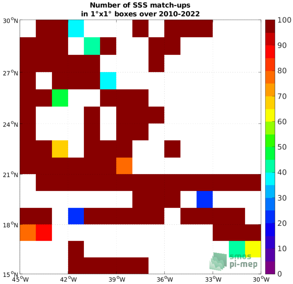
Figure 4: Number of SSS match-ups between TSG (SAMOS) SSS and the SMOS SSS L2 v700 (ESA) SSS product for the SPURS 1 Pi-MEP region over 1°×1° boxes and for the full satellite product period.
