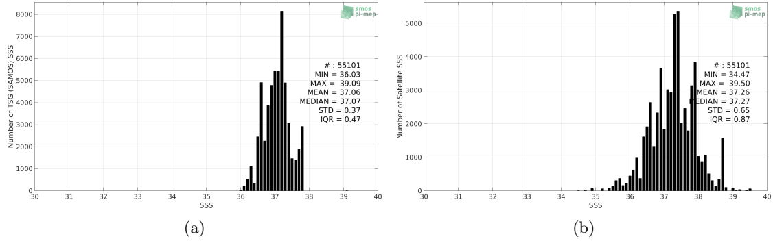
Figure 2: Histograms of SSS from TSG (SAMOS) (a) and SMOS SSS L2 v700 (ESA) (b) considering all match-up pairs per bins of 0.1 over the SPURS 1 Pi-MEP region and for the full satellite product period.
