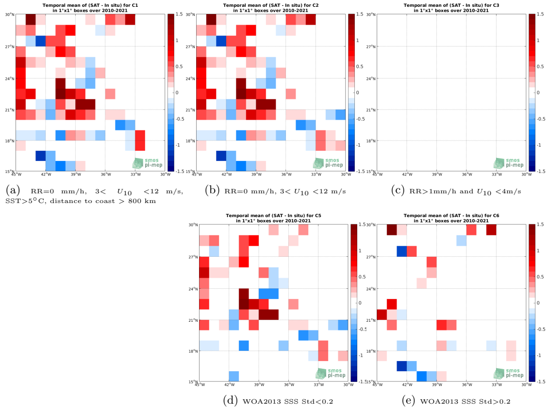
Figure 12: Temporal mean gridded over spatial boxes of size 1^\circ \times 1^\circ of \Delta SSS (SMOS SSS L2 v700 (ESA) - TSG (SAMOS)) for 5 different subdatasets corresponding to: RR=0 mm/h, 3 < U_{10} < 12 m/s, SST > 5^\circ C , distance to coast > 800 km (a), RR=0 mm/h, 3 < U_{10} < 12 m/s (b), RR > 1 mm/h and U_{10} < 4 m/s (c), WOA2013 SSS Std < 0.2 (d), WOA2013 SSS Std > 0.2 (e).
