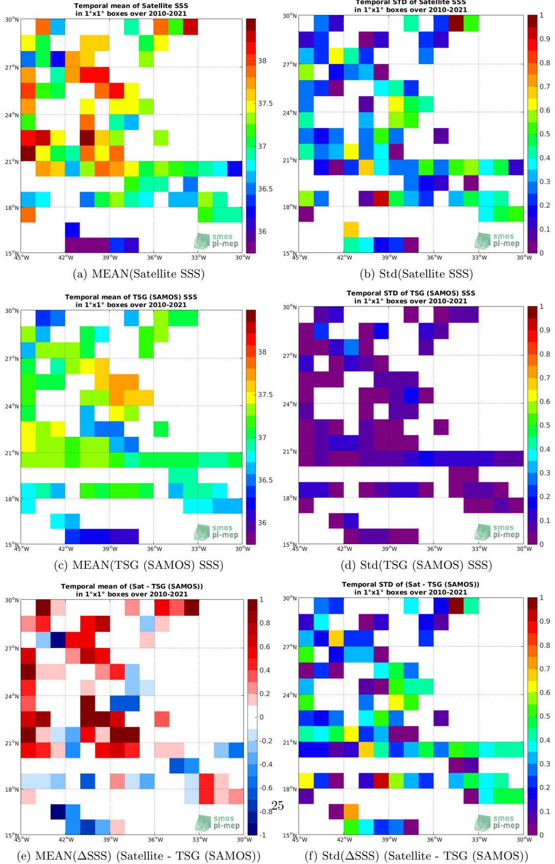
Figure 6: Temporal mean (left) and Std (right) of SSS from SMOS SSS L2 v700 (ESA) (top), TSG (SAMOS) (middle), and of \Delta SSS (Satellite - TSG (SAMOS)). Only match-up pairs are used to generate these maps.
