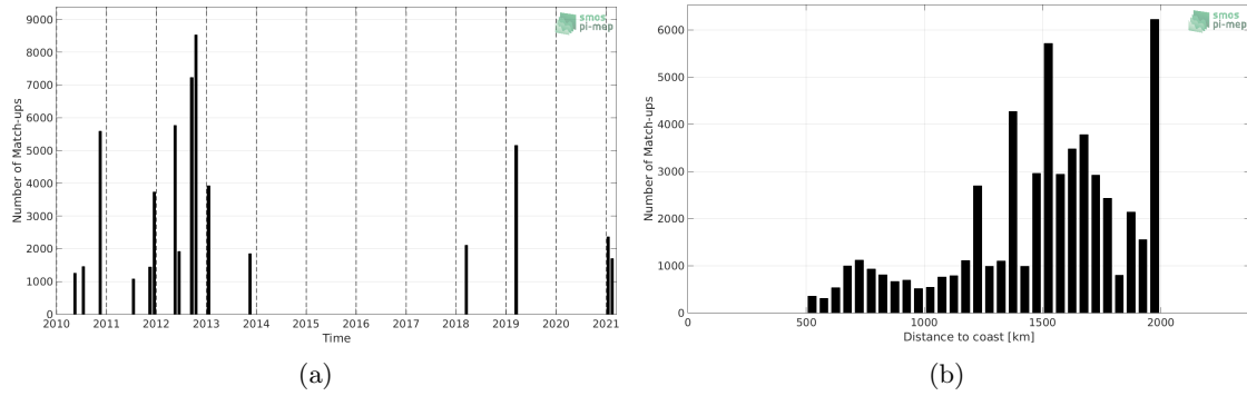
Figure 1: Number of match-ups between TSG (SAMOS) and SMOS SSS L2 v700 (ESA) SSS as a function of time (a) and as function of the distance to coast (b) over the SPURS 1 Pi-MEP region and for the full satellite product period.
