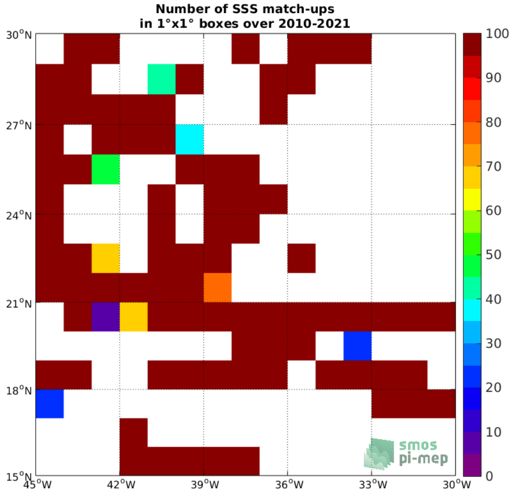
Figure 4: Number of SSS match-ups between TSG (SAMOS) SSS and the SMOS SSS L2 v700 (ESA) SSS product for the SPURS 1 Pi-MEP region over 1^\circ \times 1^\circ boxes and for the full satellite product period.
