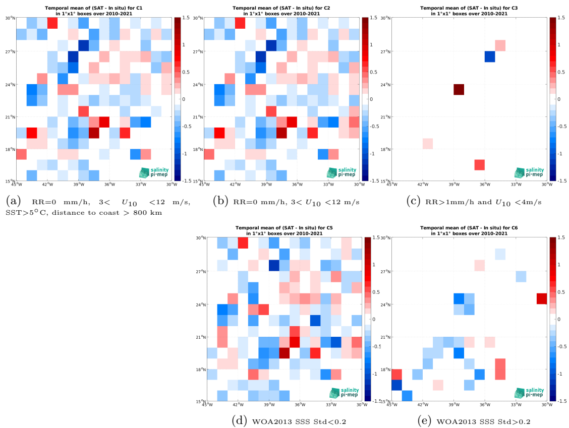
Figure 14: Temporal mean gridded over spatial boxes of size 1^\circ \times 1^\circ of \Delta SSS (SMOS SSS L2 v700 (ESA) - TSG (LEGOS-DM)) for 5 different subdatasets corresponding to:RR=0 mm/h, 3 < U_{10} < 12 m/s, SST >5^\circ C, distance to coast > 800 km (a), RR=0 mm/h, 3 < U_{10} < 12 m/s (b), RR >1 mm/h and U_{10} < 4 m/s (c), WOA2013 SSS Std <0.2 (d), WOA2013 SSS Std >0.2 (e).
