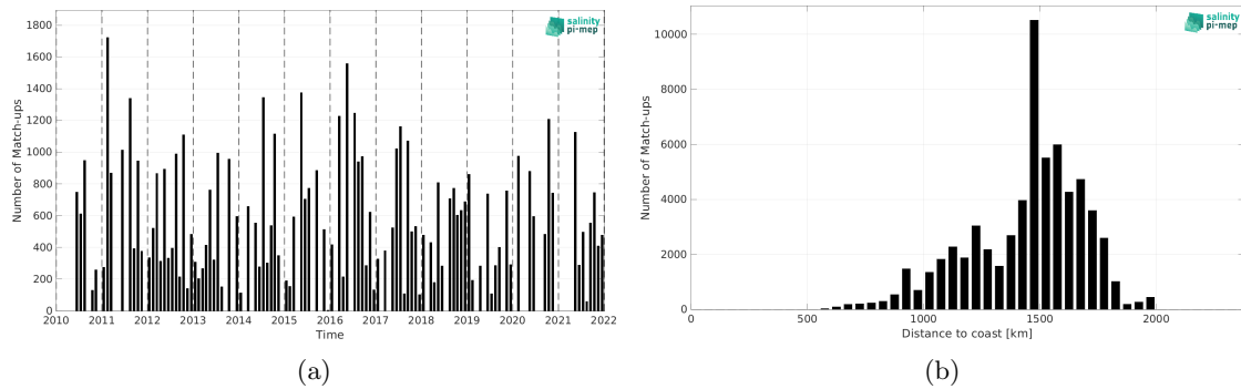
Figure 2: Number of match-ups between TSG (LEGOS-DM) and SMOS SSS L2 v700 (ESA) SSS as a function of time (a) and as function of the distance to coast (b) over the SPURS 1 Pi-MEP region and for the full satellite product period.
