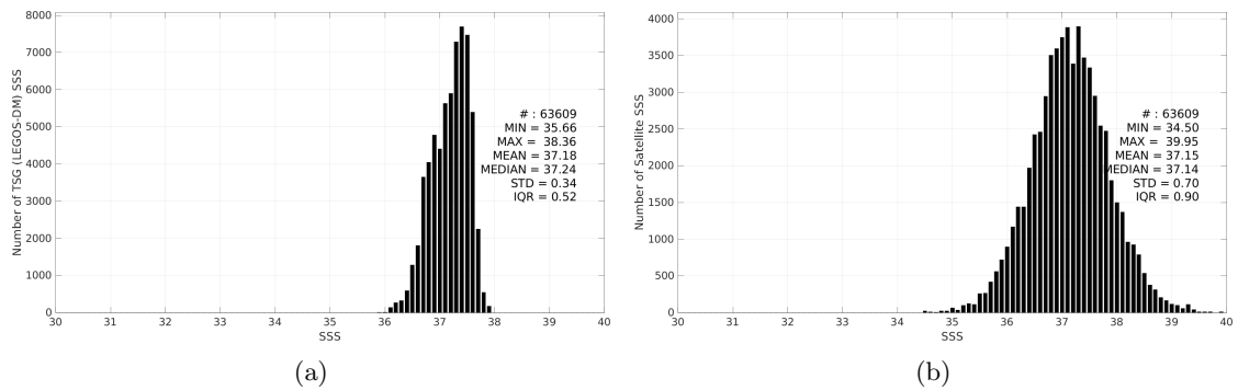
Figure 3: Histograms of SSS from TSG (LEGOS-DM) (a) and SMOS SSS L2 v700 (ESA) (b) considering all match-up pairs per bins of 0.1 over the SPURS 1 Pi-MEP region and for the full satellite product period.
