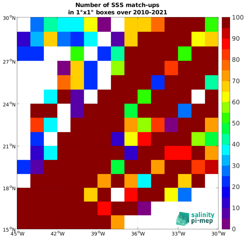
Figure 5: Number of SSS match-ups between TSG (LEGOS-DM) SSS and the SMOS SSS L2 v700 (ESA) SSS product for the SPURS 1 Pi-MEP region over 1°x1° boxes and for the full satellite product period.
