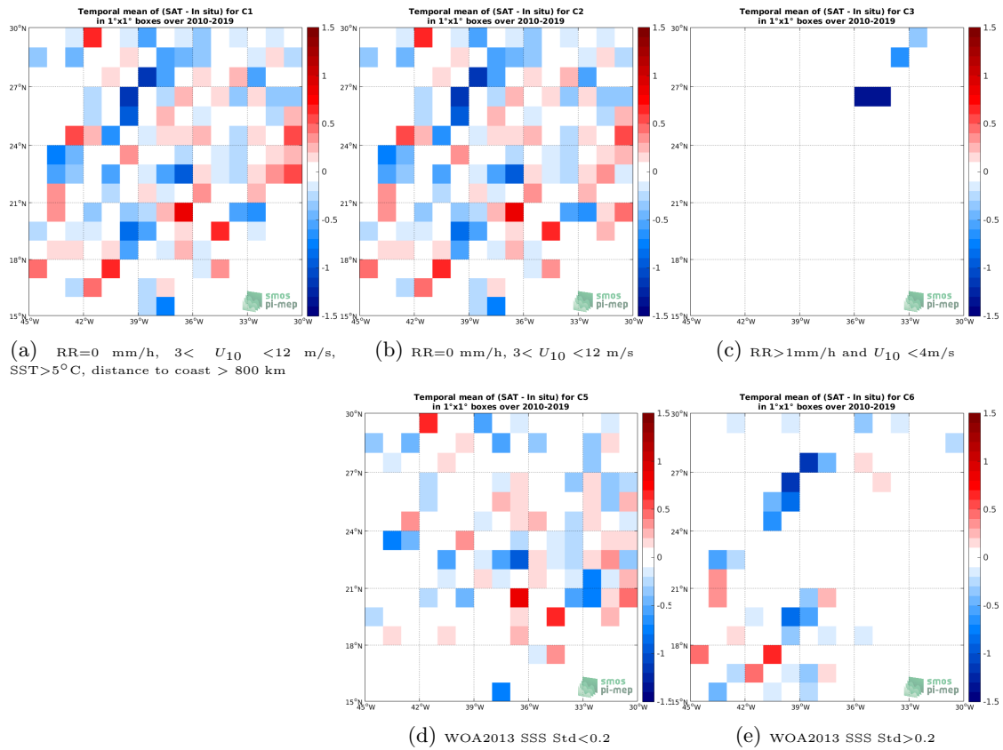
Figure 12: Temporal mean gridded over spatial boxes of size 1^\circ \times 1^\circ of \Delta SSS (SMOS SSS L2 v700 (ESA) - TSG (LEGOS-DM)) for 5 different subdatasets corresponding to: RR=0 mm/h, 3 < U_{10} < 12 m/s, SST > 5^\circ C , distance to coast > 800 km (a), RR=0 mm/h, 3 < U_{10} < 12 m/s (b), RR > 1 mm/h and U_{10} < 4 m/s (c), WOA2013 SSS Std < 0.2 (d), WOA2013 SSS Std > 0.2 (e).
