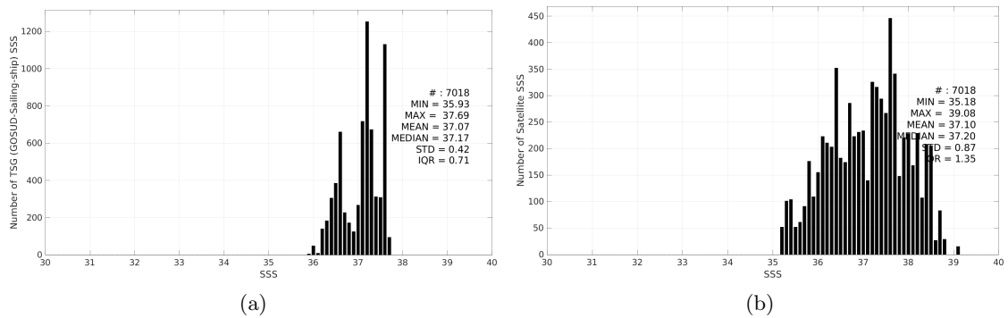
Figure 3: Histograms of SSS from TSG (GOSUD-Sailing-ship) (a) and SMOS SSS L2 v700 (ESA) (b) considering all match-up pairs per bins of 0.1 over the SPURS 1 Pi-MEP region and for the full satellite product period.
