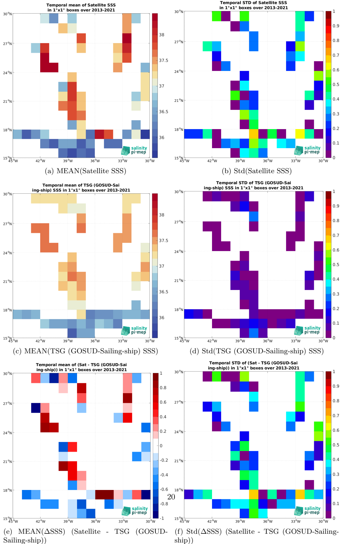
Figure 7: Temporal mean (left) and Std (right) of SSS from SMOS SSS L2 v700 (ESA) (top), TSG (GOSUD-Sailing-ship) (middle), and of \Delta SSS (Satellite - TSG (GOSUD-Sailing-ship)). Only match-up pairs are used to generate these maps.
