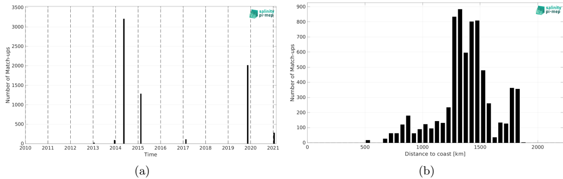
Figure 2: Number of match-ups between TSG (GOSUD-Sailing-ship) and SMOS SSS L2 v700 (ESA) SSS as a function of time (a) and as function of the distance to coast (b) over the SPURS 1 Pi-MEP region and for the full satellite product period.
