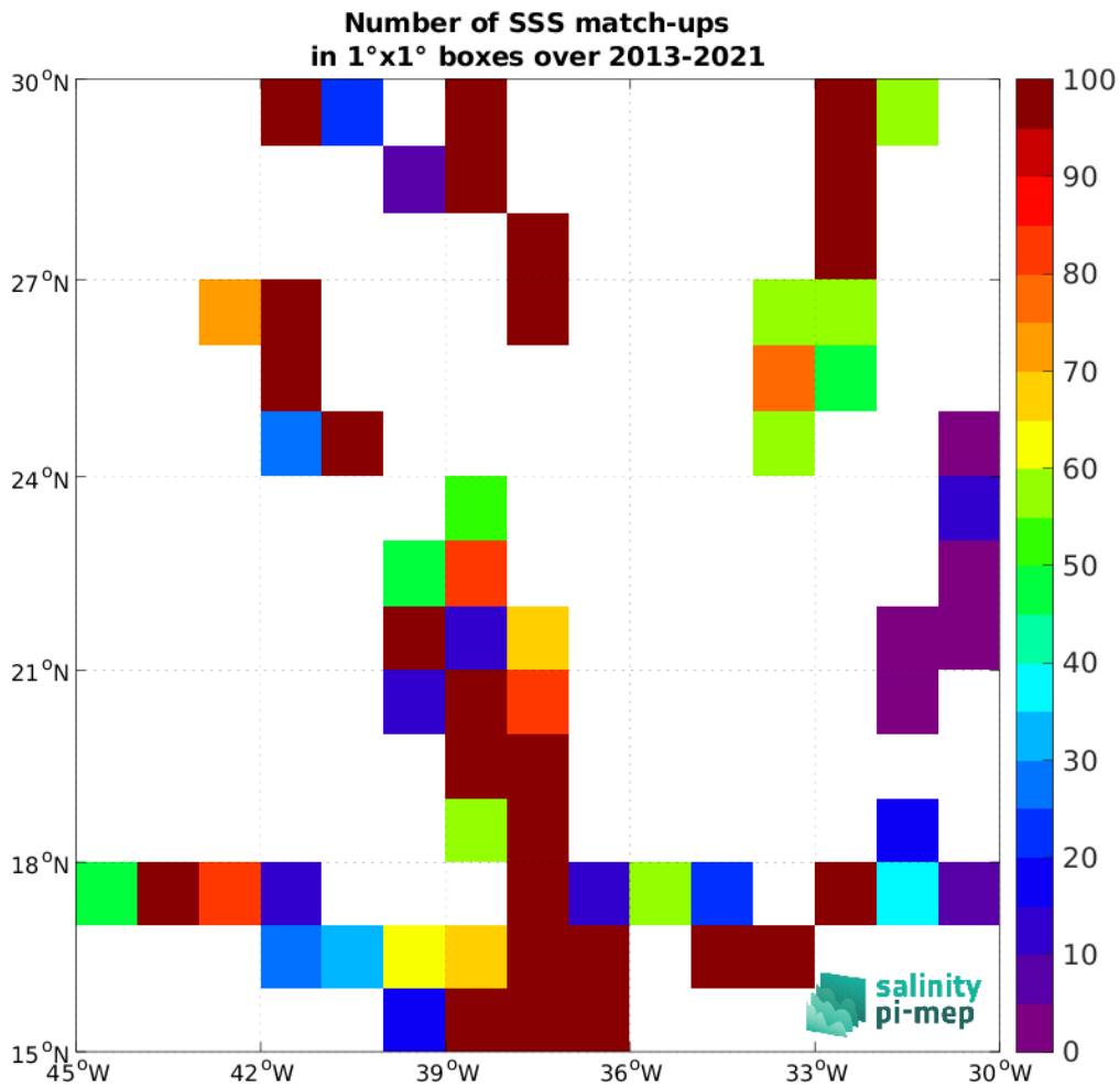
Figure 5: Number of SSS match-ups between TSG (GOSUD-Sailing-ship) SSS and the SMOS SSS L2 v700 (ESA) SSS product for the SPURS 1 Pi-MEP region over 1^\circ \times 1^\circ boxes and for the full satellite product period.
