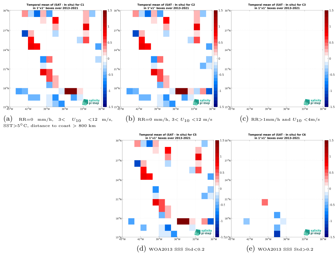
Figure 14: Temporal mean gridded over spatial boxes of size 1^\circ \times 1^\circ of \Delta SSS (SMOS SSS L2 v700 (ESA) - TSG (GOSUD-Sailing-ship)) for 5 different subdatasets corresponding to:RR=0 mm/h, 3 < U_{10} < 12 m/s, SST >5^\circ C, distance to coast > 800 km (a), RR=0 mm/h, 3 < U_{10} < 12 m/s (b), RR >1 mm/h and U_{10} < 4 m/s (c), WOA2013 SSS Std <0.2 (d), WOA2013 SSS Std >0.2 (e).
