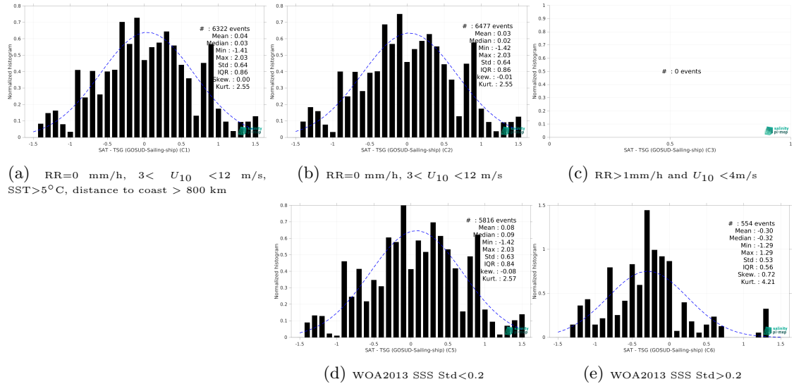
Figure 15: Normalized histogram of \Delta SSS (SMOS SSS L2 v700 (ESA) - TSG (GOSUD-Sailing-ship)) for 5 different subdatasets corresponding to: RR=0 mm/h, 3 < U_{10} < 12 m/s, SST > 5°C, distance to coast > 800 km (a), RR=0 mm/h, 3 < U_{10} < 12 m/s (b), RR > 1mm/h and U_{10} < 4 m/s (c), WOA2013 SSS Std < 0.2 (d), WOA2013 SSS Std > 0.2 (e).
