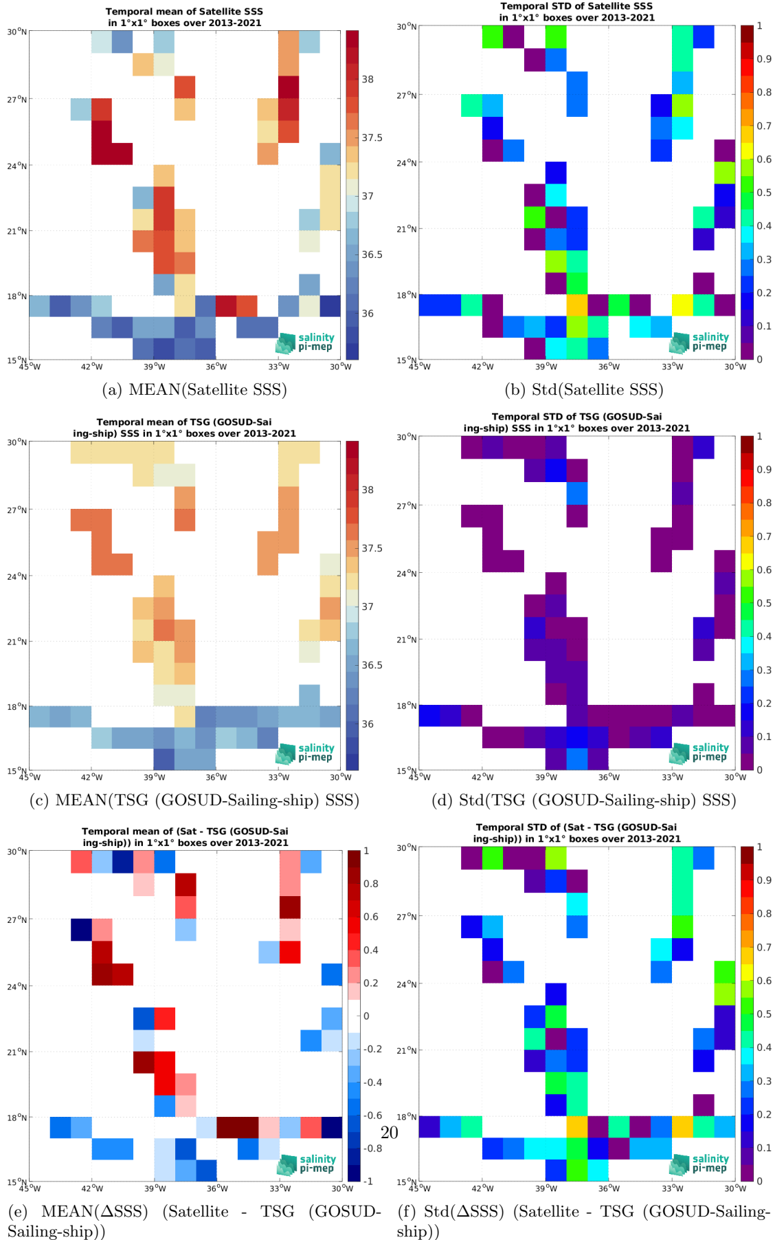
Figure 6: Temporal mean (left) and Std (right) of SSS from SMOS SSS L2 v700 (ESA) (top), TSG (GOSUD-Sailing-ship) (middle), and of \Delta SSS (Satellite - TSG (GOSUD-Sailing-ship)). Only match-up pairs are used to generate these maps.
