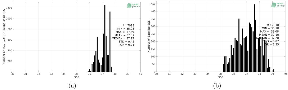
Figure 2: Histograms of SSS from TSG (GOSUD-Sailing-ship) (a) and SMOS SSS L2 v700 (ESA) (b) considering all match-up pairs per bins of 0.1 over the SPURS 1 Pi-MEP region and for the full satellite product period.
