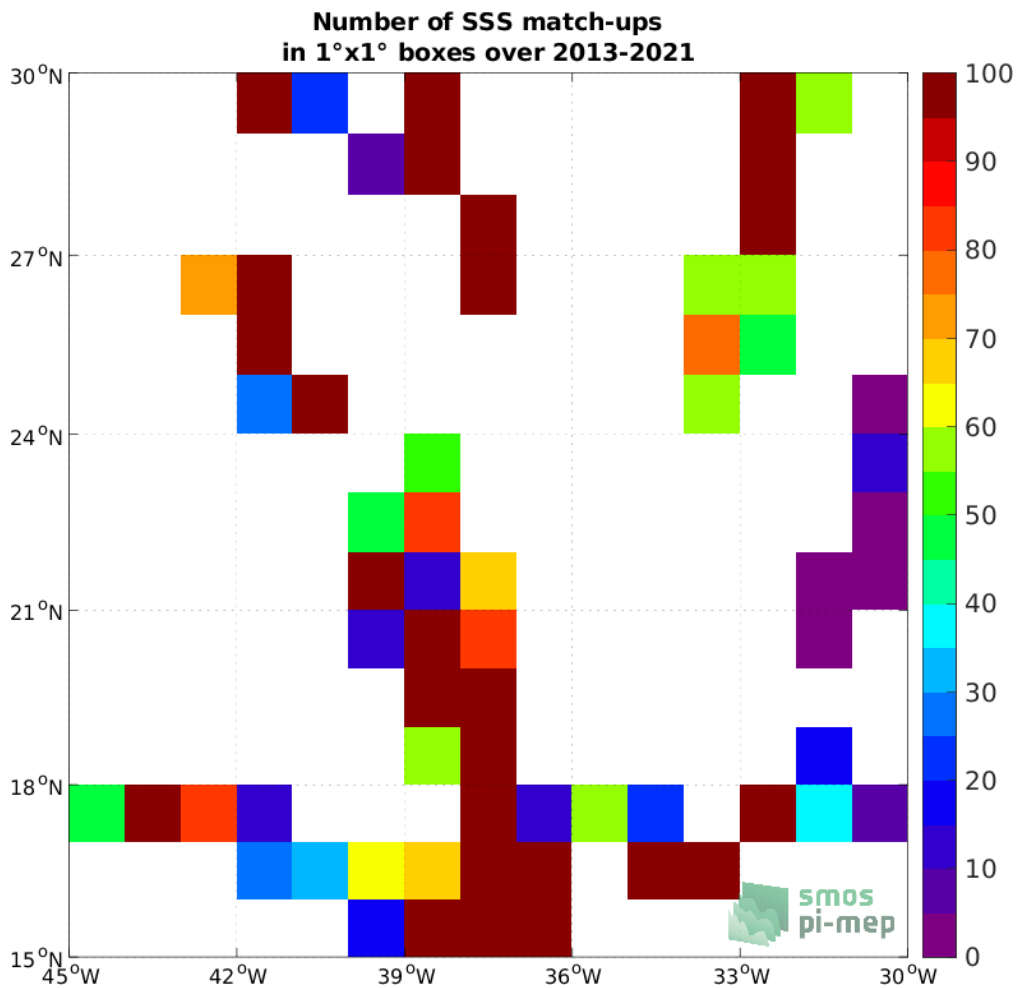
Figure 4: Number of SSS match-ups between TSG (GOSUD-Sailing-ship) SSS and the SMOS SSS L2 v700 (ESA) SSS product for the SPURS 1 Pi-MEP region over 1°×1° boxes and for the full satellite product period.
