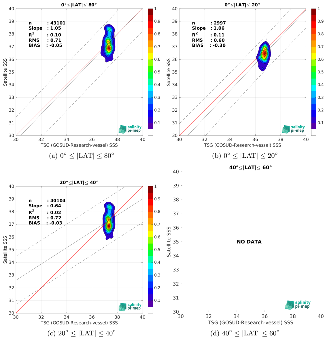
Figure 10: Contour maps of the concentration of SMOS SSS L2 v700 (ESA) SSS (y-axis) versus TSG (GOSUD-Research-vessel) SSS (x-axis) at match-up pairs for different latitude bands. For each plot, the red line shows x=y . The black thin and dashed lines indicate a linear fit through the data cloud and the \pm 95\% confidence levels, respectively. The number match-up pairs n , the slope and R^2 coefficient of the linear fit, the root mean square (RMS) and the mean bias between satellite and in situ data are indicated for each latitude band in each plots.
