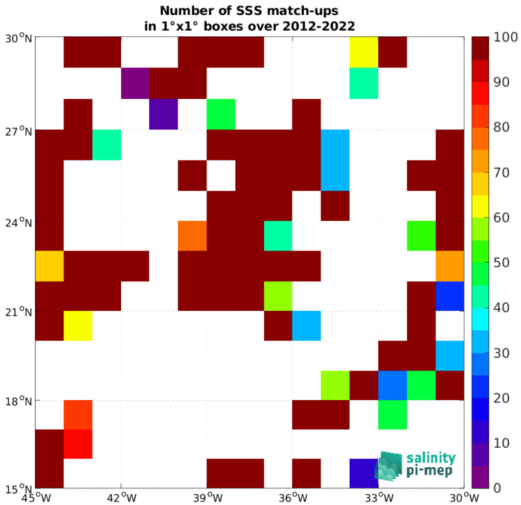
Figure 5: Number of SSS match-ups between TSG (GOSUD-Research-vessel) SSS and the SMOS SSS L2 v700 (ESA) SSS product for the SPURS 1 Pi-MEP region over 1^\circ \times 1^\circ boxes and for the full satellite product period.
