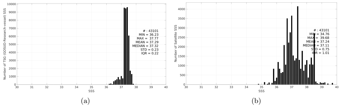
Figure 3: Histograms of SSS from TSG (GOSUD-Research-vessel) (a) and SMOS SSS L2 v700 (ESA) (b) considering all match-up pairs per bins of 0.1 over the SPURS 1 Pi-MEP region and for the full satellite product period.
