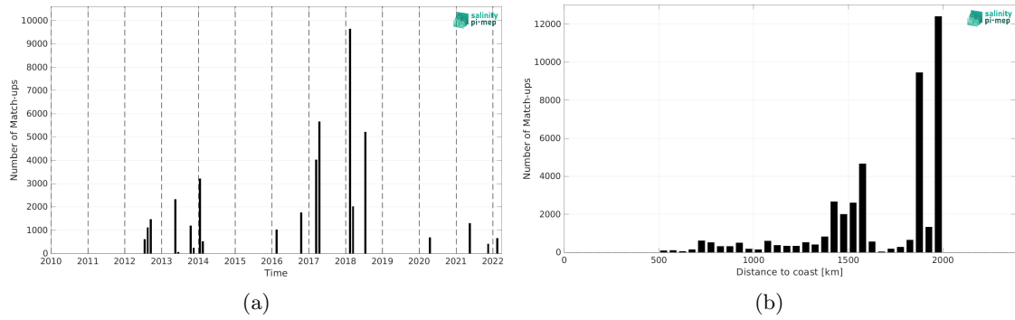
Figure 2: Number of match-ups between TSG (GOSUD-Research-vessel) and SMOS SSS L2 v700 (ESA) SSS as a function of time (a) and as function of the distance to coast (b) over the SPURS 1 Pi-MEP region and for the full satellite product period.
