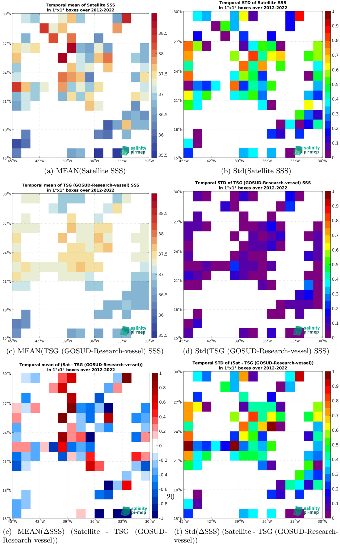
Figure 7: Temporal mean (left) and Std (right) of SSS from SMOS SSS L2 v700 (ESA) (top), TSG (GOSUD-Research-vessel) (middle), and of \Delta SSS (Satellite - TSG (GOSUD-Research-vessel)). Only match-up pairs are used to generate these maps.
