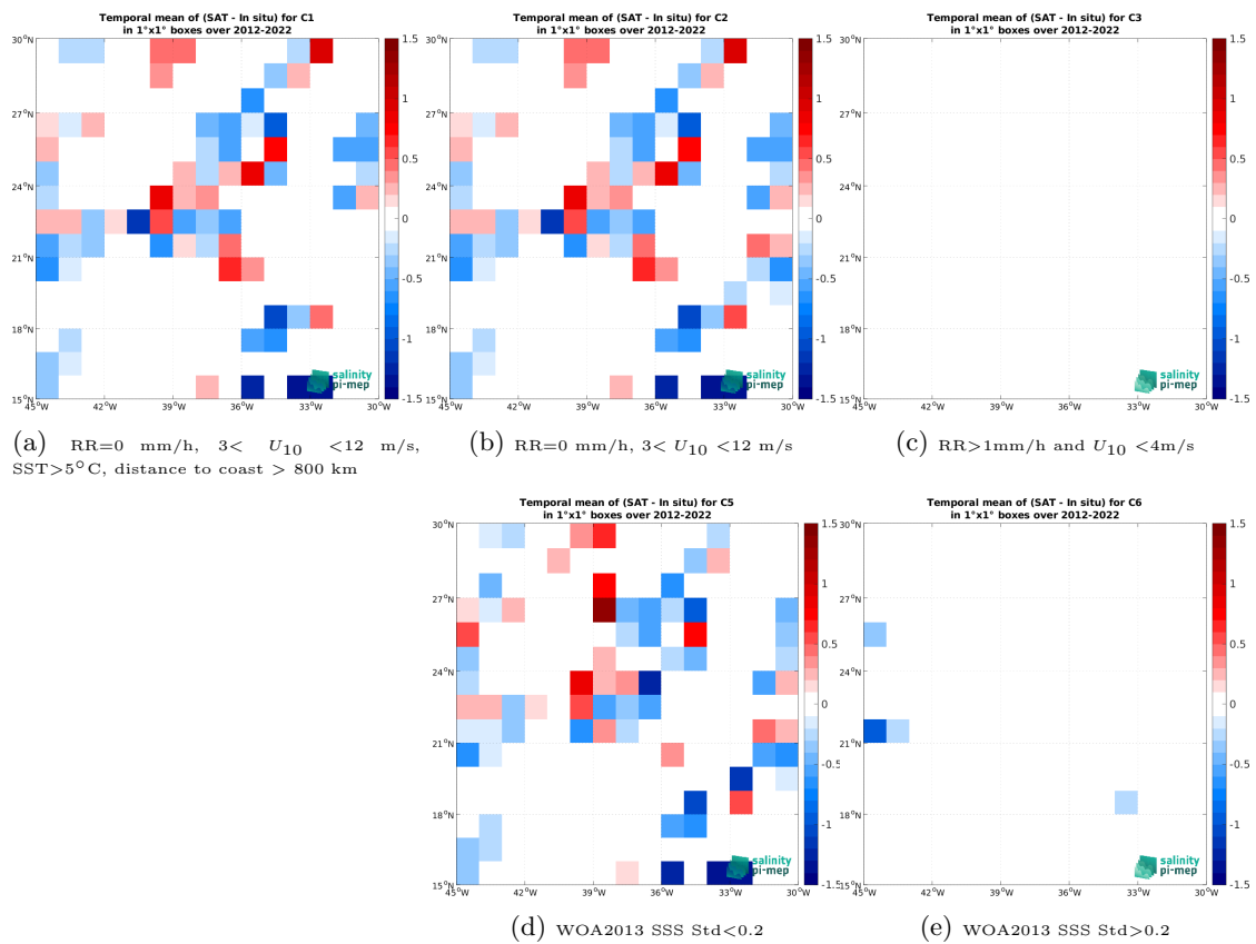
Figure 14: Temporal mean gridded over spatial boxes of size 1^\circ \times 1^\circ of \Delta SSS (SMOS SSS L2 v700 (ESA) - TSG (GOSUD-Research-vessel)) for 5 different subdatasets corresponding to: RR=0 mm/h, 3 < U_{10} < 12 m/s, SST > 5^\circ C , distance to coast > 800 km (a), RR=0 mm/h, 3 < U_{10} < 12 m/s (b), RR > 1 mm/h and U_{10} < 4 m/s (c), WOA2013 SSS Std < 0.2 (d), WOA2013 SSS Std > 0.2 (e).
