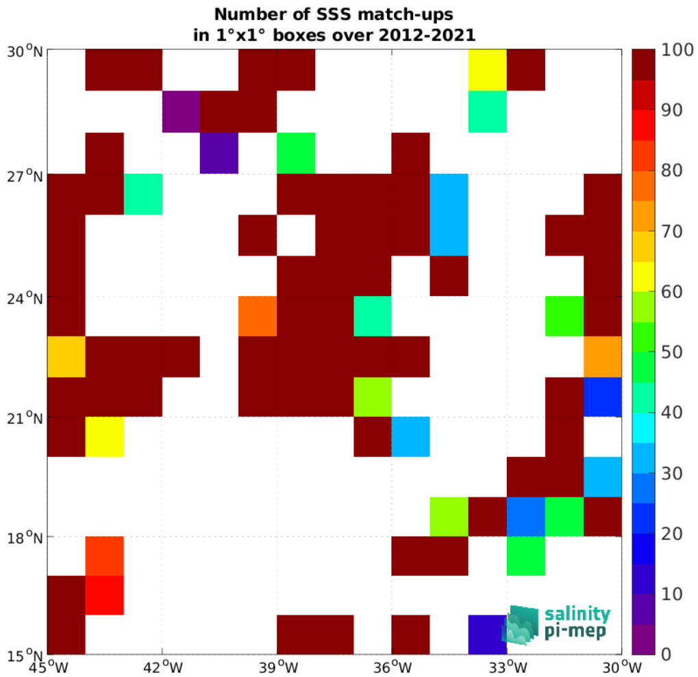
Figure 5: Number of SSS match-ups between TSG (GOSUD-Research-vessel) SSS and the SMOS SSS L2 v700 (ESA) SSS product for the SPURS 1 Pi-MEP region over 1°x1° boxes and for the full satellite product period.
